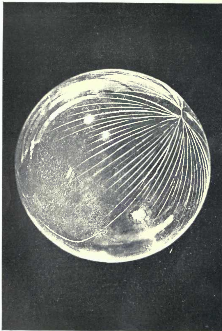
PLATE XXIII. — Glass Globe, cracked by internal pressure, illustrating the cause of the bright streaks radiating from Tycho.
