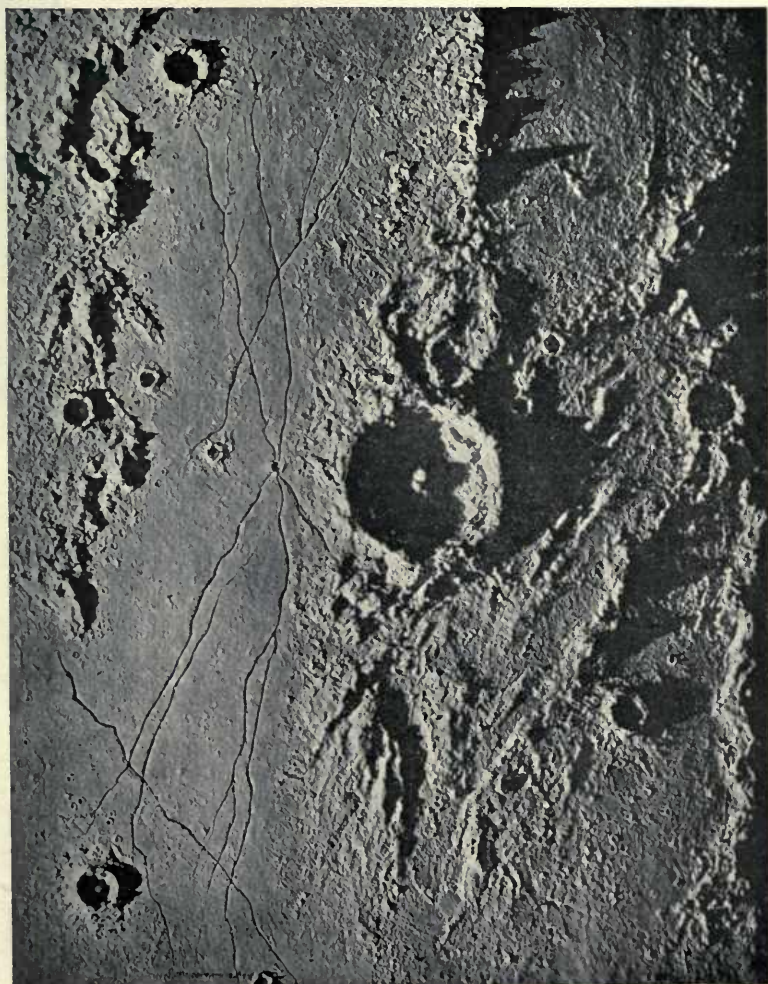
PLATE IX.—Triesnecker.
