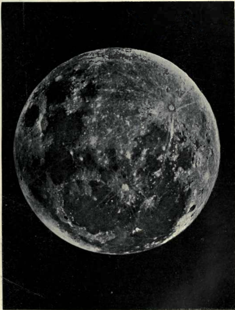
PLATE IV.—Full Moon.
