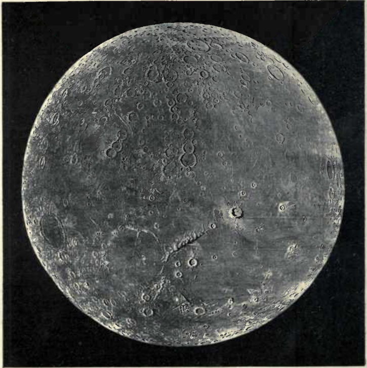
PLATE V.—Picture Map of the Moon.
