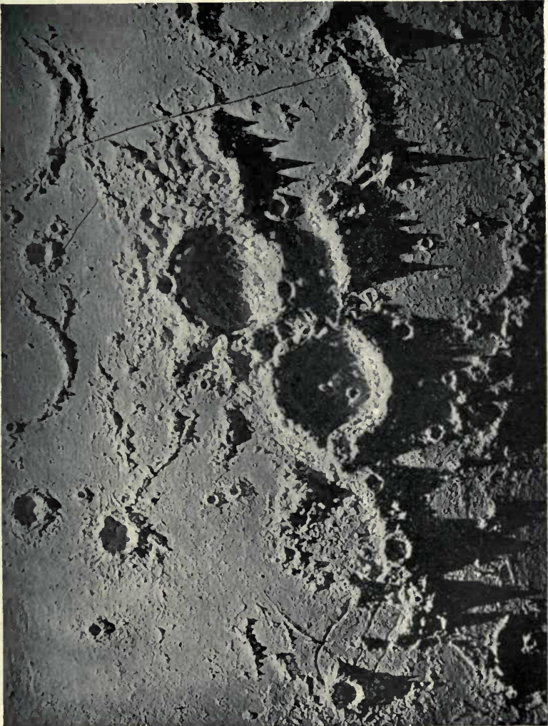
PLATE XX.—Mercator and Campanus.
