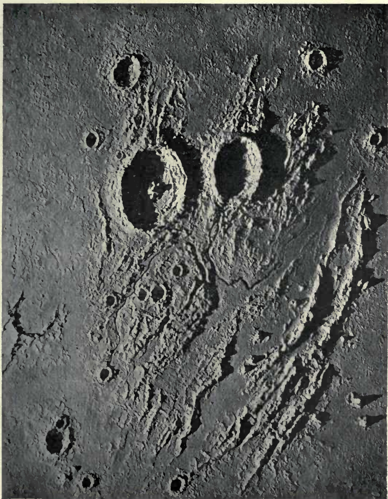
PLATE XIV.—Aristarchus and Herodotus.
