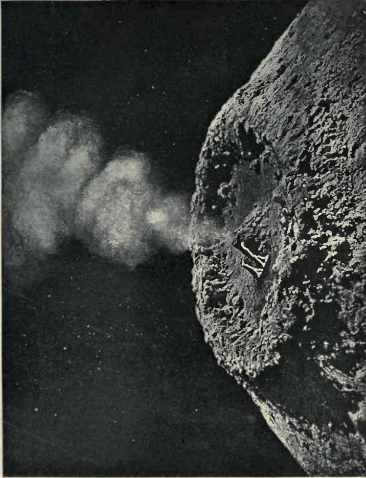
PLATE I.—The Crater of Vesuvius in 1864.
