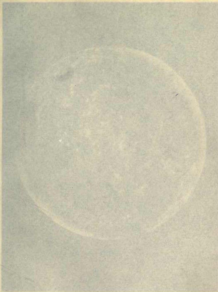
PLATE XXIV.—Full Moon, exhibiting the bright streaks radiating from Tychon.
