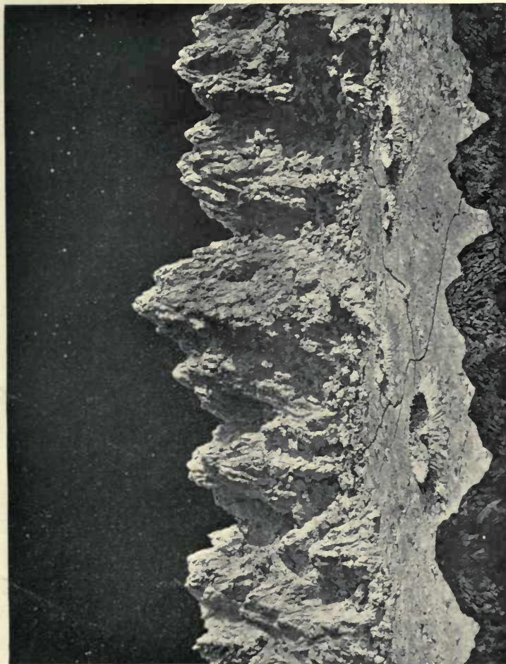
PLATE XXV.—Group of Lunar Mountains (Ideal Lunar Landscape).
