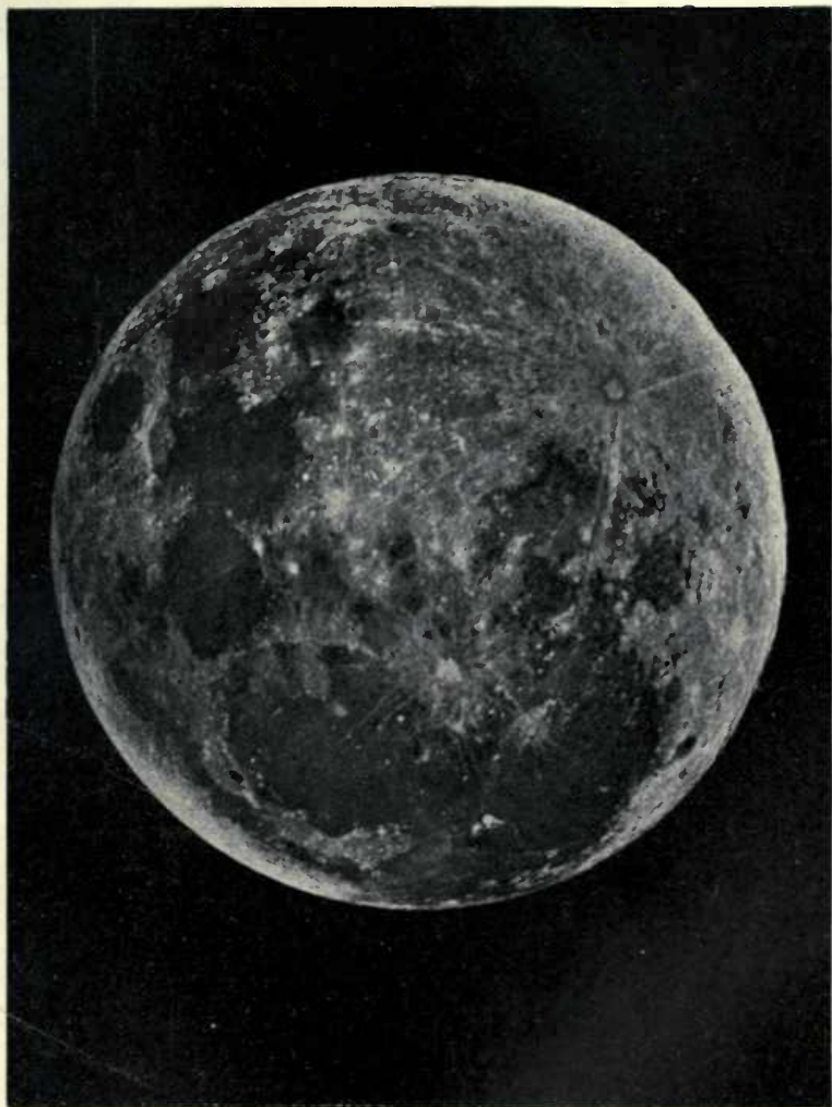
PLATE XXIV.—Full Moon, exhibiting the bright streaks radiating from Tycho.
