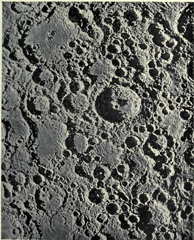
PLATE XIII.—Tycho and its surroundings.
