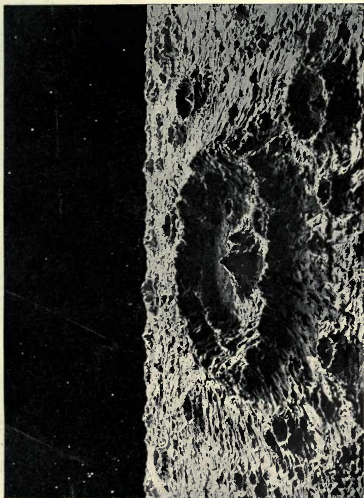
PLATE XVII.—Normal Lunar Crater.
