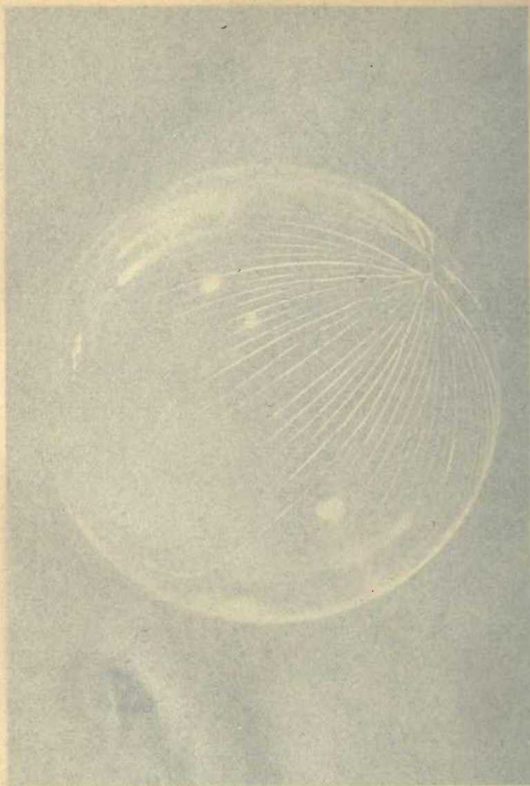
PLATE XXIII.—Glass Globe, expanded by internal pressure, illustrating the course of the bright streaks radiating from Tycho.
