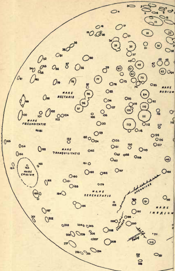
SKELETON MAP OF THE MOON TO ACCOMPANY PICTURE MAP (PI)
