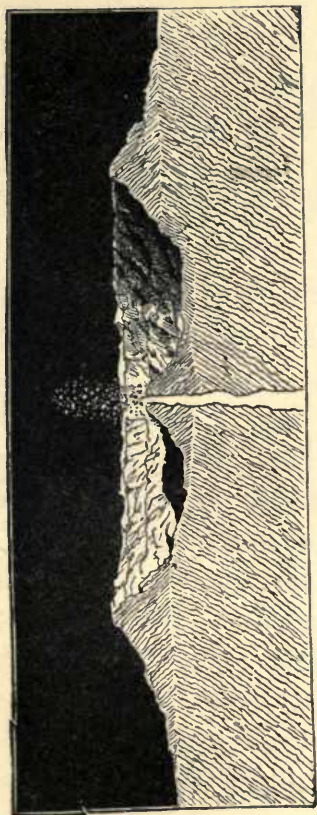
The formation of the Central Cone. Final action of a Lunar Volcano.
