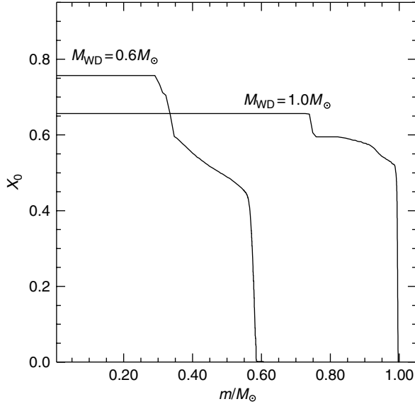
Figure 7.9 Oxygen profile within the core of two WD models
