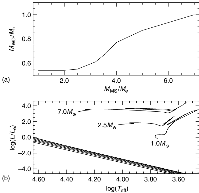
Figure 7.5 (a) shows an approximate relationship between the initial stellar mass ( M_{MS} ) and the final WD mass ( M_{WD} ) for a range of low- and intermediate-mass stars. (b) displays the HRD location of WD evolutionary tracks for different values of M_{WD} (between 0.54 and 1 M_{\odot} ) compared with previous evolutionary phases
