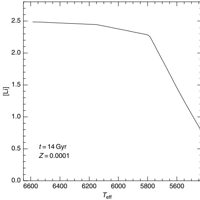
Figure 9.20 Trend of [Li] with T_{\text{eff}} along the MS of a theoretical isochrone with Z = 0.0001 and t = 14 Gyr, for an initial lithium abundance [Li] = 2.5
