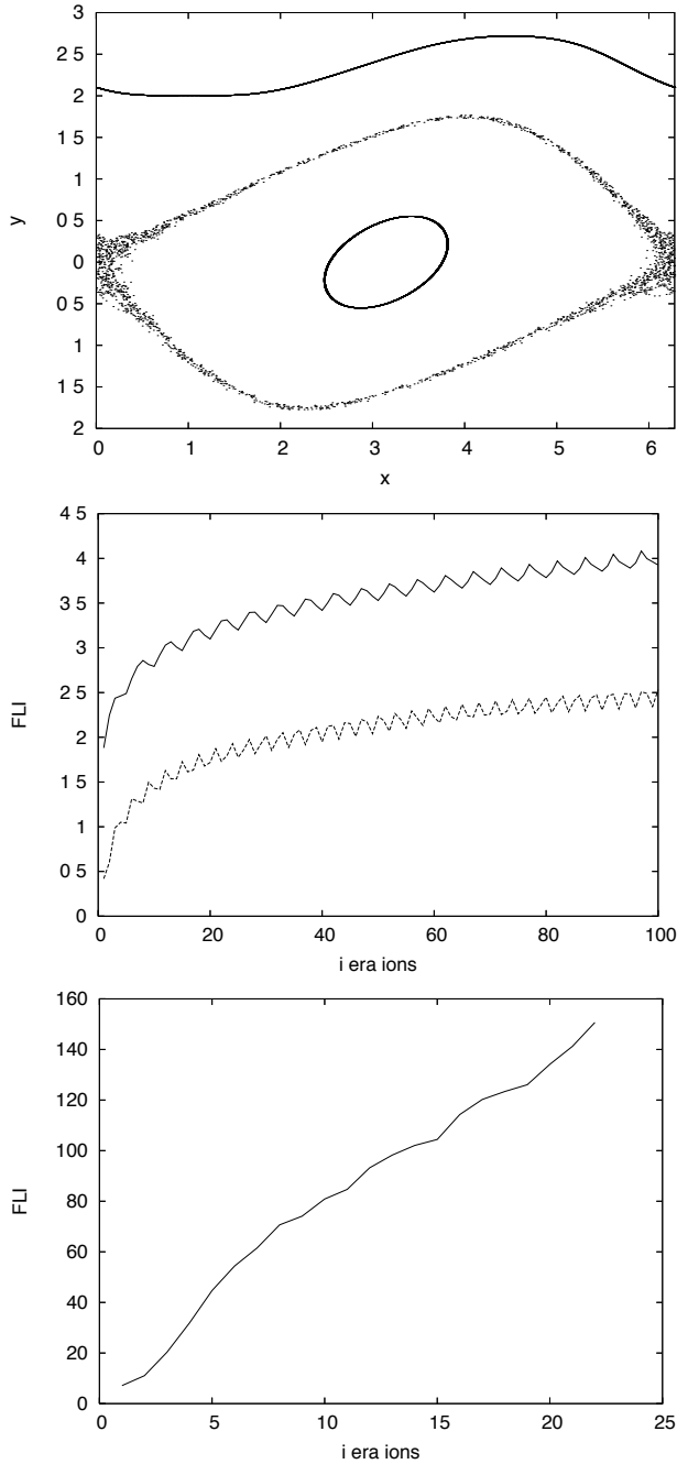
Fig. 2.8. The computation of the FLI for the classical standard map. The upper panel shows a librational island, a chaotic separatrix and an invariant curve. The middle panel shows the FLIs for the librational island (bottom line) and for the invariant curve (upper line). The bottom panel shows the FLI for the chaotic region.
