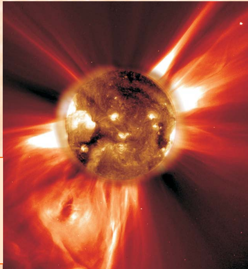
■ Above: The intense burst from a solar flare (top right) is captured by the SOHO EIT instrument during the 24–26 November 2000 series of six major solar flares and associated "halo" coronal mass ejections (CMEs). Image courtesy SOHO-EIT Consortium, ESA, NASA.
