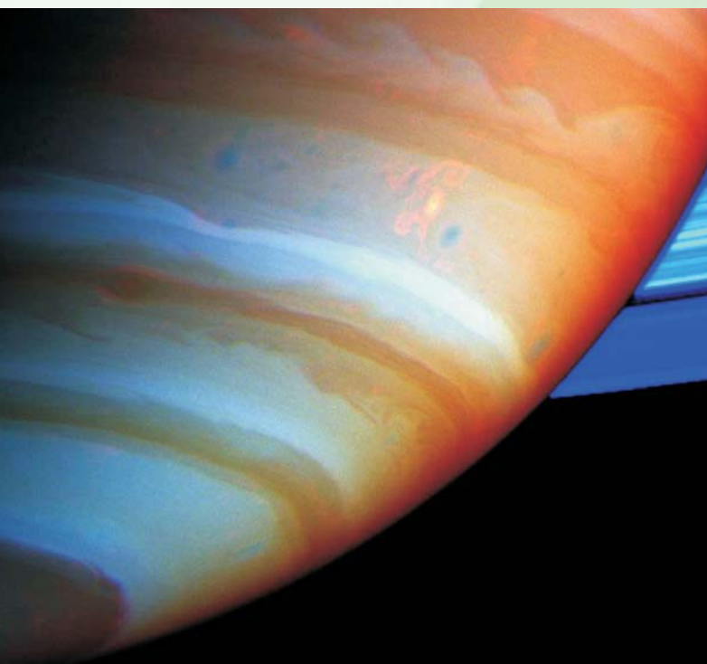
■ Left: A false colour composite of Saturn's southern atmosphere made from Cassini images taken in near infrared light through filters that sense different amounts of methane gas. Clouds that are deep in the atmosphere are red, while grey indicates high clouds, and brown indicates clouds at intermediate altitudes. The bright feature just above and to the right of centre is a complex convective storm called the 'Dragon Storm'. It lies in a region referred to as 'Storm Alley' because of the high level of storm activity observed there. The Dragon Storm was a powerful source of radio emissions during July and September of 2004. Scientists have concluded that the Dragon Storm is a giant thunderstorm whose precipitation generates electricity as it does on Earth. Image courtesy NASA/JPL/Space Science Institute.
