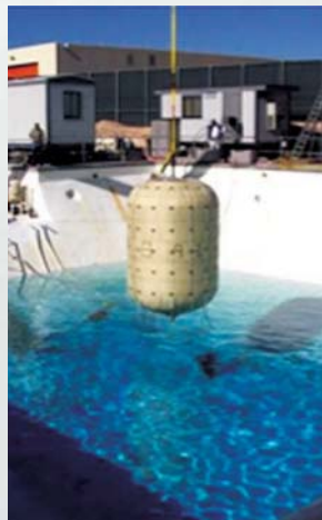
Below: A 2.24-metre diameter demonstration restraint layer being prepared for hydrostatic testing (top) at Johnson Space Center in November 2005. The fact that the restraint layer failed only at a pressure of 197 psi (13.85 kg/cm 2 ) demonstrated a factor of safety exceeding 4.0 (bottom). Images courtesy NASA/Chris Johnson/Gary Spexarth.
