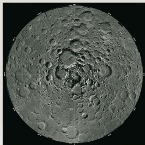
■ Below: The polar regions of the Moon: north to the left and south to the right. The images were obtained by the Clementine spacecraft. The colour-coded overlays show the epithermal neutron emission measured by the Lunar Prospector spacecraft, with dark blue and purple indicating low counting rates consistent with hydrogen-rich deposits intermixed with desiccated regolith. Clementine images courtesy Naval Research Laboratory, with post-processing by the US Geological Survey. Lunar Prospector images courtesy NASA Ames Research Center, and William Feldman of the Los Alamos National Laboratory.
