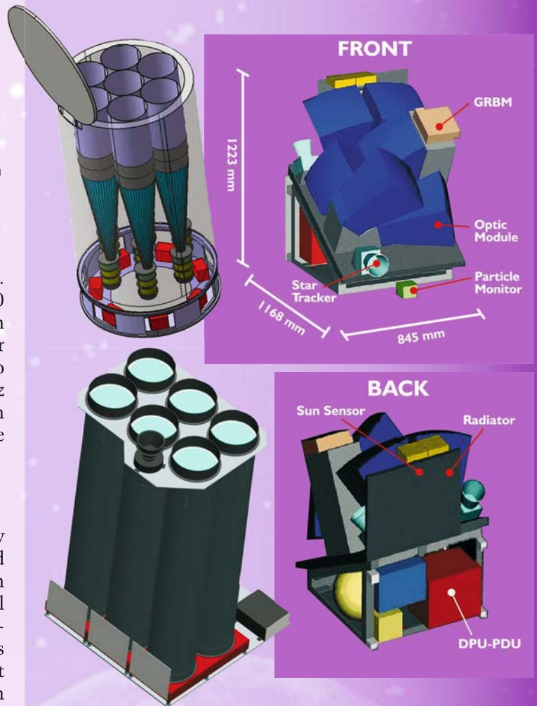
■ Above: Artist's schematics showing the three main instruments to be carried by the Spektr RG space observatory: eROSITA with its cluster of seven Wolter-I telescope modules (top left), LOBSTER, a wide-field X-ray monitor (right), and ART-XC, an X-ray concentrator based on Kumakhov optics (bottom left). Images courtesy IKI, Institute for Space Research, Moscow.
