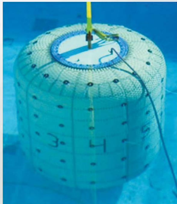
Below: A 2.24-metre diameter demonstration restraint layer being prepared for hydrostatic testing (top) at Johnson Space Center in November 2005. The fact that the restraint layer failed only at a pressure of 197 psi (13.85 kg/cm 2 ) demonstrated a factor of safety exceeding 4.0 (bottom). Images courtesy NASA/Chris Johnson/Gary Spexarth.
