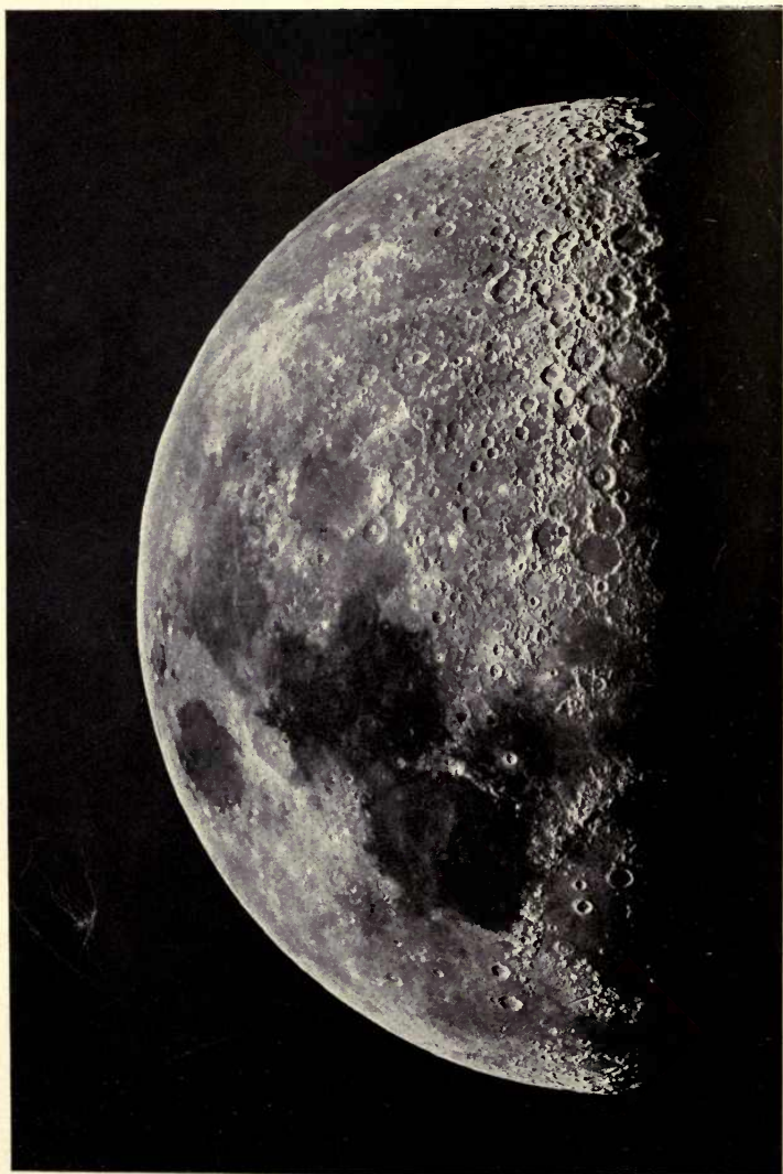
The Moon. First Quarter.
