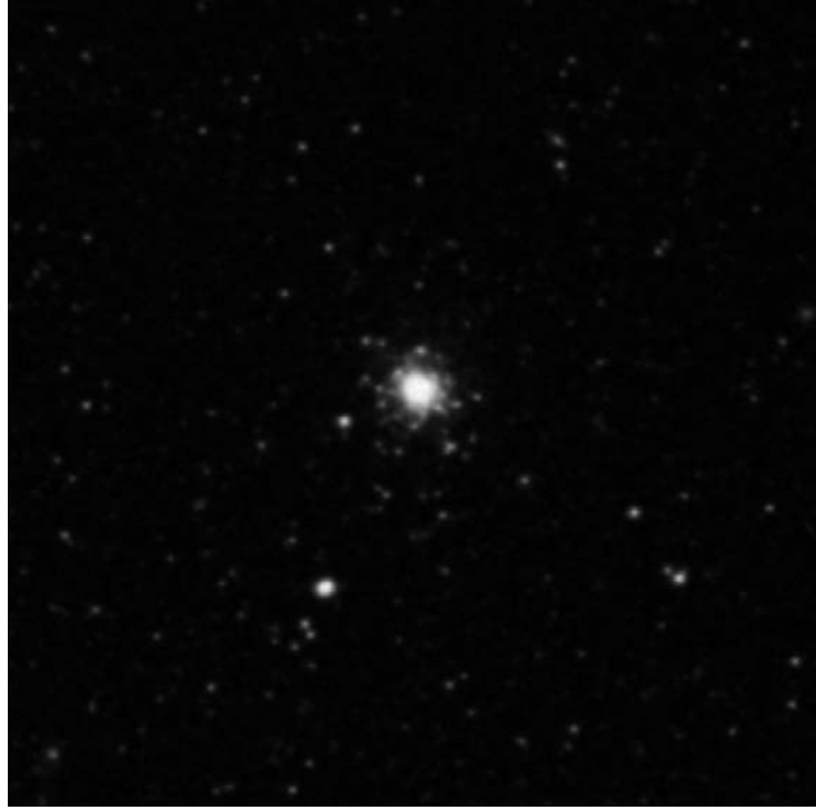
Fig. 8.2. NGC 1049, a bright globular cluster in the Fornax dwarf galaxy
