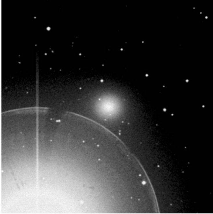
Fig. 10.1. The peculiar S0 galaxy NGC 404 near Mirach ( \beta And)
