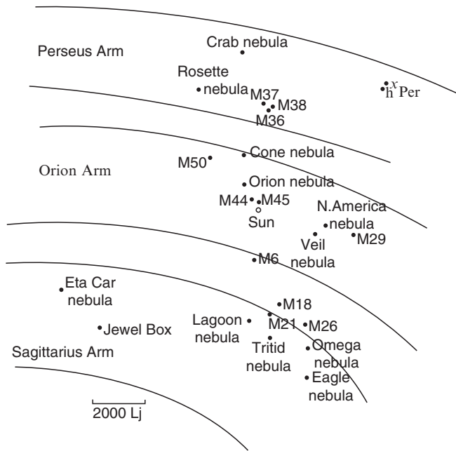
Fig. 1.8. Local and neighboring spiral arms with a sample of embedded nebulae and clusters
