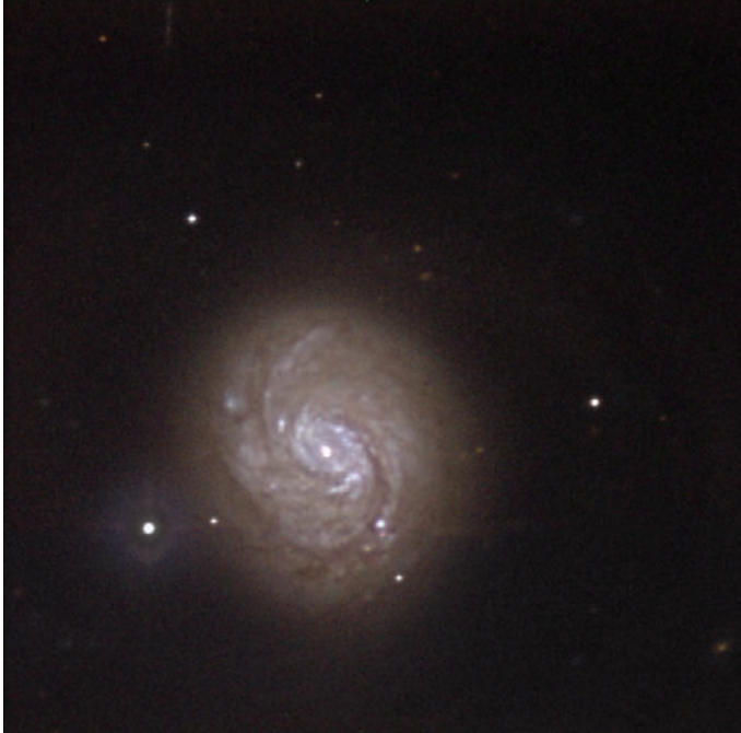
Fig. 1.27. M 77 in Cetus, a prominent Seyfert galaxy
