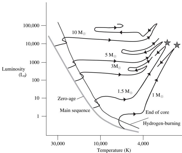
Figure 3.14. Post-main-sequence evolutionary track for several stars of different masses.
