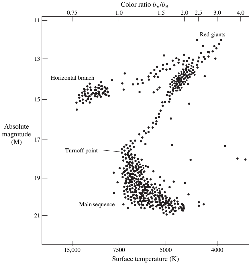
Figure 3.15. Color-magnitude diagram for the globular cluster M3.
