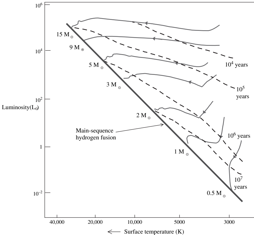
Figure 3.1. Pre-main-sequence lifetracks.
