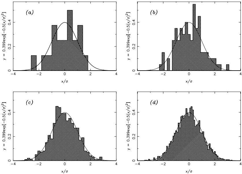
Fig. 3.1. X_i drawn at random from a Gaussian distribution of \sigma = 1 : (a) 20 values, (b) 100 values, (c) 500 values, (d) 2500 values. The average values of x_i are 0.003, 0.080, -0.032 and -0.005 ; the median values 0.121, 0.058, -0.069 and -0.003 ; and the rms values 0.968, 1.017, 0.986, and 1.001. Solid curves represent Gaussians of unit area and standard deviation.
