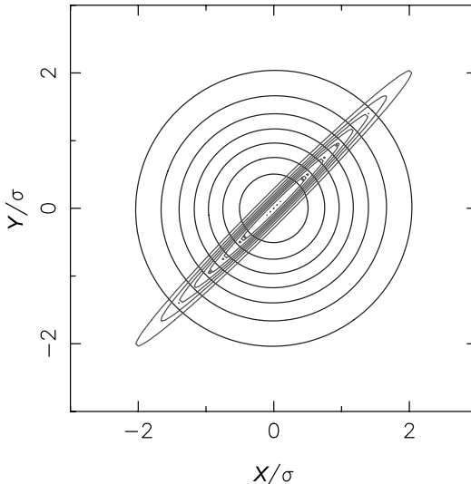
Fig. 4.4. Linear contours of the bivariate Gaussian probability distribution; the near-circular contours represent \rho = 0.01 , a bivariate distribution with little connection between x and y , while the highly elliptical contours represent \rho = 0.99 , indicative of a strong correlation between x and y . Negative values of \rho reverse the tilt, and indicate what is loosely referred to as anticorrelation.
