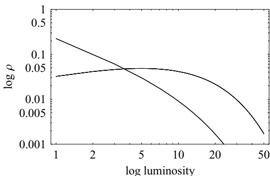
Fig. 7.3. The luminosity function \rho (steep curve) and the (flat-space) luminosity distribution are plotted for the Schechter form of the luminosity function.
