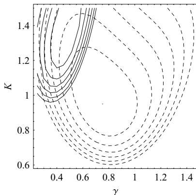
Fig. 6.5. The log likelihoods for the two models; the black contours are for model A and the dashed contours are for model B.
