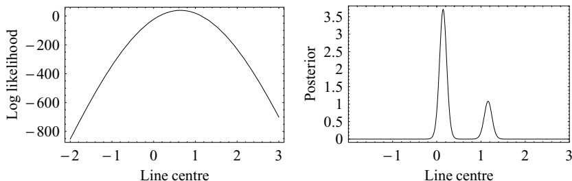
Fig. 6.12. The log likelihood function for the combined, unweighted data (left) and the posterior distribution for the line centre, after marginalizing out the weights (right).
