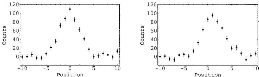
Fig. 6.11. The two synthetic spectra which are our input data.
