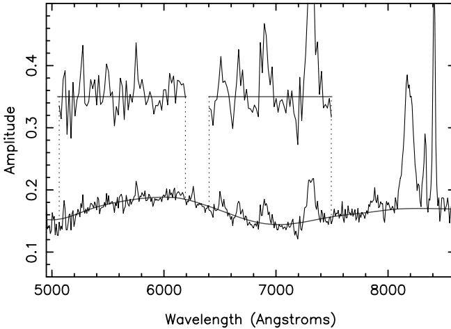
Fig. 5.5. A spectrum of the quasar 3C207, taken with the 4.2-m William Herschel Telescope. The solid curve is a baseline fitted by a Fourier minimum-component technique. The regions considered for the runs test are shown in the separated sections, each with the baseline subtracted and magnified by a factor of 3.
