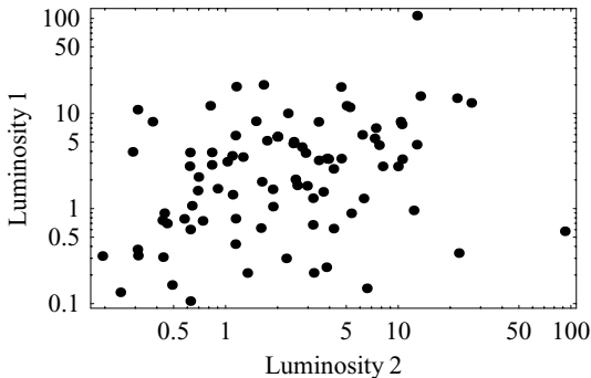
Fig. 7.16. The apparent correlation between two new luminosities in the doubly resurveyed sample.
