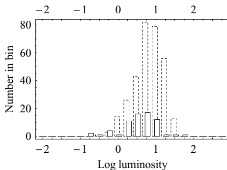
Fig. 7.12. The luminosity distribution, and upper limits, for the field-galaxy simulation; there are 67 detections and 317 upper limits. The bins (dashed) for the upper limits are slightly displaced for clarity.
