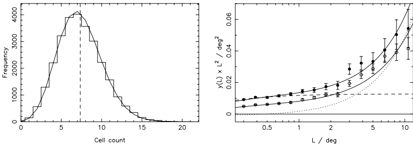
Fig. 9.4. Left: counts of NVSS radio sources with S_{1.4\text{GHz}} > 20 mJy in cells of diameter 1^\circ . Vertical dashed line – expected mean count derived from the source surface density; solid curve – the corresponding Poisson distribution. Right: The variance statistic y(L) is plotted for thresholds 20 mJy (solid circles) and 10 mJy (open circles), with predictions of the double power-law w(\theta) models at 20 mJy and 10 mJy (solid lines). The dashed and dotted lines show the separate contributions to y(L) at 20 mJy of the steep (multiple-component) w(\theta) and the shallow (cosmological) w(\theta) .
