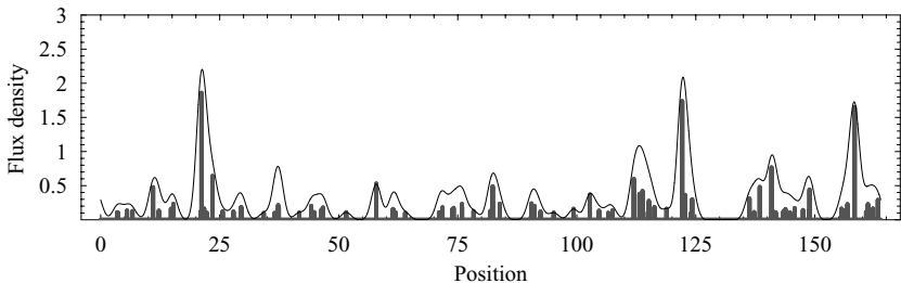
Fig. 7.17. A confusion simulation at a level of one source per beam area. The input sources are shown as vertical lines, with the solid line representing the response when observed (convolved) with a Gaussian beam.
