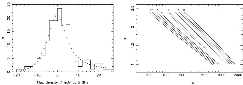
Fig. 6.6. An example of model fitting via minimum \chi^2 . The object of the experiment was to estimate the surface-density count [ N(S) relation; see Section 6.1, Fig. 6.1] of faint extragalactic sources at 5 GHz, assuming a power-law N(> S) = KS^{-(\gamma-1)} , \gamma and K to be determined from the distribution of background deflections, the so-called P(D) method, Section 7.6. The histogram of measured deflections is shown left, together with the curve representing the optimum model from minimizing \chi^2 . Contours of \chi^2 in the \gamma - K plane are shown right, with \chi^2 indicated for every second contour.
