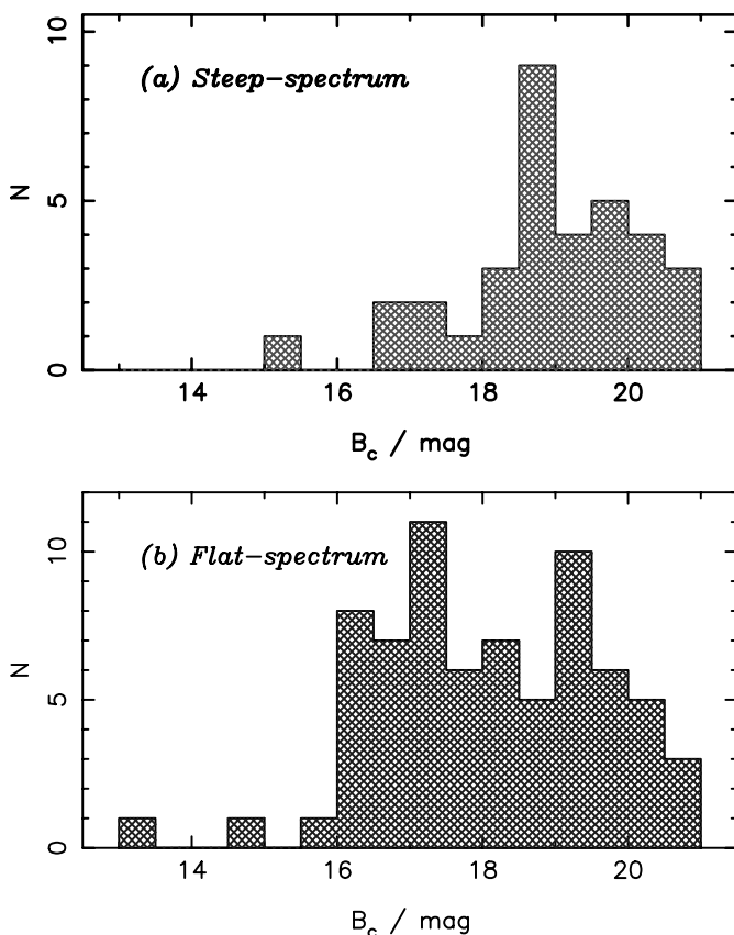
Fig. 5.6. Magnitude histograms for a complete sample of quasars from the Parkes 2.7-GHz survey, distinguished by radio spectrum. H_0 , that the magnitude distributions are identical, is rejected using the Mann–Whitney–Wilcoxon U test at the 0.004 level of significance.
