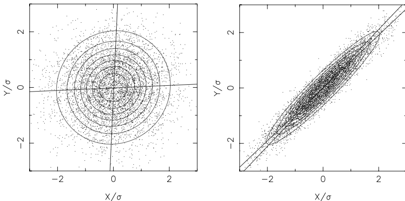
Fig. 6.2. Linear contours of the bivariate Gaussian probability distribution. Left: \rho = 0.05 , a bivariate distribution with weak connection between x and y ; right: \rho = 0.95 , indicative of a strong connection between x and y . In each case 5000 (x, y) pairs have been plotted, selected at random from the appropriate distribution as described in Section 6.5. Two lines are shown as fits for each distribution, the OLS( X/Y ) and the OLS( Y/X ).
