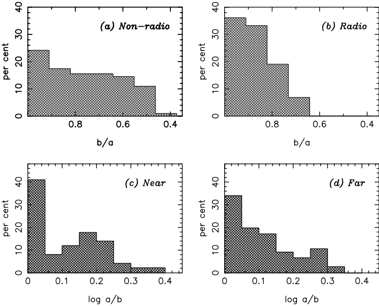
Fig. 5.7. Kolmogorov–Smirnov tests on subsamples of ellipticals from the Disney–Wall (1977) sample of bright ellipticals. Upper panels – distribution functions in b/a , minor to major axis, for (a) the 102 undetected and (b) the 30 radio-detected ellipticals in the sample. The Kolmogorov–Smirnov two-sample test rejects H_0 , that the subsamples are drawn from the same population, at a significance level of < 1 per cent. Lower panels – distribution functions in \log a/b for (c) the 51 ellipticals closer than 30 Mpc, (d) 76 bright ellipticals in the sample more distant than this. The Kolmogorov–Smirnov test indicates no significant difference between these latter subsamples.
