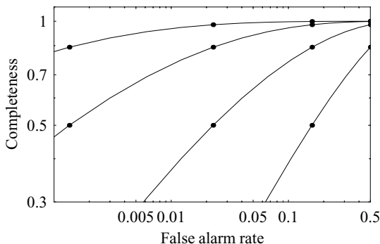
Fig. 7.1. Completeness versus false-alarm rate, plotted for source flux densities in terms of \sigma_{\text{noise}} ranging from 1 unit (right) to 4 units (left). The flux limits are indicated by the dots, starting at zero on the right and increasing by one unit at a time. For example, a 4\sigma source and a 2\sigma flux limit give a false-alarm rate of 2 per cent and a completeness of 99 per cent with the Gaussian noise model.
