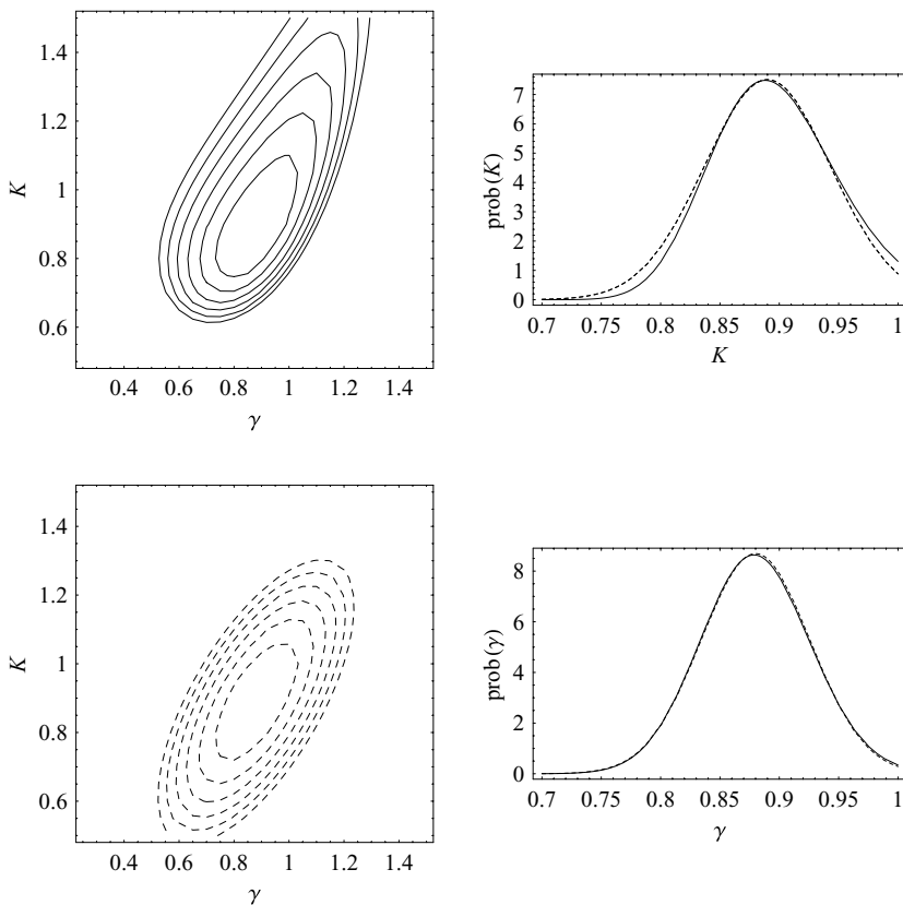
Fig. 6.4. Top left, a contour plot of the log likelihood function; bottom left, the Gaussian approximation; right panels, the marginal distributions of k and \gamma , comparing the Gaussian approximation to the full likelihood.
