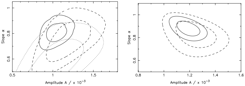
Fig. 9.5. Constraints on the clustering parameters A and \alpha , w(\theta) = A\theta^{-\alpha} . Contours of constant \chi^2 are shown; these are approximate 1\sigma and 2\sigma contours for flux-density thresholds 30 mJy (dotted), 20 mJy (dashed) and 10 mJy (solid). The left diagram is derived from fitting the correlation function (Fig. 9.3) directly; the right diagram from fitting the counts-in-cells variance function shown in the right panel of Fig. 9.4.
