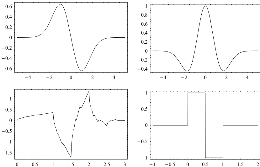
Fig. 8.6. Four possible wavelets; a wavelet decomposition will be in terms of scaled and translated versions of each of these. Top left, asymmetrical; top right, Mexican hat; bottom left, Daubechies (this wavelet is actually a fractal); bottom right, Haar.
