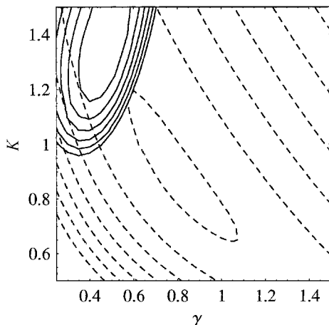
Fig. 6.10. The log likelihoods for the two models; the black contours are for the simplest model, with no provision for offsets; the dashed contours are for the weak hierarchical model, allowing separate offsets at each frequency.
