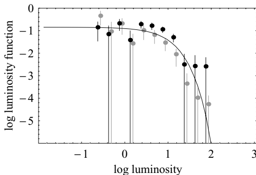
Fig. 7.13. The luminosity probability distribution (black dots), and theoretical distribution (solid line), together with bootstrapped error estimates (the interquartile range is shown). The lighter dots are a V_{\max} estimate, displaced slightly in luminosity for clarity.
