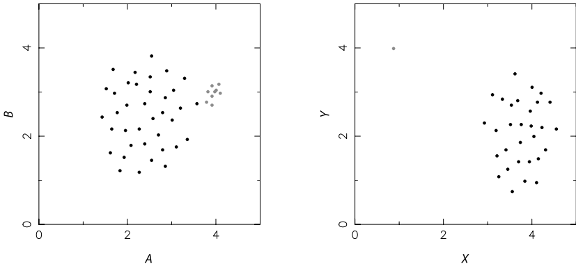
Fig. 4.2. Dodgy correlations: in each case formal calculation will indicate that a correlation exists to a high degree of significance.
