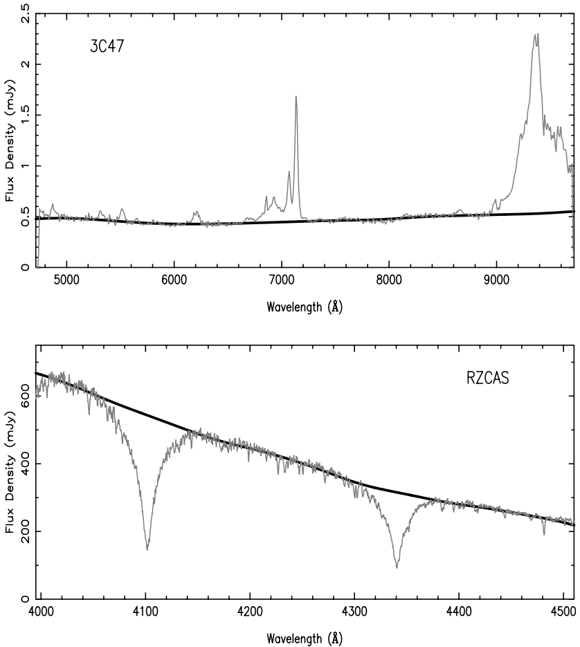
Fig. 8.2. Top a spectrum of 3C47 obtained by Laing et al. (1994) with the Faint Object Spectrograph of the William Herschel Telescope, La Palma. The redshift is 0.345; broad lines of the hydrogen Balmer series can be seen, together with narrow lines of [OIII]. Bottom: a spectrum of the star RZ Cas (Maxted et al. 1994). The continuum obtained with the minimum-component technique is shown as the black line superposed on the original data.
