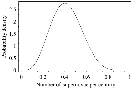
Fig. 2.3. The posterior probability distribution for \rho , given that we have four supernovae in ten centuries.
