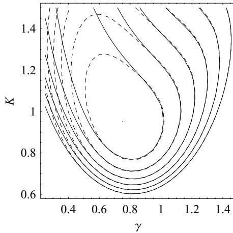
Fig. 6.9. The log likelihoods for the two models; the black contours are for the hierarchical model and the dashed contours are for known \mu .
