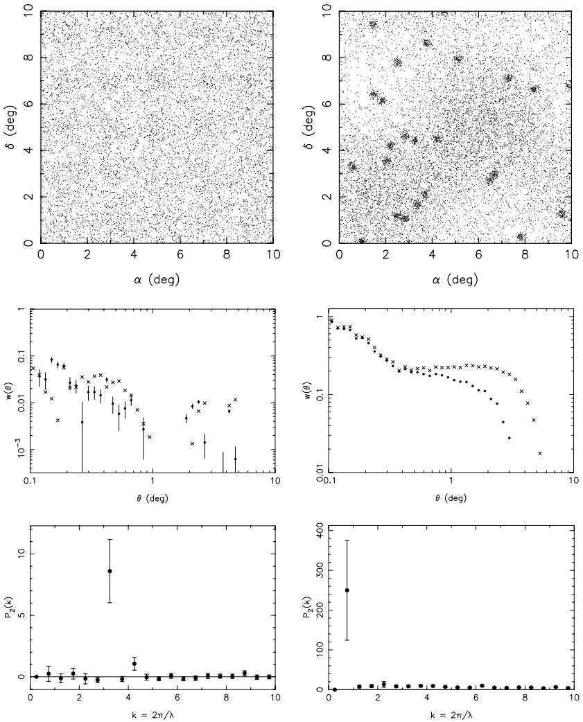
Fig. 9.1. Two sky simulations (see text); left – a uniform 2^\circ grid of 25 low-surface-brightness clusters on a random background, and right – a quadrupole background with 25 randomly placed clusters. Measured w(\theta) and angular power spectra appear below each. The w(\theta) were evaluated with the simple estimator (crosses – equation 9.22) and the Landy–Szalay estimator (dots with error bars – equation 9.25).
