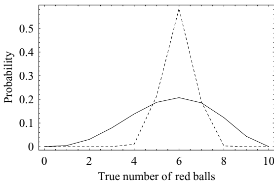
Fig. 2.1. The probability distribution of the number of red balls in the urn, for five (solid curve) and 50 drawings (dashed curve).
