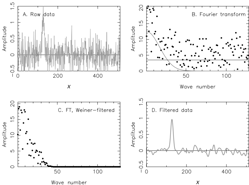
Fig. 8.1. A Wiener filter in action. The raw data of A is a Gaussian sitting on a flat baseline, with random Gaussian noise added. The DFT in B shows the signal and noise components, modelled by the Gaussian and horizontal curves, respectively. The Wiener filter, applied in the frequency domain, produces the DFT of C, and the reverse transform produces the greatly improved signal/noise of D.
