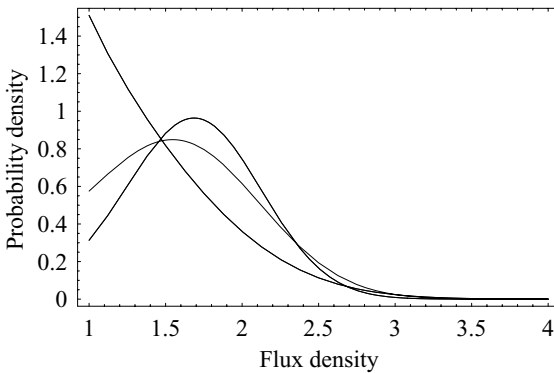
Fig. 2.2. Measurement of flux density given a power-law prior (source count) and a Gaussian error distribution. The posterior probability distribution for flux density is plotted for two, four and then six of the measurements listed in the text; the form of the curve approaches Gaussian as numbers increase.
