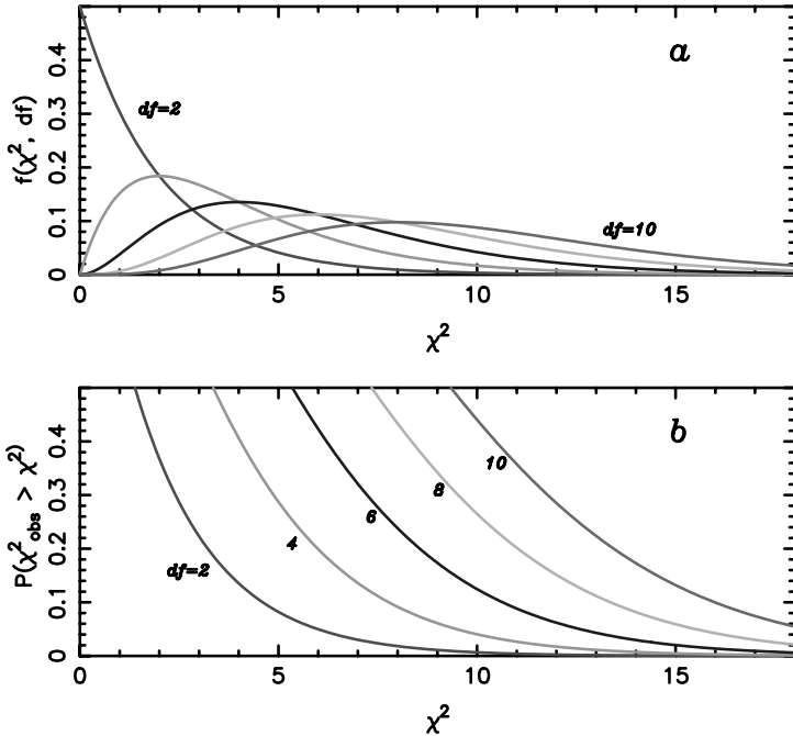
Fig. 5.4. The chi-square distribution: (a) f(\chi^2, df) , the probability density function of \chi^2 for df degrees of freedom; (b) the distribution function \int_{\chi^2}^{\infty} f(\chi^2, df) d\chi^2 of Table A2.6, consulted to determine if \chi^2 is ‘large enough’ to reject H_0 .
