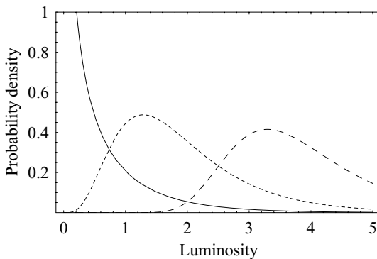
Fig. 3.5. The Schechter luminosity function (solid curve) and the distribution of the maximum of 10 and 100 samples from the distribution, plotted as short- and long-dash curves respectively.
