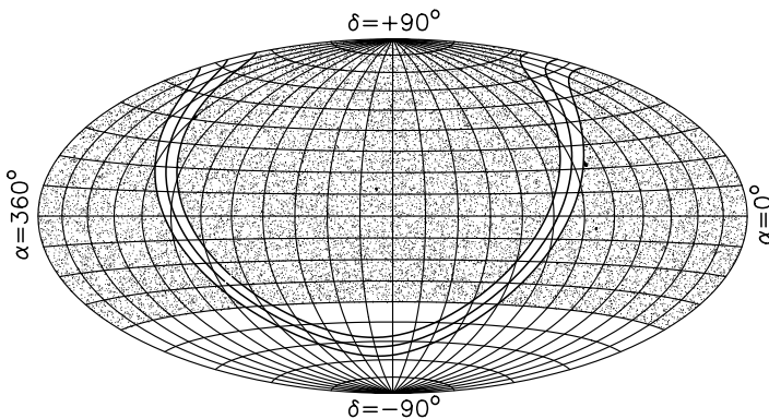
Fig. 9.2. The sources of the NVSS survey; catalogue entries with S_{1.4\text{GHz}} > 200 mJy are plotted on an equal-area projection. The Galactic plane and Galactic latitudes \pm 5^\circ are shown and sources within this region are masked from large-scale structure analysis as most are Galactic in origin.
