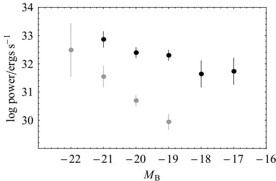
Fig. 7.14. The sample of Sadler, Jenkins & Kotanyi (1989): the 30th-percentile radio power (light symbols) and emission-line power (dark symbols), as a function of absolute magnitude.
