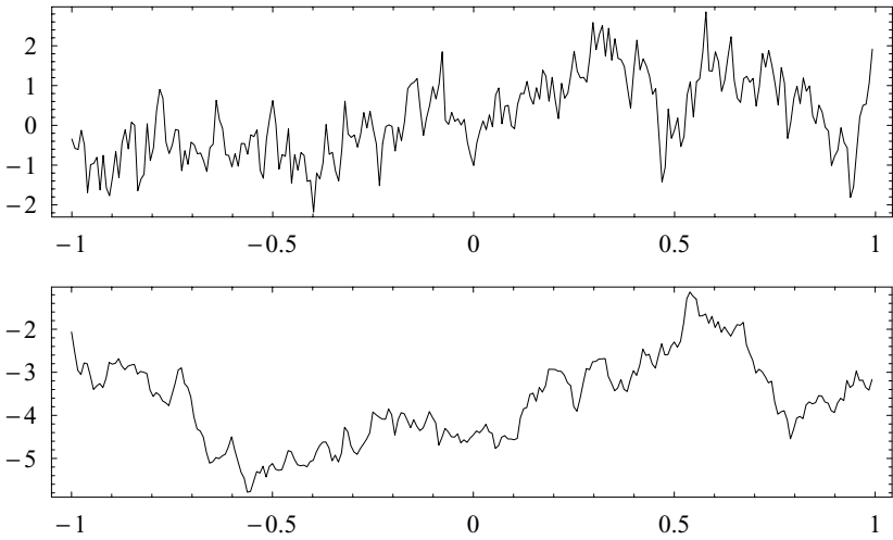
Fig. 8.8. Above: flicker ( 1/f ) noise of unit variance. The data are implicitly band-limited by the finite sampling rate. Below: a random walk of unit variance.
