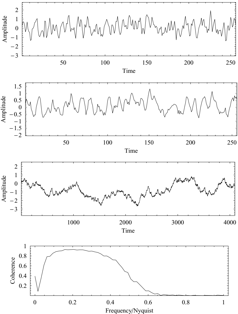
Fig. 8.3. From top to bottom; the input to the system f ; the input, convolved, with a small amount of noise added f \otimes h + \epsilon(t) , the extraneous effect b(t) , and at bottom, the coherence between f and g .
