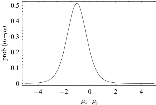
Fig. 5.1. The distribution of the difference of means for the example data.
