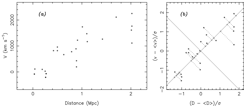
Fig. 4.3. (a) An early Hubble diagram (Hubble 1936); recession velocities of a sample of 24 galaxies versus distance measure. (b) The same plot but with data normalized by standard deviation; the lines represent principal components, as described in Section 4.5.
