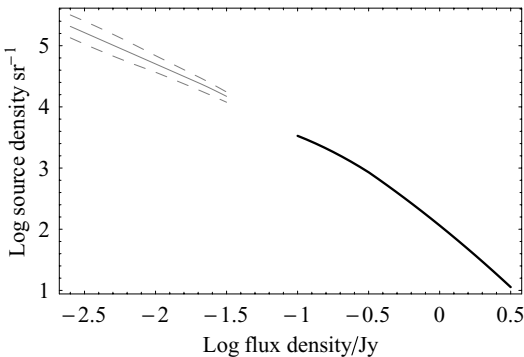
Fig. 7.18. The 2.7-GHz counts from Wall & Cooke (1975): the darker line is derived from ordinary source counts with error bars not much wider than the line, while the p(D) results are shown in grey, the dashed lines representing one standard deviation of the fitted parameters.
