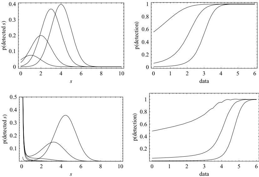
Fig. 7.2. The top left panel shows the probability of a detected source of flux density s ; the curves correspond to measurements of 1–4 units (as before, a unit is one noise standard deviation). A prior \epsilon = 0.05 was used. On the top right these curves are integrated to give the probability of detection at any positive flux density, as a function of the data values; the curves are for \epsilon = 0.5, 0.05 and 0.005 . The bottom panels show the results of the calculation for the power-law prior, truncated at 0.1 unit.
