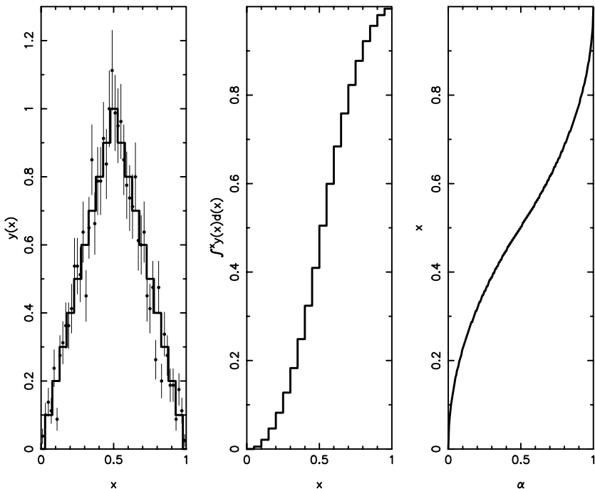
Fig. 6.7. An example of generating a Monte Carlo distribution following a known histogram. Left: the step-ladder histogram, with points from 2000 trials, produced by (a) integrating the function (middle) and (b) transforming the axes to produce f^{-1} of the integrated distribution (right). The points with \sqrt{N} error bars in the left diagram are from drawing 2000 uniformly distributed random numbers and transforming them according to the right diagram.
