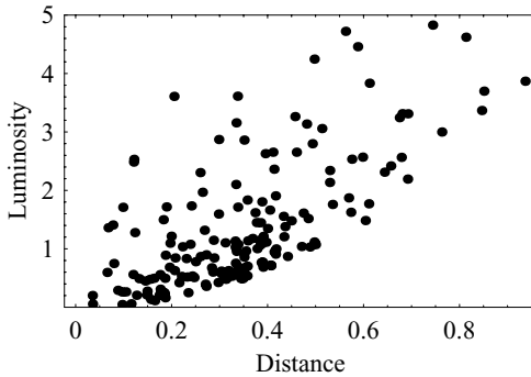
Fig. 7.5. Results of a simulation of a flux-limited survey of galaxies drawn from a Schechter function.
