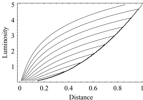
Fig. 7.4. Contour plots of the bivariate \text{prob}(l, r) . The contours are at logarithmic intervals; galaxies tend to bunch up against the selection line, leading to a bogus correlation between luminosity and distance.
