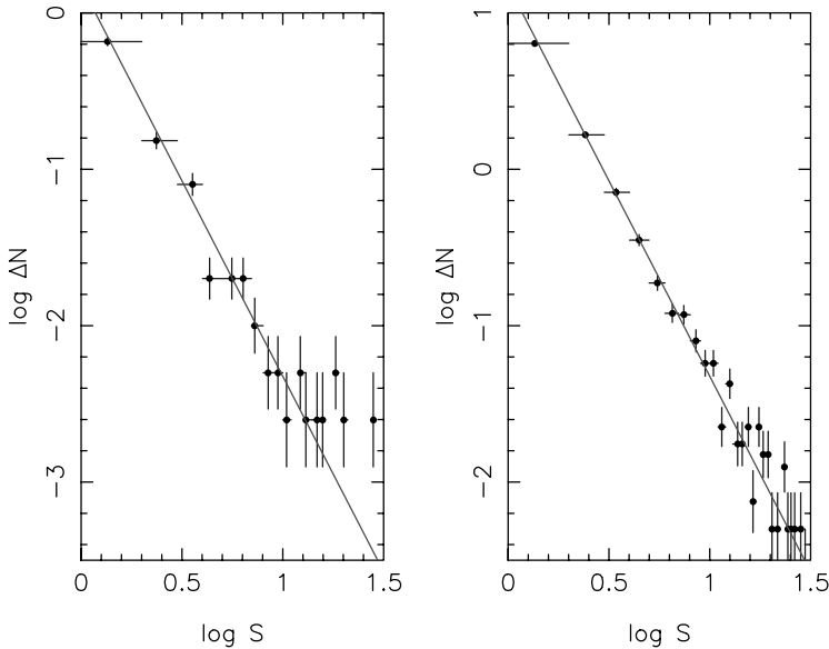
Fig. 6.1. A maximum-likelihood application. The figures show differential source counts generated via Monte Carlo sampling with an initial uniform deviate (see Section 6.5) obeying the source-count law N(> S) = kS^{-1.5} . The straight line in each shows the anticipated count with slope -2.5 : left, k = 1.0 , 400 trials; right, k = 10.0 , 4000 trials. The ML results for the slopes are -2.52 \pm 0.09 and -2.49 \pm 0.03 , the range being given by the points at which the log likelihood function has dropped from its maximum by a factor of 2. The anticipated errors in the two exponents, given by |\text{slope}|/\sqrt{\text{trials}} (see the next-but-one example), are 0.075 and 0.024.
