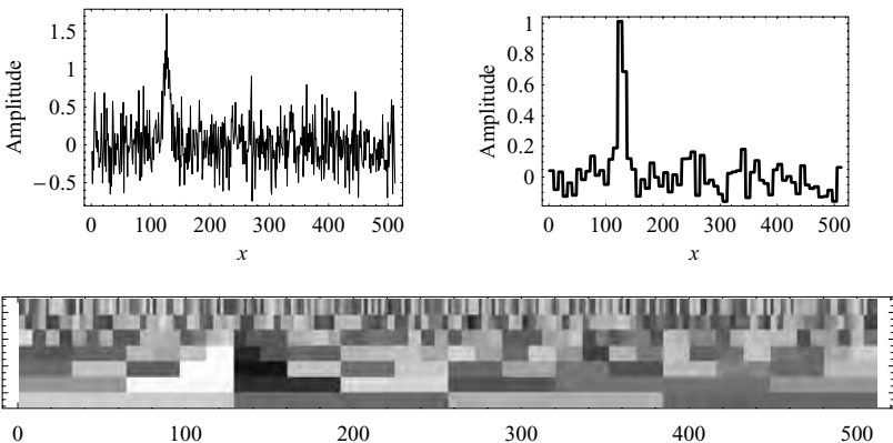
Fig. 8.7. Top left, the original spectrum of Fig. 8.1; top right, the filtered spectrum; bottom, the wavelet coefficients as a function of location and scale.
