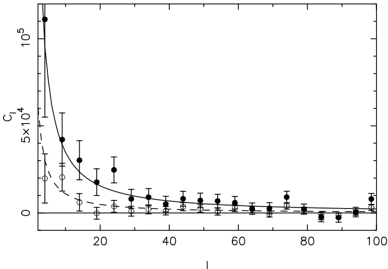
Fig. 9.6. Measurement of the NVSS c_\ell spectrum. Results at flux-density thresholds S_{1.4\text{GHz}} = 10 mJy (solid circles) and 20 mJy (open circles) are plotted. The solid and dashed lines show the prediction of equation (9.45) at these thresholds assuming that w(\theta) = (1 \times 10^{-3})\theta^{-0.8} . The difference in amplitude between the two measurements arises from the factor c_0^2 in equation (9.45).
