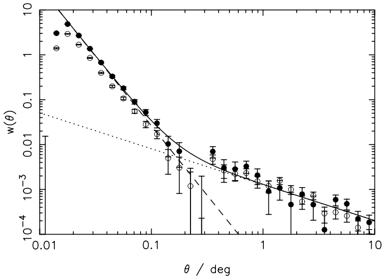
Fig. 9.3. The angular correlation function w(\theta) for the source catalogue of the NVSS survey, at S_{1.4\text{GHz}} = 20 mJy (solid circles) and 10 mJy (open circles). The best-fitting sum of two power laws for the 20 mJy data is shown as the solid line, with the two power laws shown individually, dashed due to multiple-component sources, dotted due to galaxy clustering.
