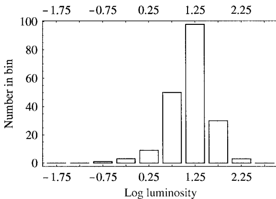
Fig. 7.7. The luminosity distribution for the simulation, in bins 0.5 dex wide, derived from the Schechter function of the previous example with a flux limit of 20 units.
