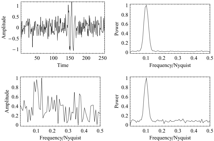
Fig. 8.4. Top left: part of the input data stream for the correlator, consisting of 64 wave packets, randomly located, with on average one per 128 units of time. Top right: the average power spectrum from forming the autocorrelation function over 128 time units. Bottom left: the average Fourier transform of one-bit quantized data, again from 128-long chunks. Bottom right: the power spectrum derived from the quantized data with the same averaging.
