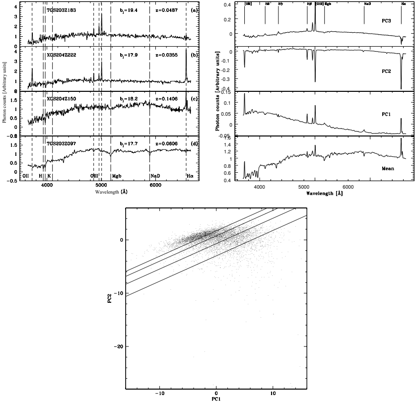
Fig. 4.9. Top left: examples of 2dF spectra prepared for PCA. Instrumental and atmospheric features have been removed, with the spectra transformed to the rest frame, resampled to 4 Å bins and normalized to unit mean flux. Top right: the mean spectrum and first three principal components; the sign of the PCs is arbitrary. Below: distribution of 2dF galaxy spectra in the PC1–PC2 plane. Slanted lines divide the plane into the five spectral classes adopted by Folkes et al.
