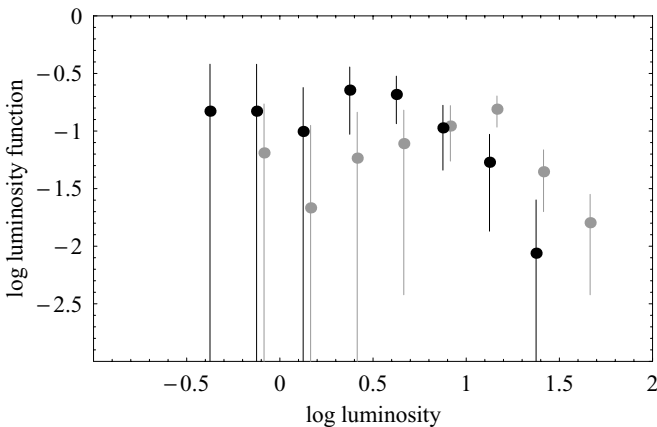
Fig. 7.15. Luminosity functions for two simulated samples drawn from field-galaxy Schechter functions (see text), estimated by the Avni method with bootstrap errors. The error bars are the interquartile ranges.
