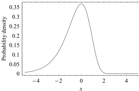
Fig. 3.2. The probability distribution of the logarithm of data drawn from an exponential distribution.
