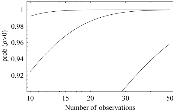
Fig. 4.6. The probability of \rho being positive, as a function of sample size, for r -values of 0.25 (lowest curve), 0.5 and 0.75 (uppermost curve).
