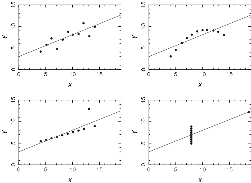
Fig. 4.8. Anscombe's quartet: four fictitious sets of 11 (X_i, Y_i) , each with the same (\bar{X}, \bar{Y}) , identical coefficients of regression, regression lines, residuals in Y and estimated standard errors in slopes.
