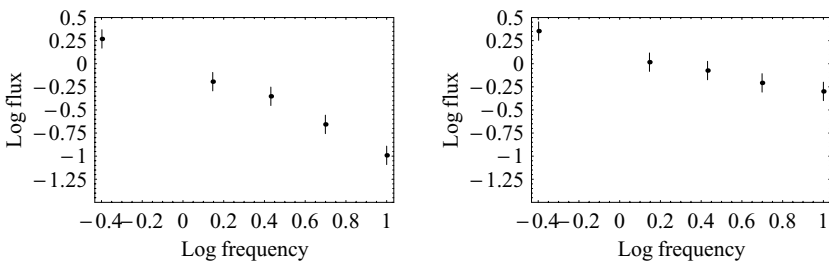
Fig. 6.3. The two experimental spectra we will examine; the right-hand one contains an offset error as well as random noise.
