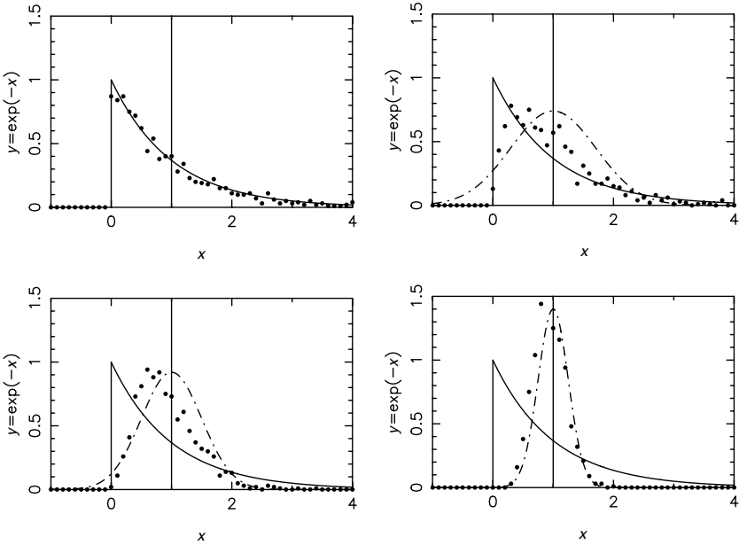
Fig. 2.6. An indication of the power of the central limit theorem. The panels show successive amounts of ‘integration’: in the upper left panel, a single value has been drawn; in the upper right, 200 values have been formed from an average of two values; lower left, 200 values from an average of four; lower right, 200 values from an average of 16.
