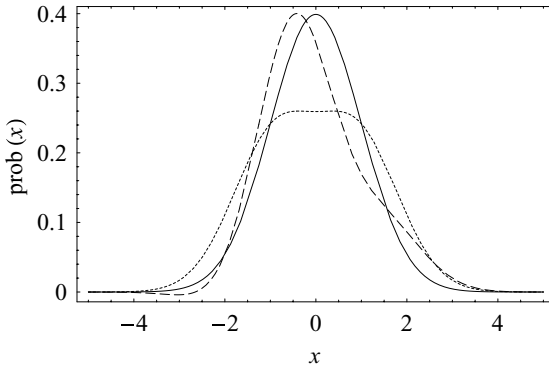
Fig. 5.3. Various distributions resulting from using just two terms in a Gram-Charlier distribution; the solid curve is a pure Gaussian.
