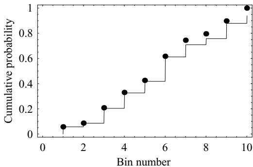
Fig. 7.11. The Kaplan–Meier estimator (solid line), compared to the cumulant derived from the Avni estimator (dots).
