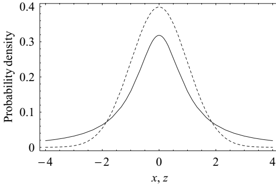
Fig. 3.4. The probability distribution of the ratio of two identical Gaussian variables the original Gaussian is the dashed curve.
