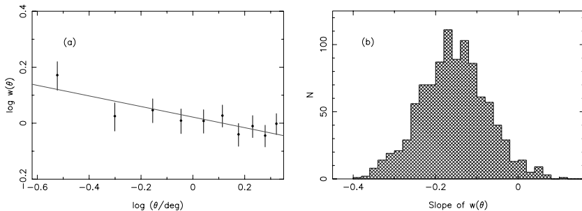
Fig. 6.8. A bootstrap application. (a) The two-point correlation function for 2812 radio sources with extended radio structure, from the White–Becker catalogue of the NRAO 1.4-GHz survey of the northern sky. A least-squares fit gives a slope of -0.19 . (b) The distribution of slopes obtained in bootstrap-testing the sample with 1000 trials. The mean slope is -0.157 , while the rms scatter is \pm 0.082 ; the slope is less than zero (i.e. signal is present) for 96.8 per cent of the trials.
