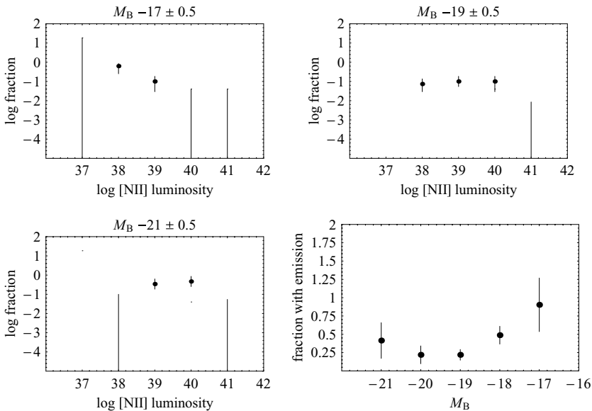
Fig. 7.9. Top left and right, bottom left: estimates of the normalized emission-line luminosity function, derived from the V_{\max} method. Bottom right: the integral of the normalized functions, plotted against absolute optical magnitude. The fraction of galaxies producing emission lines appears to fall with increasing optical luminosity.
