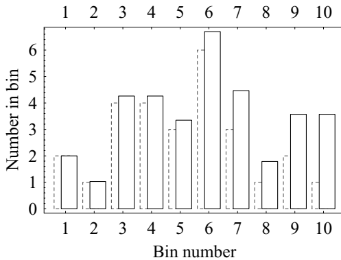
Fig. 7.10. Distribution of spectral indices (optical to X-ray) for a sample of optically selected quasars, showing the observed distribution (dashed boxes) and the estimated true distribution (solid boxes) after including the lower limits.
