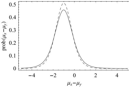
Fig. 5.2. Distribution of the difference of means assuming equal variances (dashed) and without this assumption (solid).
