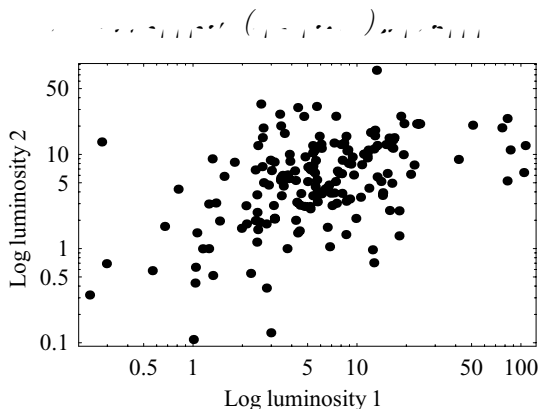
Fig. 7.6. Results of a simulation of a flux-limited survey of galaxies, where each galaxy has two statistically independent luminosities associated with it.
