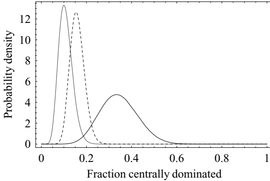
Fig. 2.4. The posterior probability distribution for the fraction of X-ray-selected clusters that are centrally dominated. The black line uses a uniform prior distribution for the fraction; the dashed line uses the prior derived from an assumed previous sample in which 10 out of 100 clusters had dominant central members. The light curve shows the distribution for this earlier sample.
