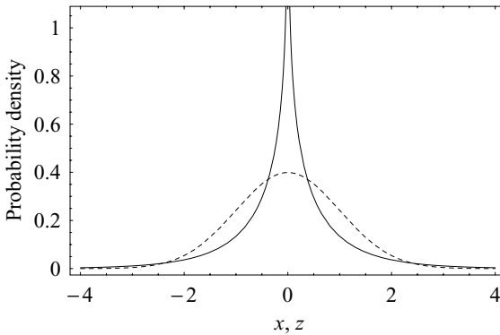
Fig. 3.3. The probability distribution of the product of two identical Gaussians – the original Gaussian is the dashed curve.
