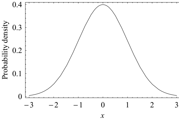
Fig. 2.5. The Normal (Gaussian) distribution. The area under the curve is 1.00; the area between \pm 1\sigma is 0.68; between \pm 2\sigma is 0.95; and between \pm 3\sigma is 0.997.
