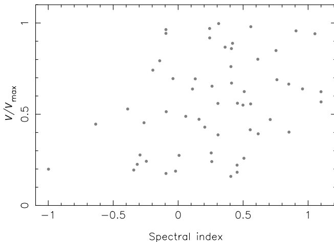
Fig. 4.7. V/V_{\max} as a function of high-frequency spectral index for a sample of radio quasars selected from the Parkes 2.7-GHz survey.
