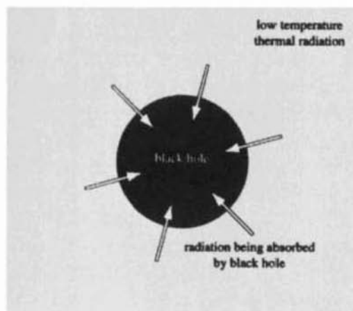
Figure 1.17 A black hole in contact with thermal radiation will absorb some of the radiation, but classically cannot send anything out.
