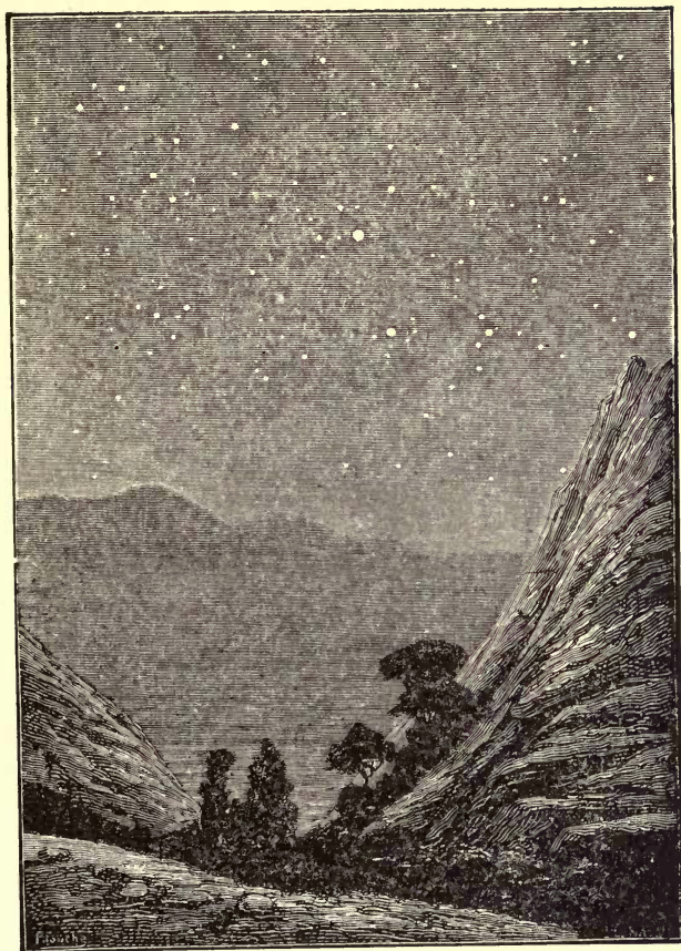
FIG. 1.—The great Book of the Heavens is open to all eyes.
