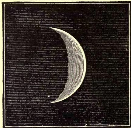
FIG. 38.—Venus at greatest brilliancy.
