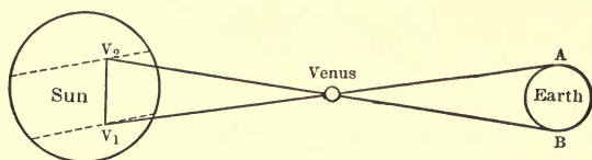
FIG. 83.—Measurement of the distance of the Sun.
