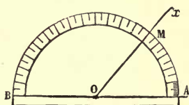
FIG. 80.—Measurement of Angles.
