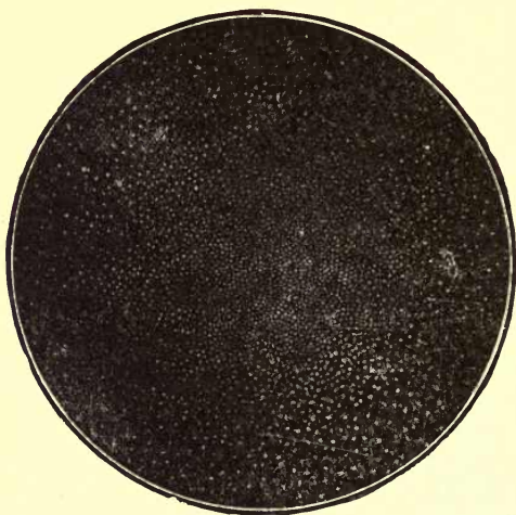
FIG. 22.—The Star-Cluster in the Centaur.
