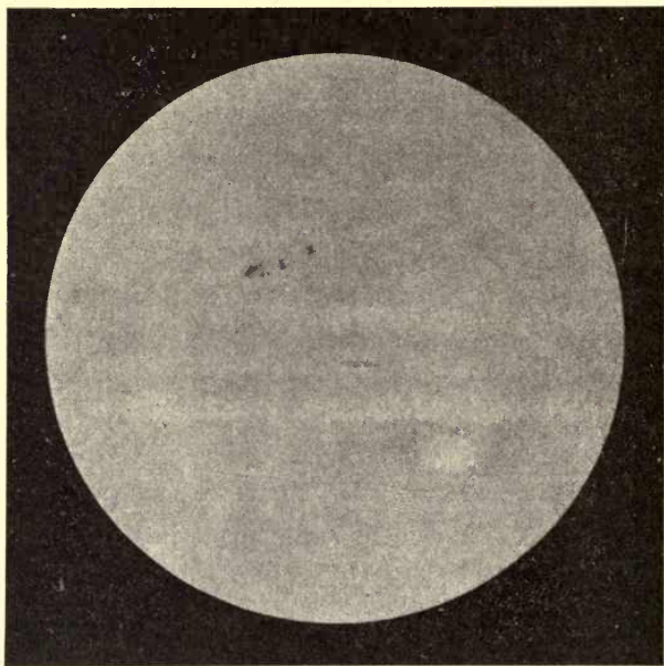
FIG. 29.—Direct photograph of the Sun.
