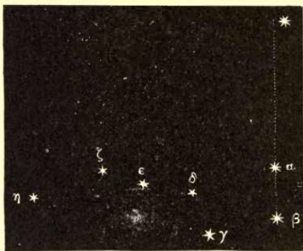
FIG. 3.—The Great Bear (or Dipper), and the Pole-Star.
