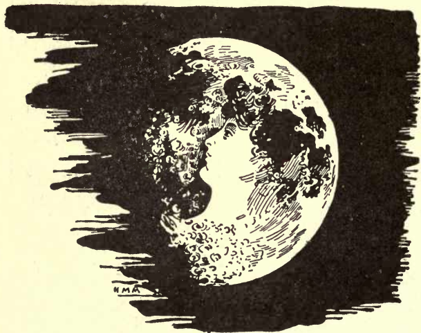
FIG. 67.—Woman's head in the Moon.
