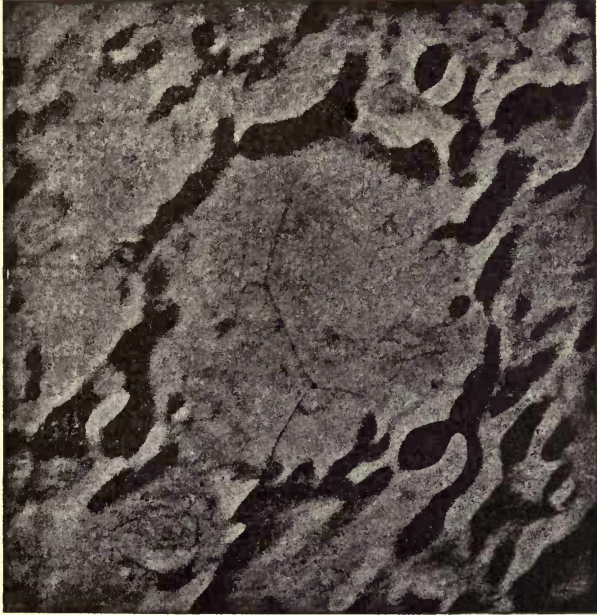
FIG. 73.—Flammarion's Lunar Ring.
