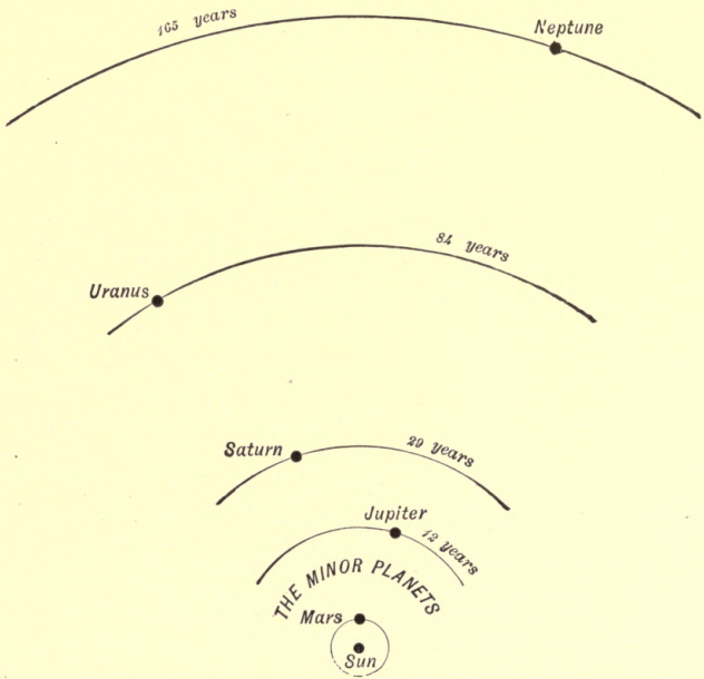
FIG. 33.—Orbits of the four Planets farthest from the Sun.
