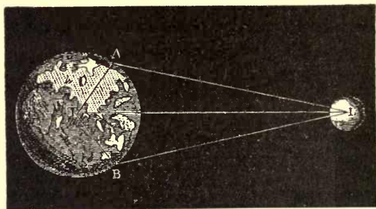
FIG. 82.—Measurement of the distance of the Moon.
