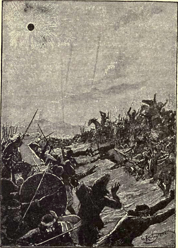
FIG. 75.—Battle between the Medes and Lydians arrested by an Eclipse of the Sun.
