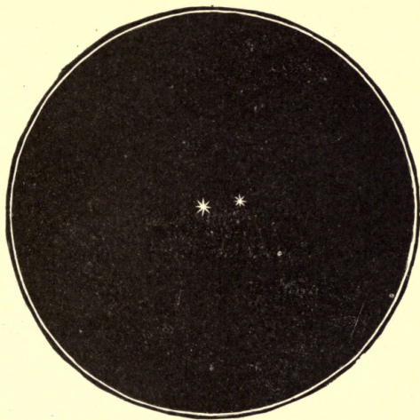
FIG. 17.—The double star Mizar.
