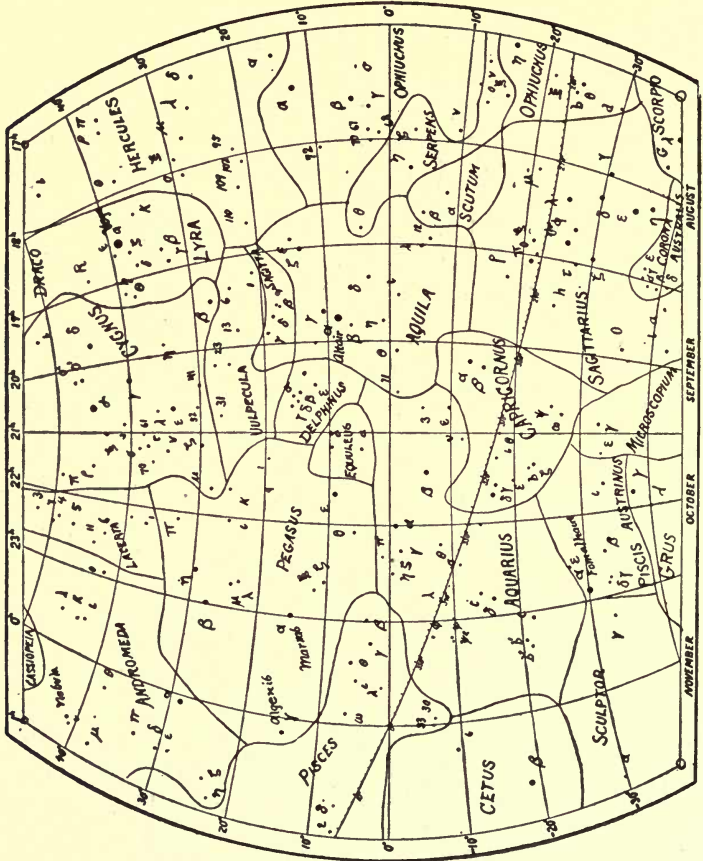
Fig. 16.—Autumn Constellations.
