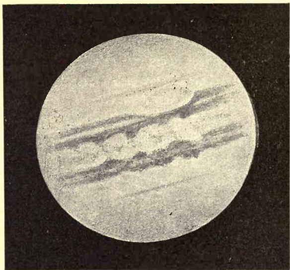
FIG. 45.—Telescopic aspect of Jupiter.
