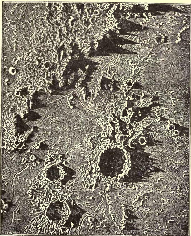
FIG. 72.—The Lunar Apennines.
