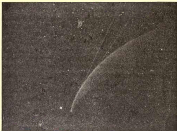
FIG. 49.—The Great Comet of 1858.
