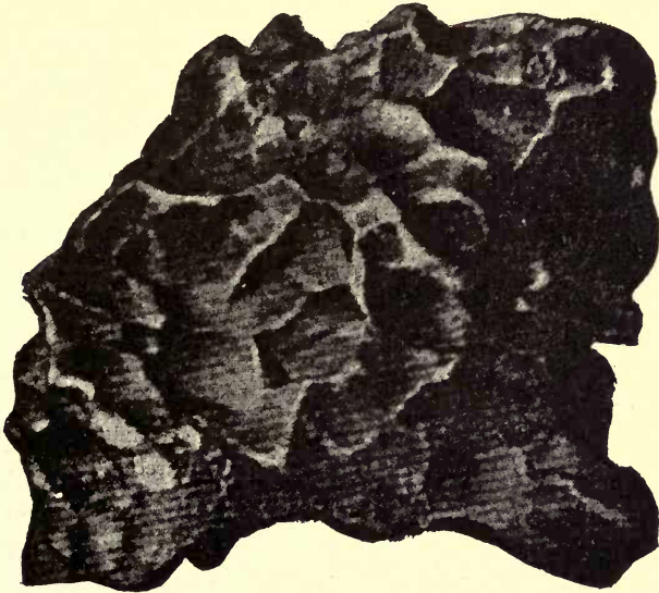
FIG. 59.—A Uranolith.
