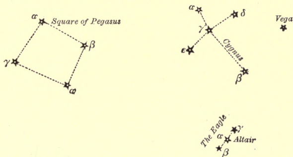
FIG. 9.—The Swan, Vega, the Eagle.
