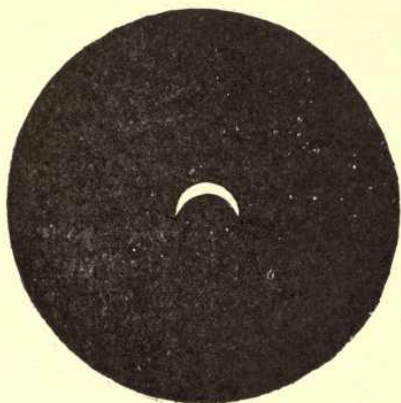
FIG. 79.—The Eclipse of May 28, 1900, as photographed by King Alfonso XIII, at Madrid.
