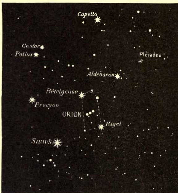
FIG. 12.—Orion and his celestial companions.
