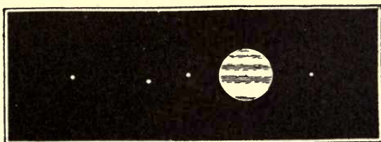
FIG. 46.—Jupiter and his four principal satellites.
