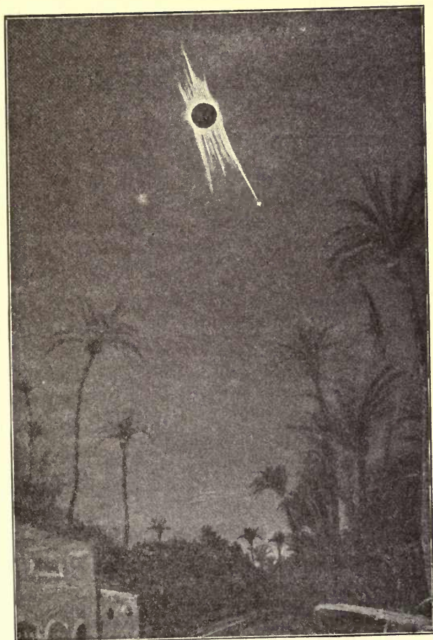
FIG. 78.—Total eclipse of the Sun, May 28, 1900, as observed from Elche (Spain).
