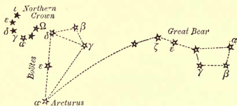
FIG. 8. —To find Arcturus, the Herdsman, and the Northern Crown.
