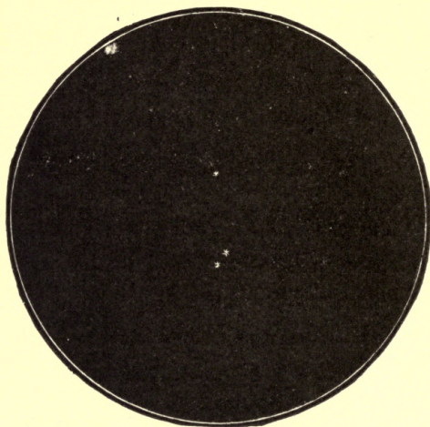
FIG. 18.—Triple star \zeta in Cancer.
