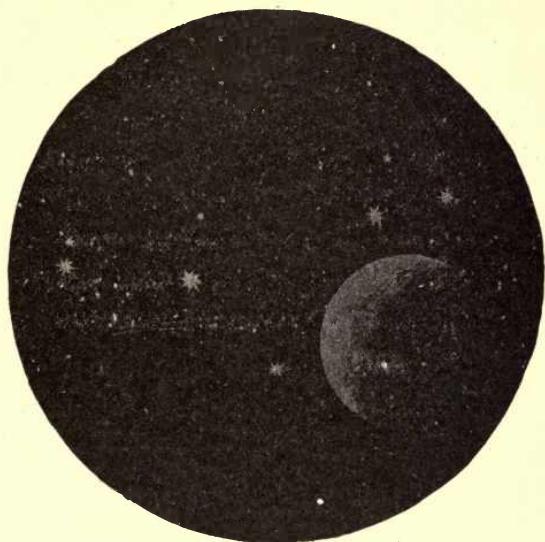
FIG. 26.—Occultation of the Pleiades by the Moon.
