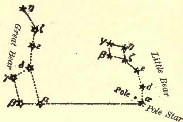
FIG. 4.—To find the Pole-Star.
