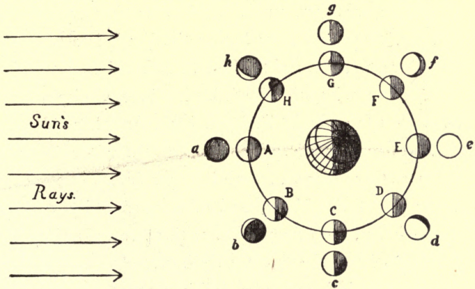
FIG. 70.—The Moon's Phases.
