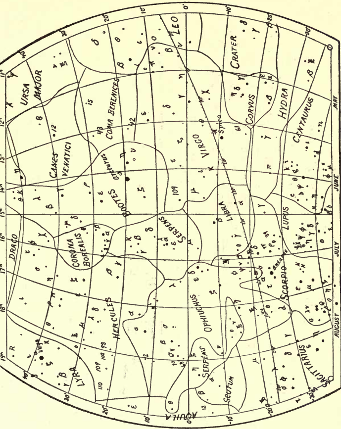
FIG. 15.—Summer Constellations.
