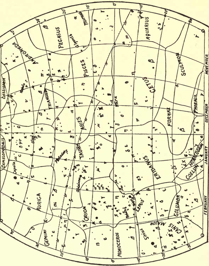
FIG. 13.— Winter Constellations.
