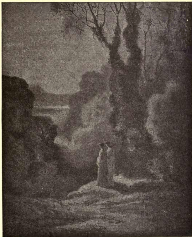
FIG. 36.—The Evening Star.
