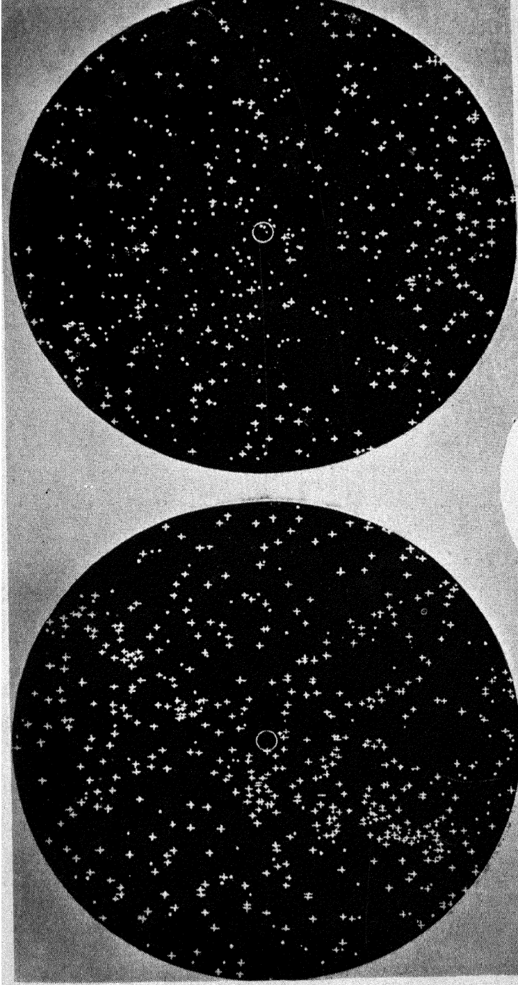
CHART OF HEMISPHERE OF SKY FROM WHICH THE SUN IS RECEDING. PLATE 1.
