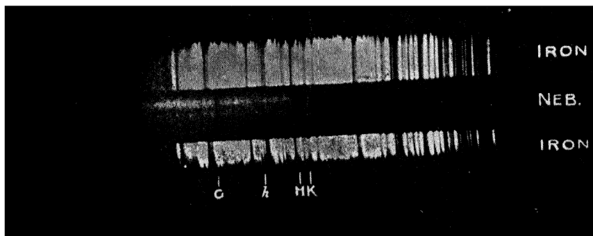
PLATE 8b—SPECTRUM OF THE NUCLEUS OF THE SPIRAL NEBULA M81, NGC 3031.
