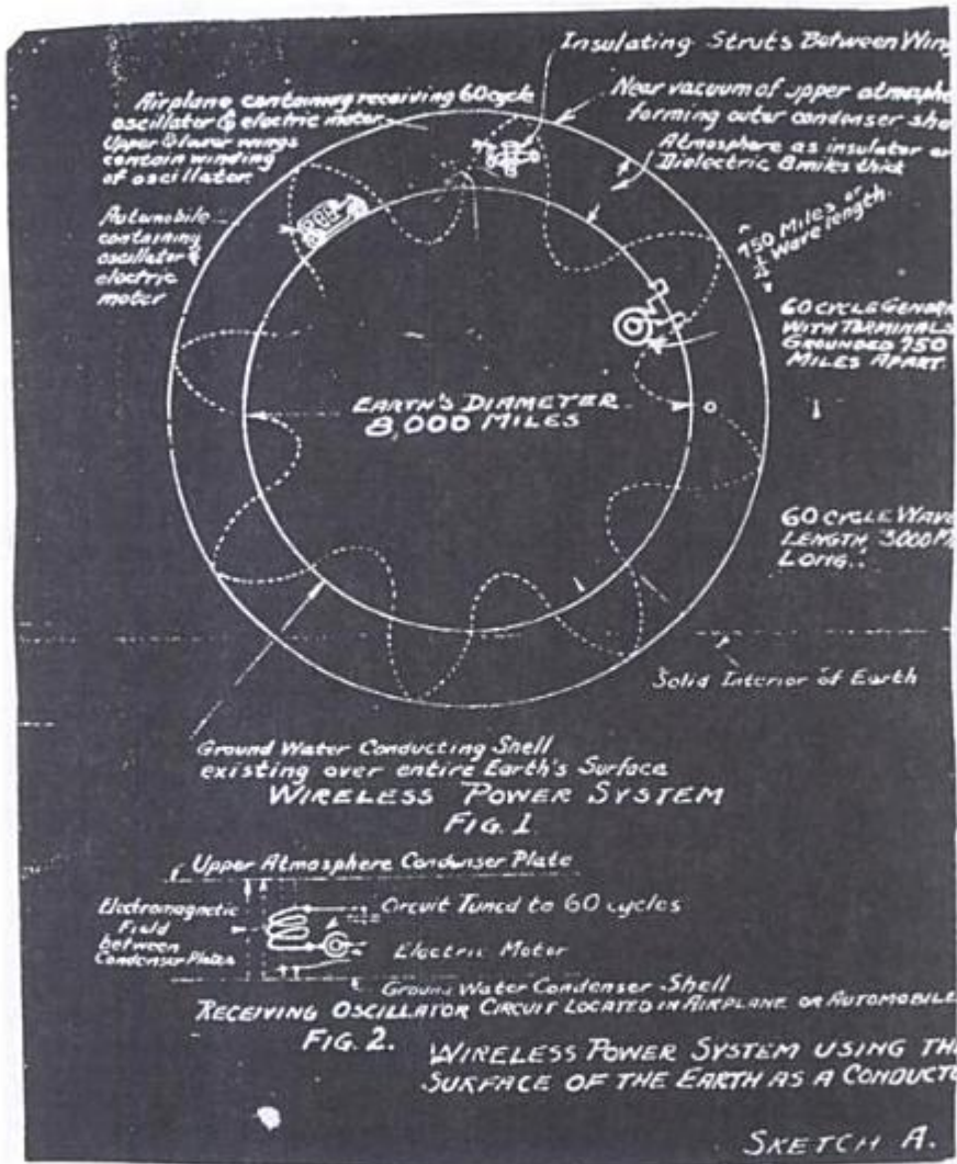
Tesla's sketch of the terrestrial resonator operating at a frequency of 60Hz. He has drawn a standing wave with 8 cycles. This gives the fundamental as 60/8 = 7.5\text{Hz} . The sketch is from a memo in 1925
