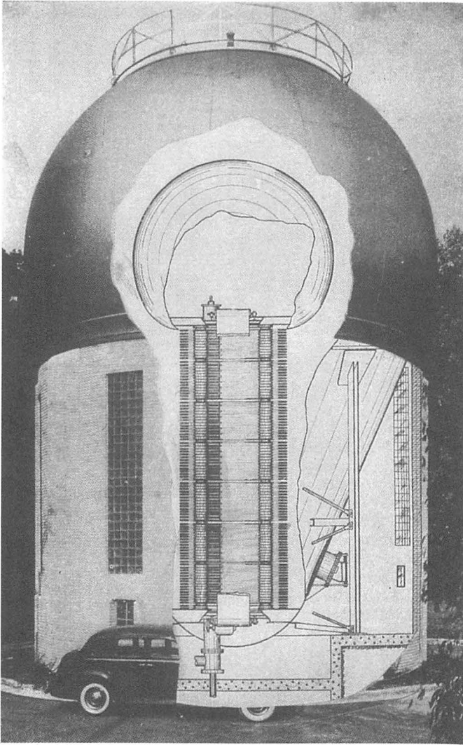
This electrostatic atom-smasher was built at the Carnegie Institution in Washington D.C., and used between 1920 and 1940. The cross-section shows a spherical conductor, its insulating supports, and tube in which particles are accelerated. The charging belt is shown cut-off near the top and bottom. This structure was also the talk of "death-rays."
