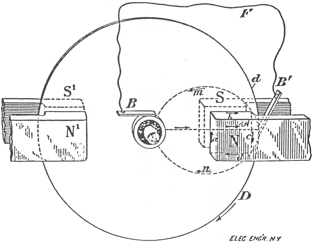
General schematic of a homopolar generator.
