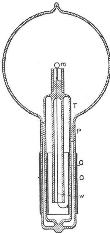
FIG. 22.—TYPE OF BULB WITHOUT LEADING-IN WIRE.
