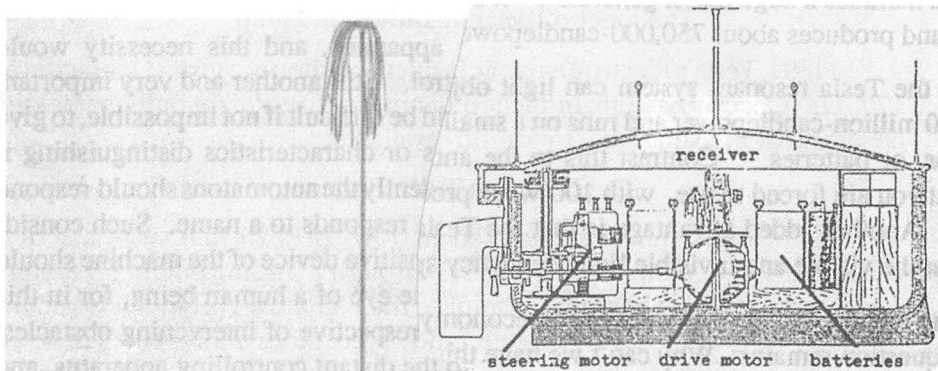
Tesla's Telautomaton Boat US Patent 613,809 -- 1898
