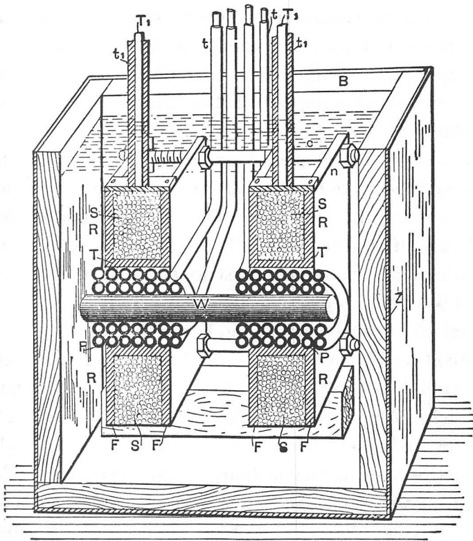
FIG. 3.—DISRUPTIVE DISCHARGE COIL.
