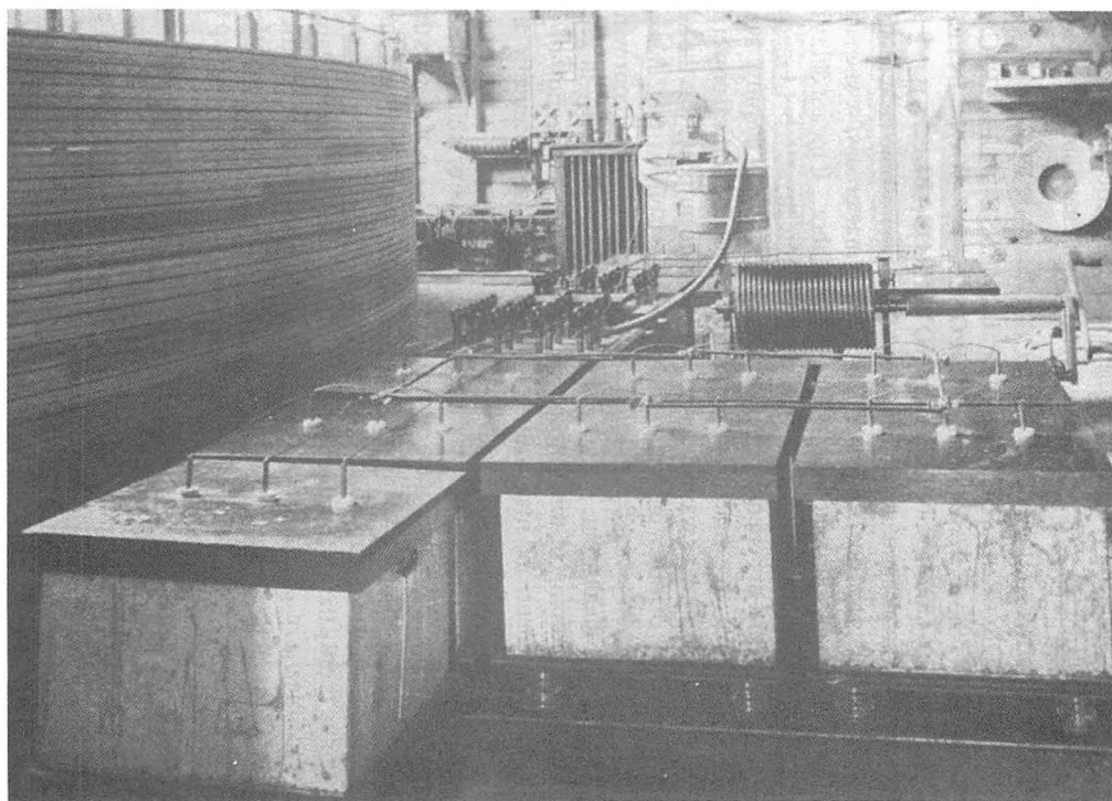
Interior views of Tesla's experimental Colorado Springs tower, showing the cage generating voltage and the banks of batteries.
