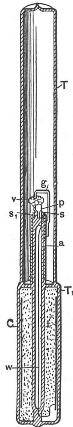
FIG. 35.—CROOKES' EXPERIMENT IN ELECTROSTATIC FIELD.
