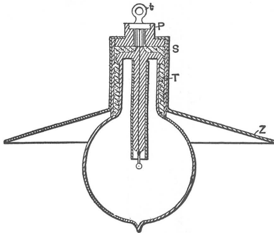
FIG. 26.—IMPROVED BULB WITH INTENSIFYING REFLECTOR.
