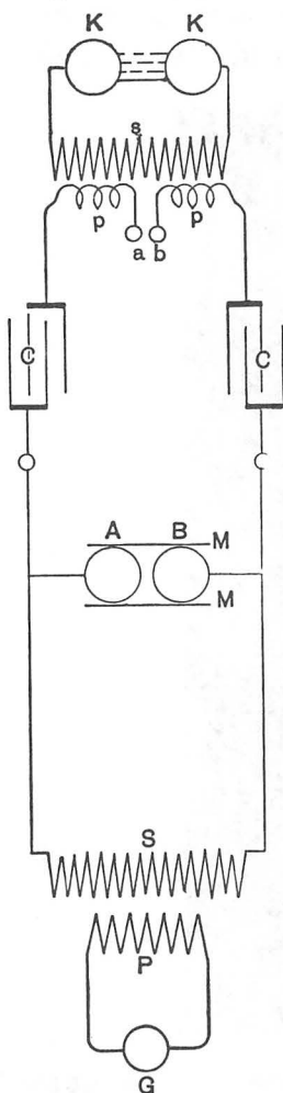
FIG. 2.—IMITATING THE SPARK OF A HOLTZ MACHINE.
