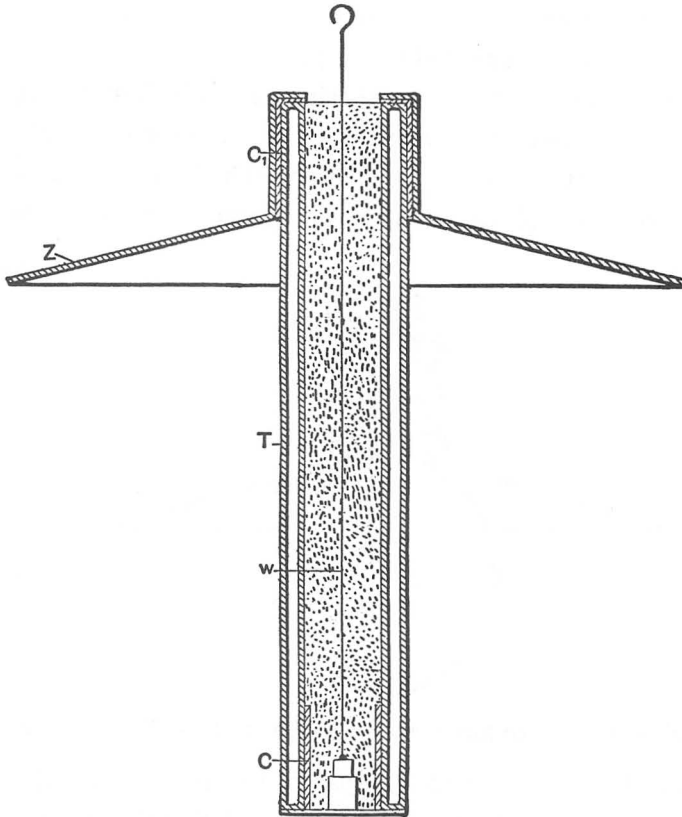
FIG. 27.—PHOSPHORESCENT TUBE WITH INTENSIFYING REFLECTOR.
