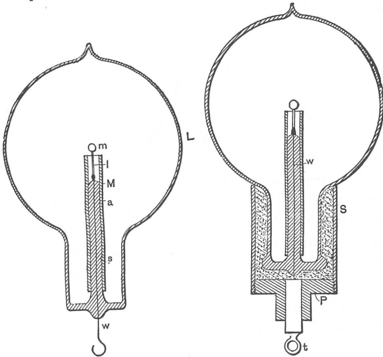
FIG. 18.—BULB WITH MICA TUBE AND ALUMINIUM SCREEN. FIG. 19.—IMPROVED BULB WITH SOCKET AND SCREEN.
