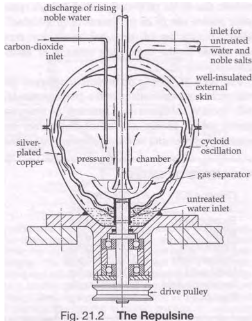
Fig. 21.2 The Repulsine
