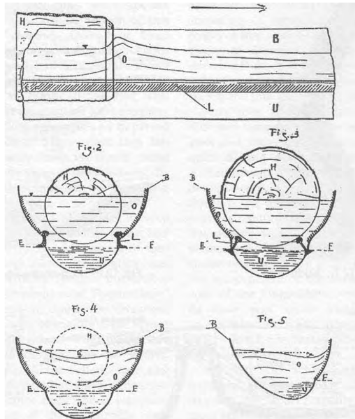
Fig. 12.13 Illustrations from Schauburger's patent application
