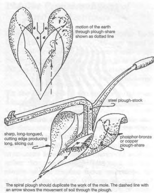
Fig. 19.5 & 6 "The Bio-Plough", 1948
