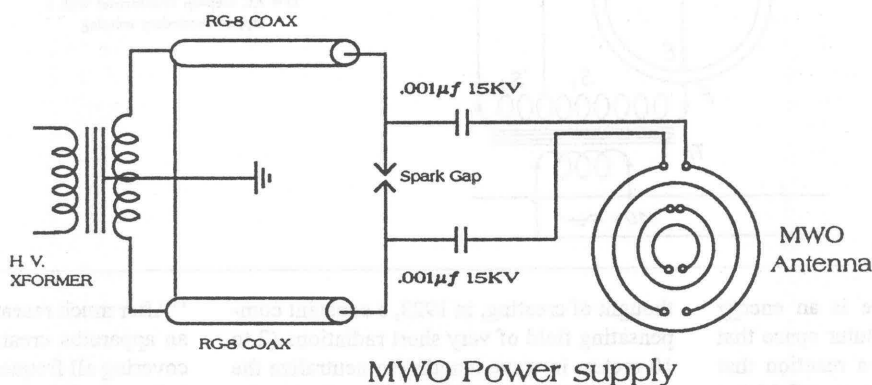
Eric Dollard's suggestions for single antenna hookup
