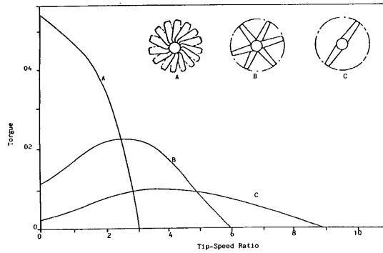
Figure 4: Solidity and torque
