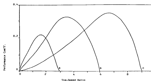
Figure 3: Tip speed ratio and the performance coefficient
