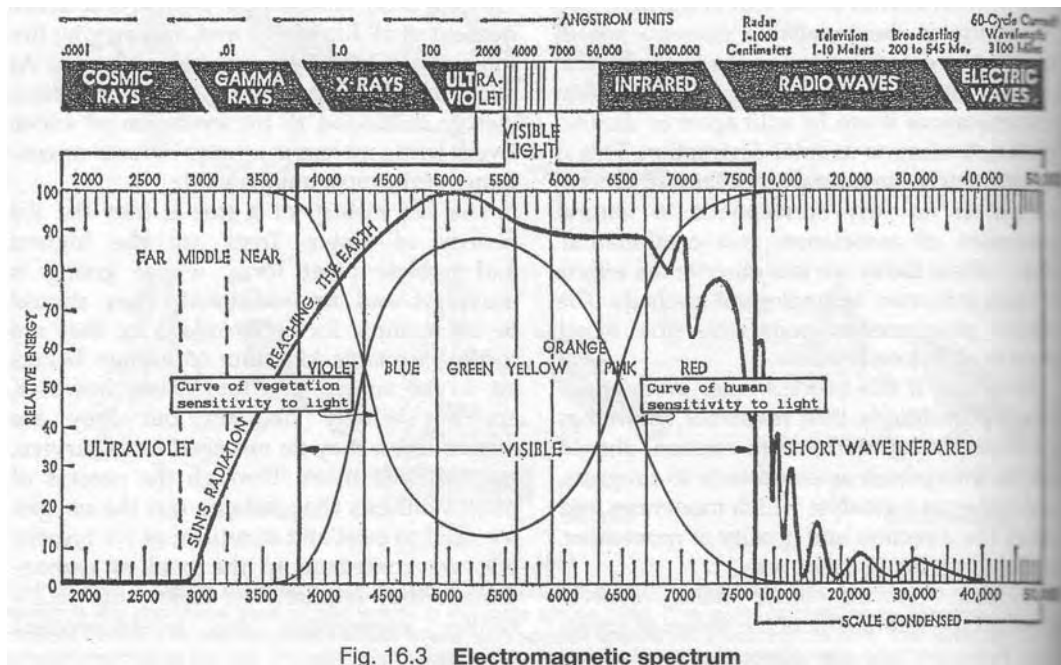
Fig. 16.3 Electromagnetic spectrum
