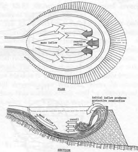
Fig. 12.9 Egg-shaped holding basin
