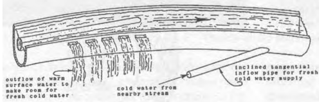
Fig. 12.12a Detail of warm/cold water exchange
