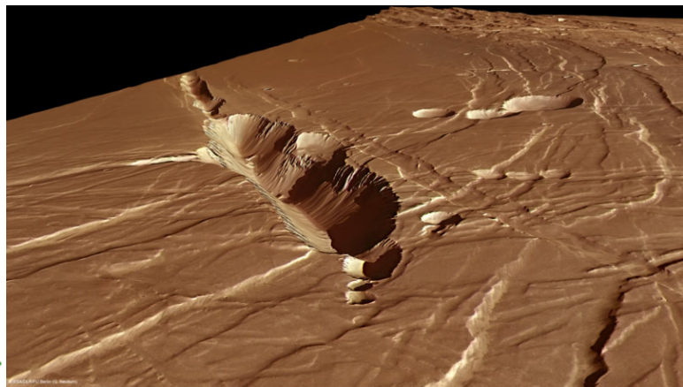
▶ Phoenicis Laqcus Rille on Mars Credit ESA/DLR/FU Berlin (G. Neukum)
