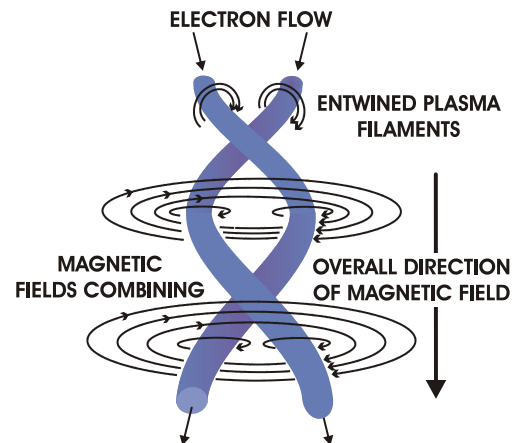
The magnetic forces that keep Birkeland currents together © author ►
