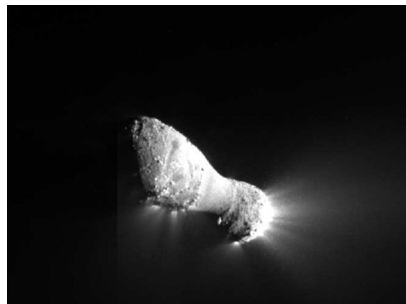
Comet Hartley displaying its “jets” Credit: EPOXI_NASA JPL-Caltech UMD
