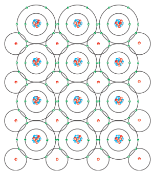
◀ Lattice structure of Ice © author
