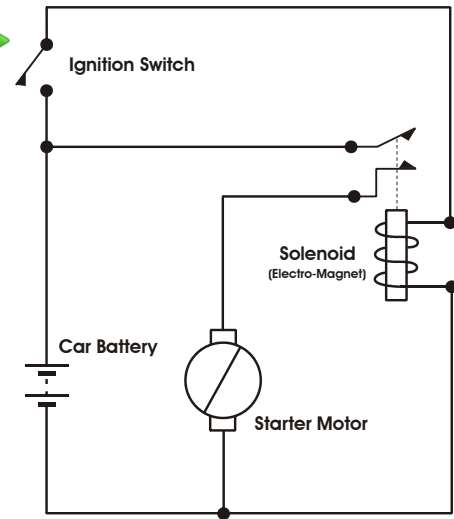
Car starter switching circuit © author ▶
