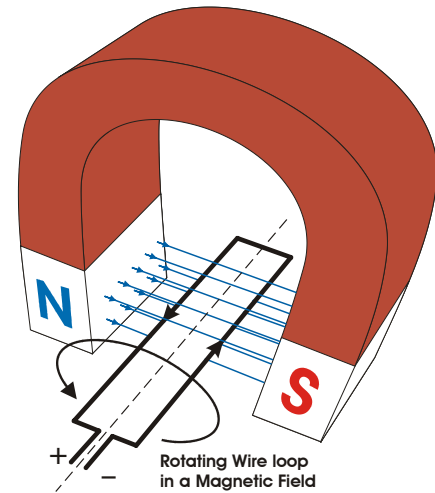
Basic DC Generator © author ▶
