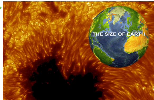
A Sunspot compared to the size of the Earth (adapted image) ▶ Original Image Credit: SST Royal Swedish Academy of Sciences
