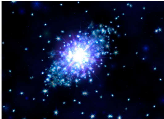
◀ A Nova event? © author
