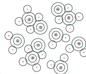
Unstructured water molecules © author ▶
