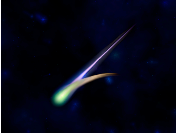
◀ The two tails of a typical comet nearing the Sun © author
