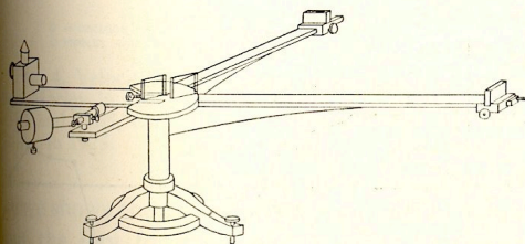
Fig. 1. Michelson's ether-drift interferometer of 1881.
