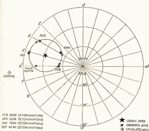
FIG. 28. Observed and calculated apexes of the absolute motion of the solar system.
