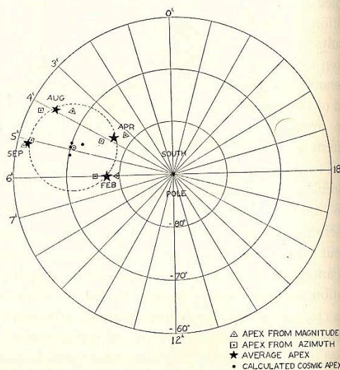
FIG. 23. Chart of the observed apexes of the resultant absolute motion of the earth.
