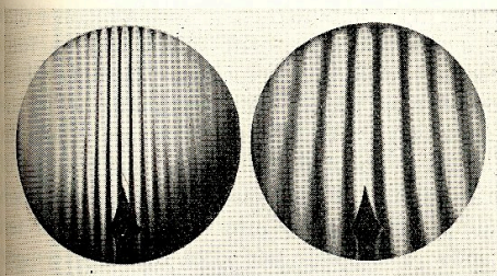
FIG. 7. The interference fringes as seen in the interferometer.
