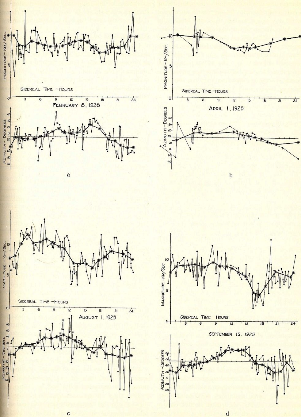
FIG. 22. Single observations and average curves for the ether-drift effect at Mount Wilson in 1925-1926.
