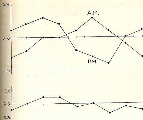
Fig. 11. Method of combining the ether-drift observations of July, 1904, now considered erroneous.
