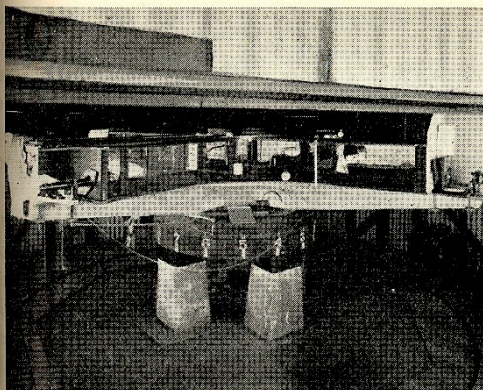
FIG. 13. Interferometer with base of concrete, 1921.
