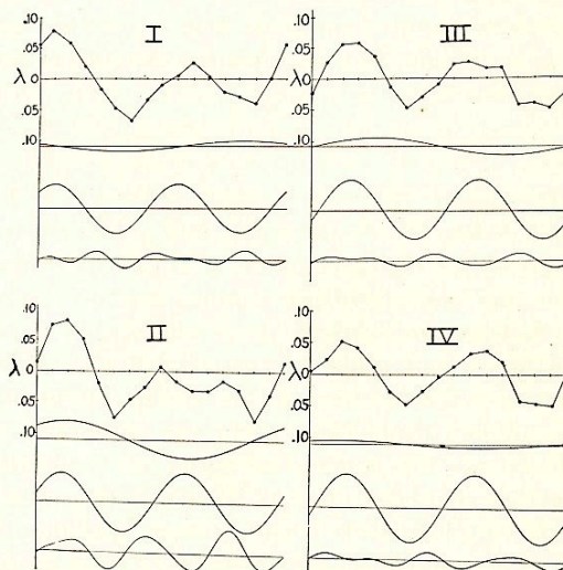
FIG. 21. Harmonic analysis of ether-drift observations.
