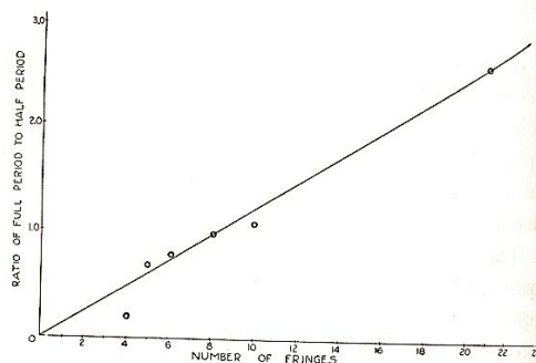
FIG. 30. The full-period effect; the relation of amplitude to width of fringes.
