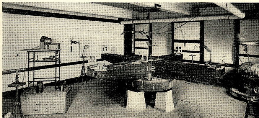
FIG. 14. The interferometer in the laboratory, 1923.
