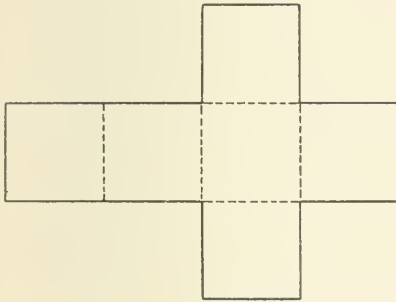
CUBE.
