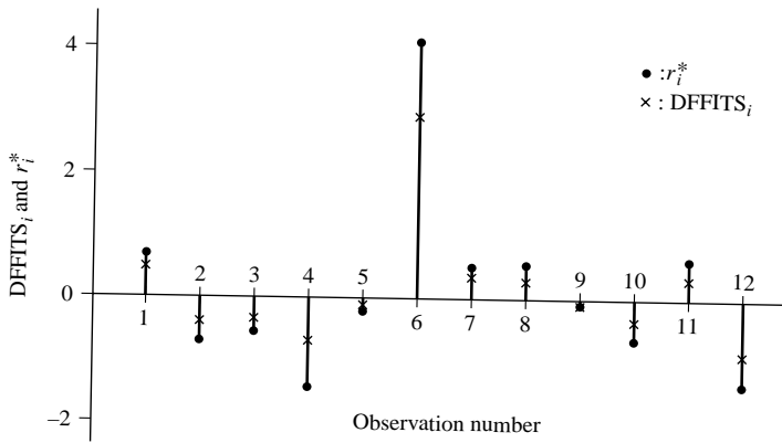
FIGURE 11.14. Studentized residuals and DFFITS_i plotted against observation number from the regression of seed weight on ozone level and cumulative solar radiation using the Lesser–Unsworth data.
