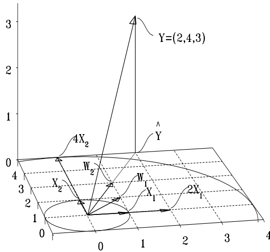
FIGURE 6.6. Projection of Y onto the two-dimensional space spanned by X_1 and X_2 . \hat{Y} is equal to the sum of 2X_1 and 4X_2 . Any two other vectors in the floor of the plot, say W_1 and W_2 , will be linear combinations of X_1 and X_2 and will define the same space. \hat{Y} is also obtained as a linear function of W_1 and W_2 ; \hat{Y} = 0W_1 + 2W_2 .
