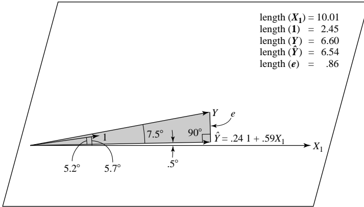
FIGURE 6.5. Geometric interpretation of the regression of heart rate at rest ( Y ) on kilograms body weight ( X_1 ). The plane in the figure is the X -space defined by \mathbf{1} and \mathbf{X}_1 . The data are from Exercise 1.4 with both \mathbf{X}_1 and \mathbf{Y} scaled by \frac{1}{20} . Angles between vectors are shown in degrees. \mathbf{Y} protrudes away from the plane at an angle of 7.5^\circ . Perpendicular projection of \mathbf{Y} onto the plane defines \hat{\mathbf{Y}} which forms an angle of 5.2^\circ with \mathbf{1} and .5^\circ with \mathbf{X}_1 .
