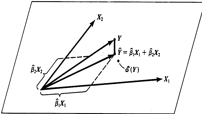
FIGURE 6.3. The geometric relationship of Y and \hat{Y} to the X -space. Y is not in the plane defined by X_1 and X_2 . The perpendicular projection from Y to the plane defines the vector \hat{Y} , which is in the plane. The estimated regression coefficients are the proportions of X_1 and X_2 that, when added, give \hat{Y} . The short vector connecting \hat{Y} to Y is the vector of residuals e .
