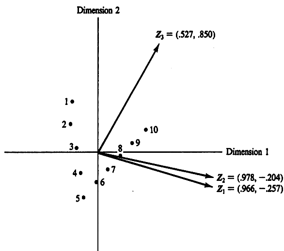
FIGURE 13.1. Gabriel's biplot of the first two principal component dimensions for Example 13.3.
