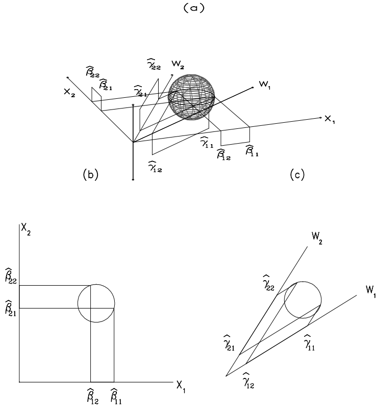
FIGURE 6.8. Illustration of the effect of collinearity on the stability of the partial regression coefficients. The points in the shaded sphere centered on the plane [panel (a)] represent 95% of a population of three-dimensional vectors \mathbf{Y} . \mathcal{E}(\mathbf{Y}) is at the center of the sphere and at the center of the circle of projections of all \mathbf{Y} onto the two-dimensional plane spanned by either the two orthogonal vectors \mathbf{X}_1 , \mathbf{X}_2 or the two nonorthogonal (somewhat collinear) vectors \mathbf{W}_1 and \mathbf{W}_2 . Points shown on opposite sides of the circle represent \hat{Y}_1 and \hat{Y}_2 , projections from two independent \mathbf{Y} . The parallelograms connecting each \hat{Y} to the two sets of vectors show the relative magnitudes of the partial regression coefficients for the pair of orthogonal vectors [panel (b)] and the pair of nonorthogonal vectors [panel (c)].
