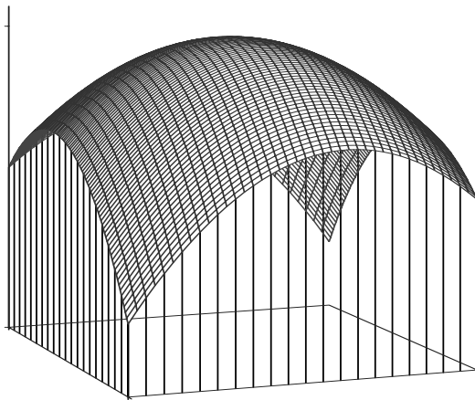
FIGURE 8.7. A bivariate quadratic response surface with a maximum.
