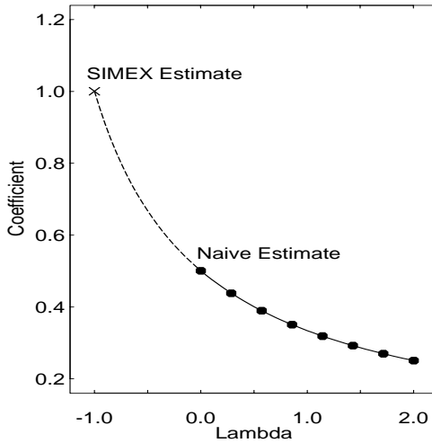
FIGURE 10.1. A generic plot of the effect of measurement error of size (1 + \lambda)\sigma_U^2 on the slope estimates. The ordinary least squares estimate occurs at \lambda = 0 and the SIMEX estimate is an extrapolation to \lambda = -1 .
