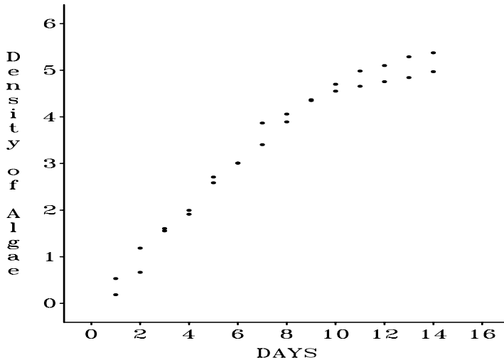
FIGURE 8.1. Algae density versus days of study.
