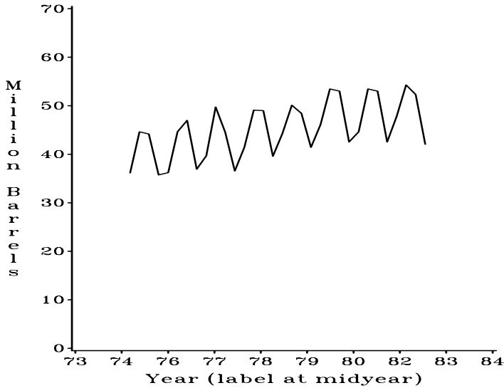
FIGURE 8.3. Quarterly U.S. beer production versus time.
