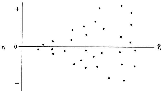
FIGURE 11.3. Plot of e versus \hat{Y} showing increasing dispersion (larger variance) with larger \hat{Y} .
