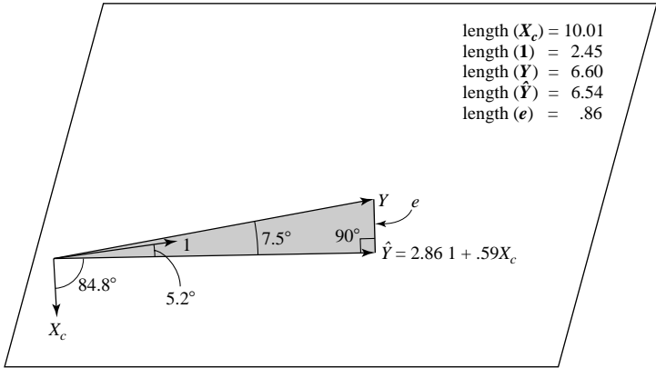
FIGURE 6.7. Geometric interpretation of the regression of heart rate at rest ( Y ) on kilograms body weight using the centered variable ( X_c ). The plane in the figure is defined by \mathbf{1} and \mathbf{X}_c and is identical to the plane defined by \mathbf{1} and \mathbf{X}_1 in Figure 6.5. All vectors are the same as in Figure 6.5 except \mathbf{X}_c replaces \mathbf{X}_1 .
