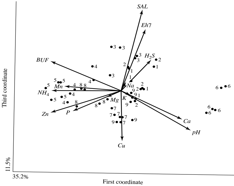
FIGURE 14.2. Gabriel's biplot of the first and third principal components of the 14 marsh substrate variables. The variables are centered and scaled so that all vectors have unit length in 14-dimensional Z-space. The third principal component accounted for 11.5% of the dispersion in the Z-space. Column markers are shown with the vectors, row markers with the •.
