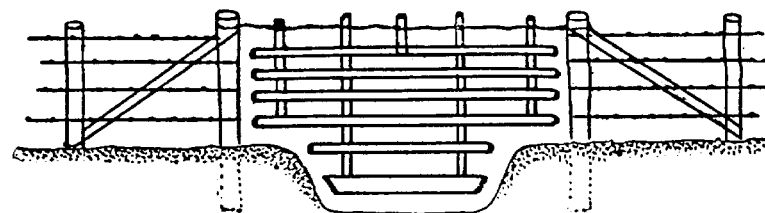
SUSPENDED GATE
