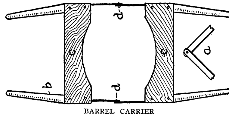
BARREL CARRIER
