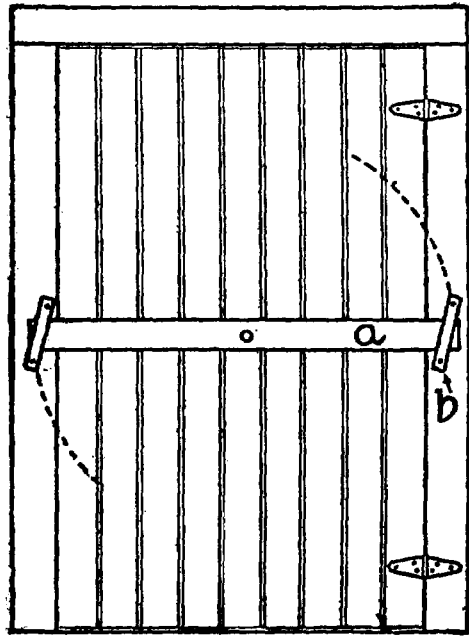
FIGURE 1—LONG FASTENER
