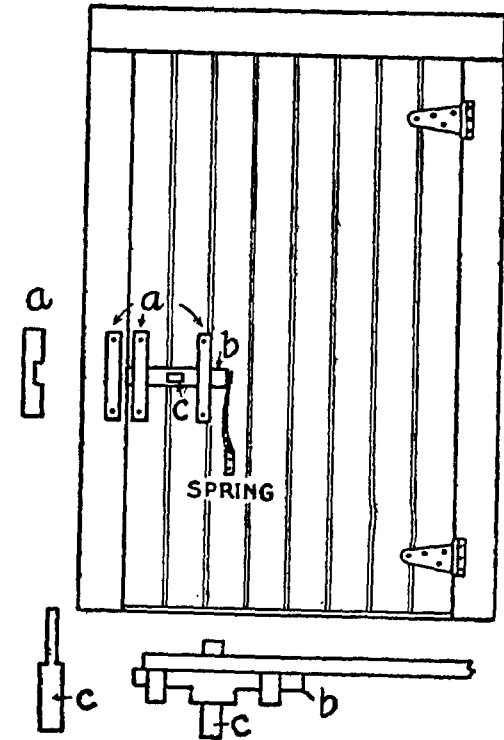
FIGURE 2—SPRING FASTENER
