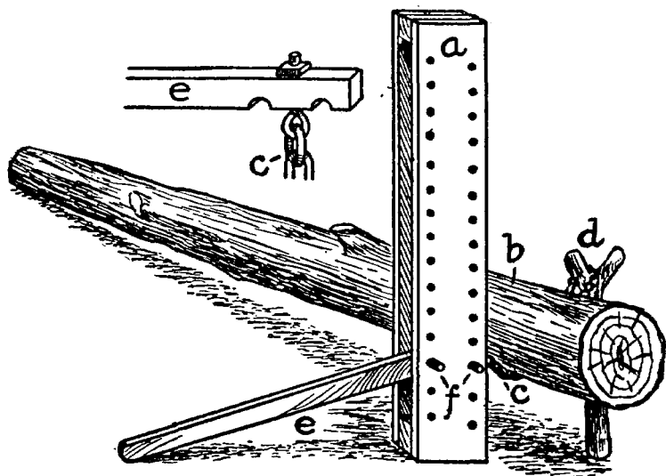
FIGURE 4—LOG JACK
