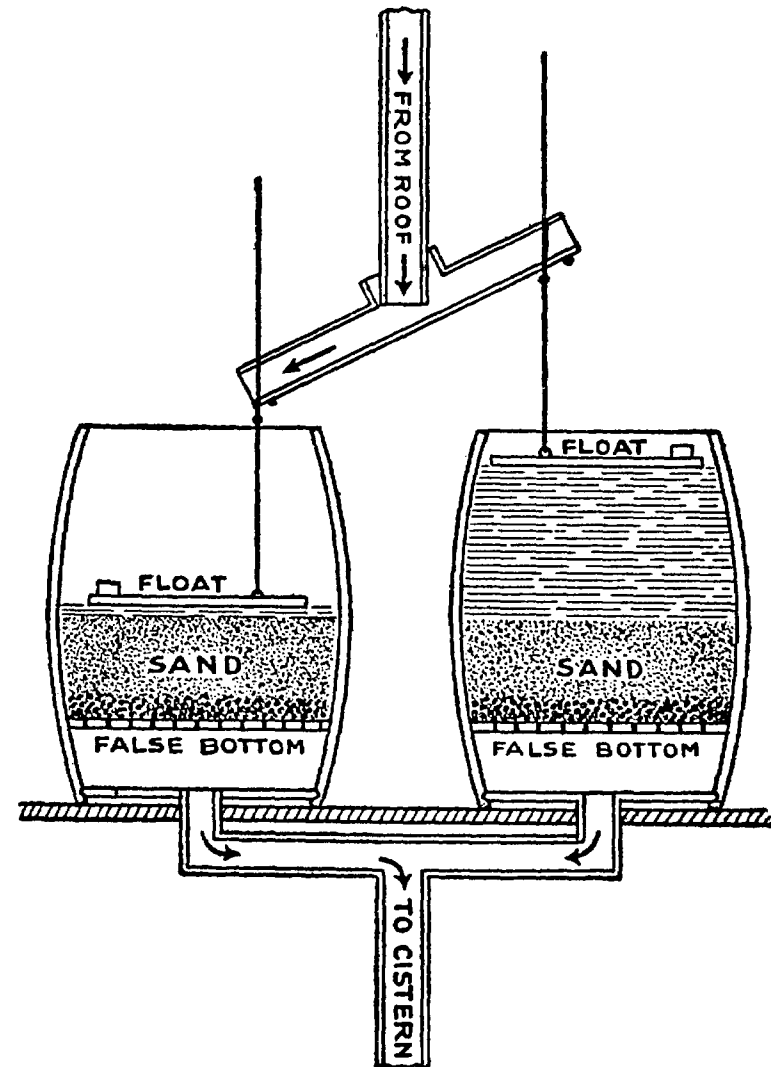
TWO-BARREL FILTER
