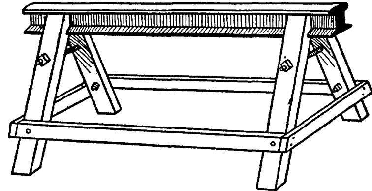
RAIL ANVIL
