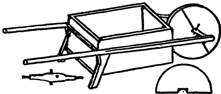
BOX WHEELBARROW
