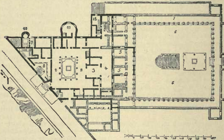
(2) * PLAN OF VILLA SUBURBANA of M. Arvius Diomedes (Donaldson's Pompeii , ii 1). 1, door. 2, peristylum . 3, tablinum . 4, gallery. 5, æcus . 6, court. 7, cryptoporticus . 8, triangular court with cold bath. 9, tepidarium . 10, caldarium . 11, bedroom. 12, staircase leading to lower story.
