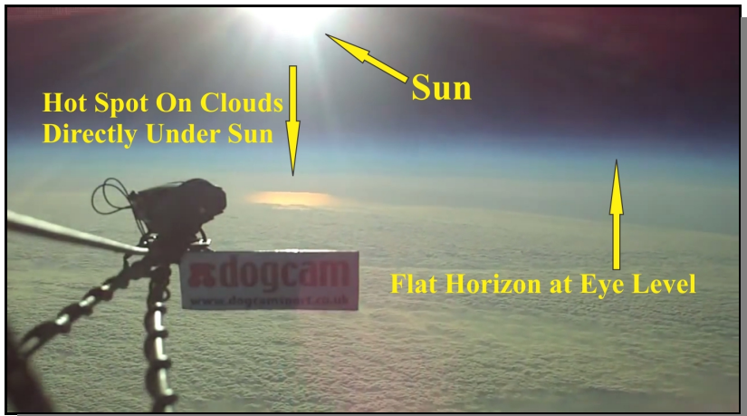
Figure 67: Flat horizon at eye level from an altitude of 80,000 feet. Note the hot spot on the clouds directly under the sun, which indicates that the sun is much smaller than the earth and close overhead.
