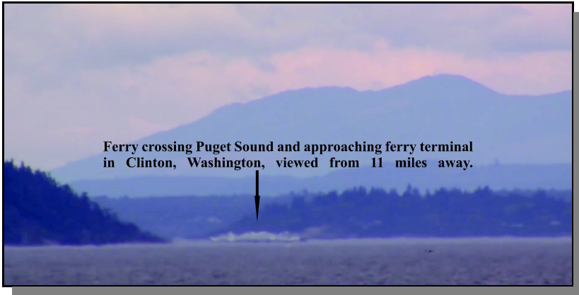
Figure 24: Frame from video of ferry taken from 11 miles away.
