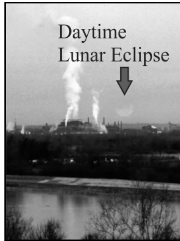
Figure 91: December 2011 Daytime Lunar Eclipse Viewed From East Saint Louis, Illinois
