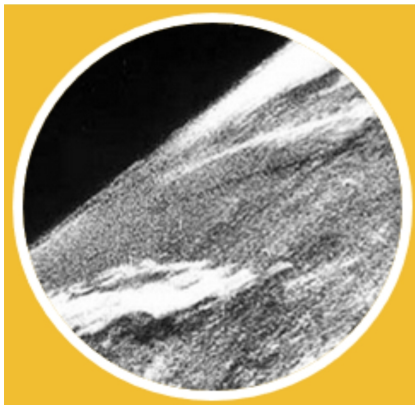
Figure 64: Horizon from V-2 photograph as it appeared on the NASA website
