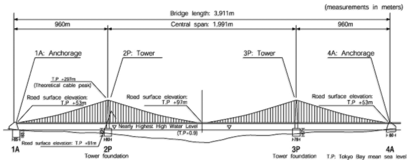
Figure 45: Diagram of the Akashi Kaikyo Bridge showing perfectly parallel suspension towers perpendicular over flat level water.
