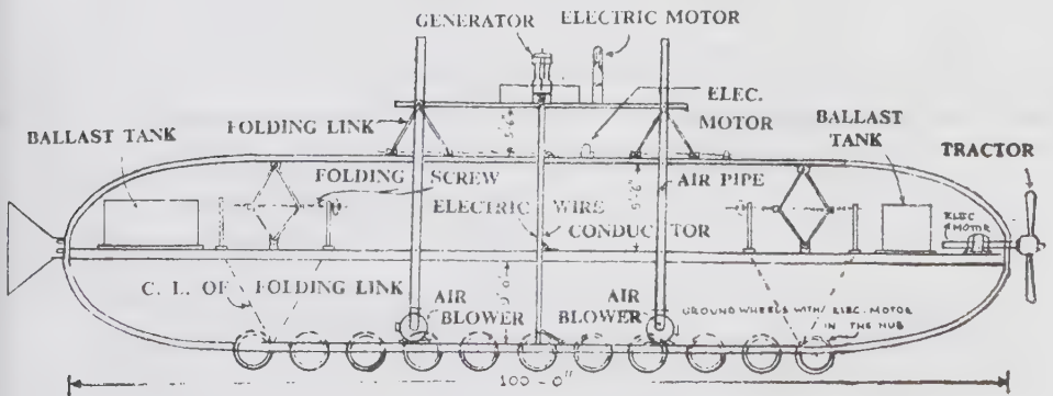
A 1923 drawing by T.K. Ellappa of Bangalore, India of a Vimana (Vimaana) prepared under instruction from Pandit Subbaraya Sastry of Ankal, Bangalore.
