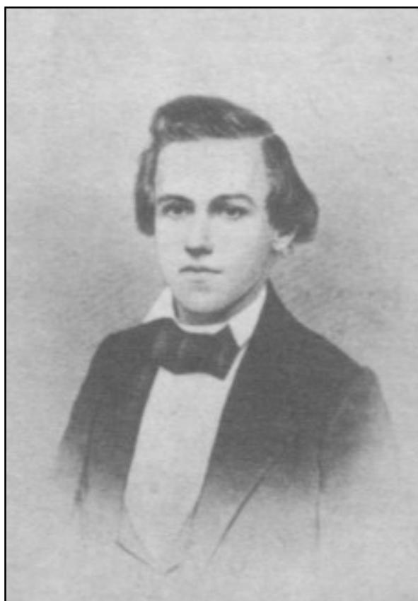
Paul Morphy
