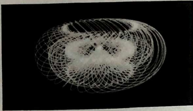
A Torus Construction
