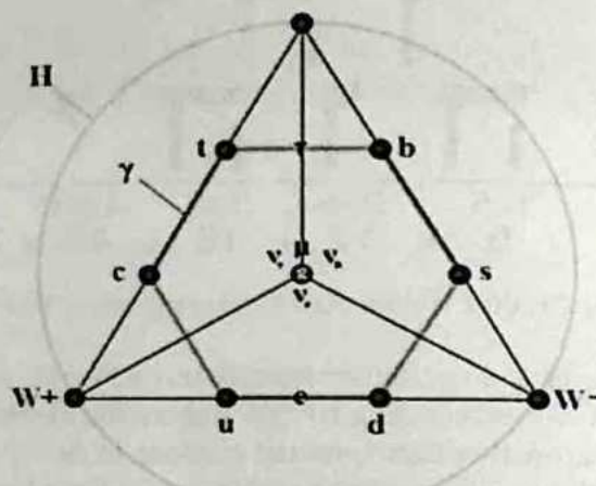
Higgs Boson At Center
