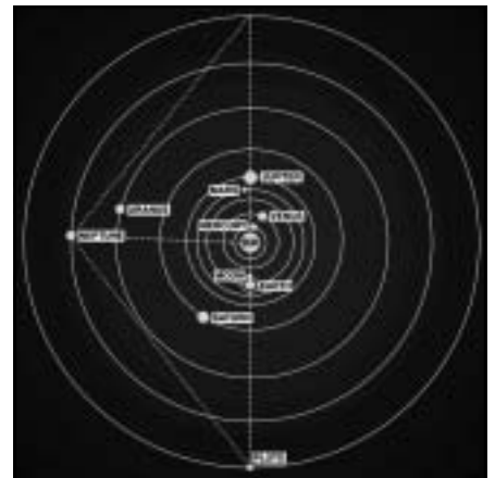
Compressed heliocentric view of the solar system at dawn, Sept. 14, 1814.
