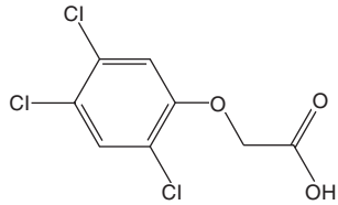
2,4,5-T [93-76-5]
