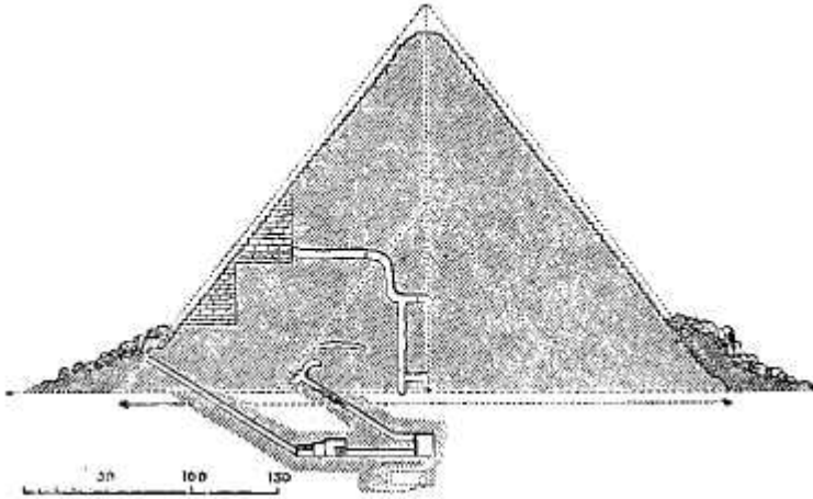
SECTION OF THE THIRD PYRAMID, SHOWING PASSAGES.
