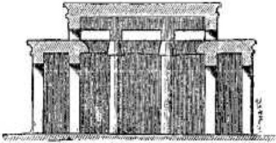
SECTION OF PILLARED HALL OF THOTHMES III. AT KARNAK.
