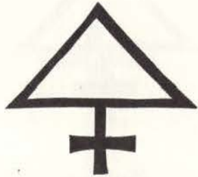
Sulphur
