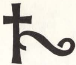
Arsenic
