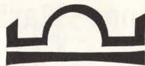
Sublimation
