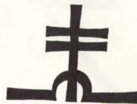
White arsenic
