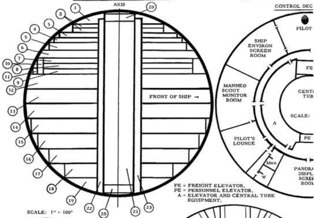
SPC-12 FLOOR LAYOUT (SIDE VIEW)
