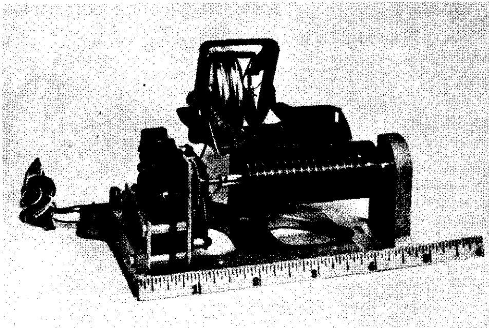
Figure 30. Olland-Cycle pressure modulator.
