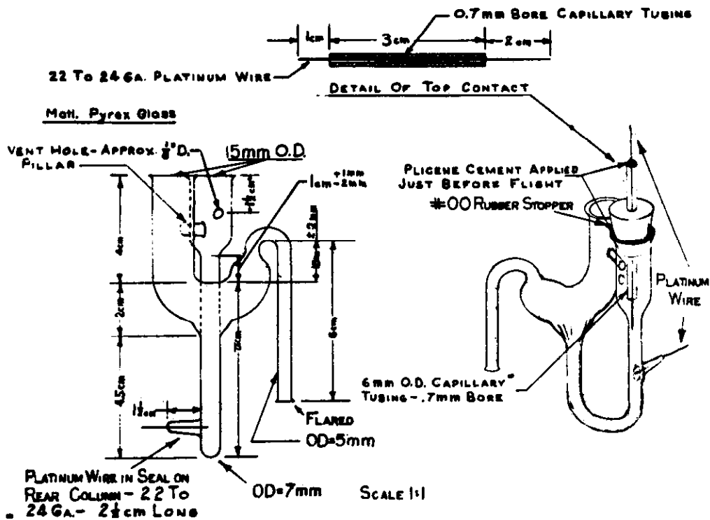
Figure 37. Automatic siphon.
