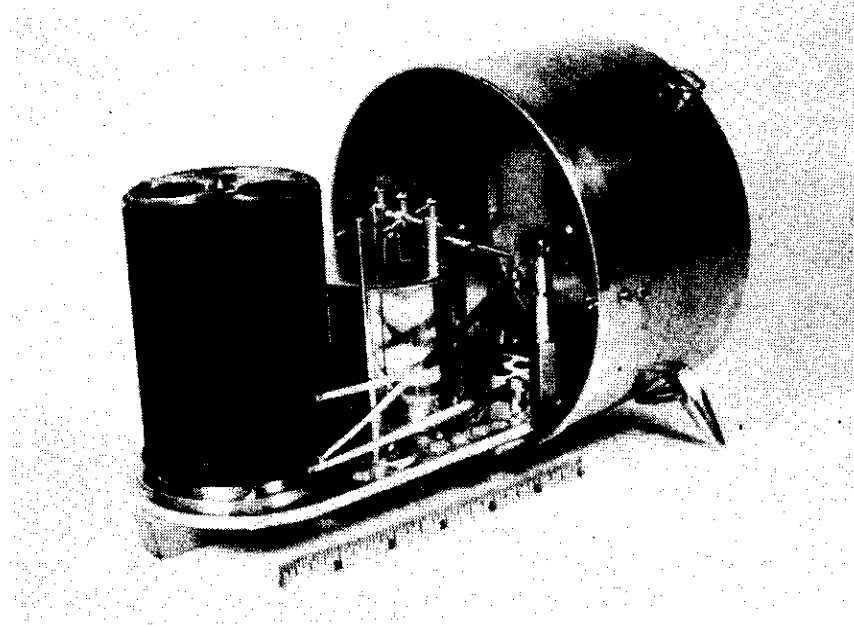
Figure 33. Smoked drum barograph.
