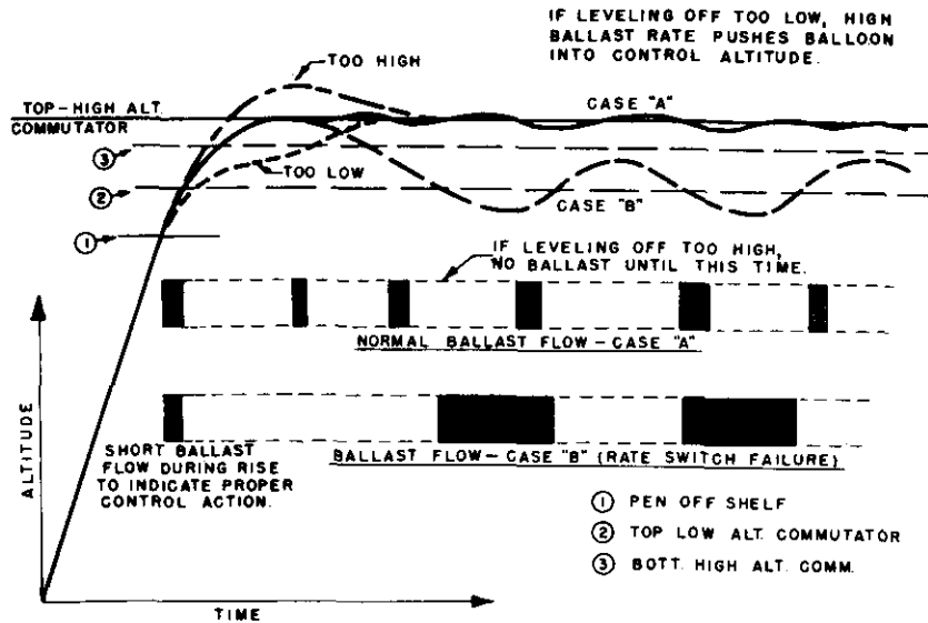
Figure 15. Theoretical height-time curve.
