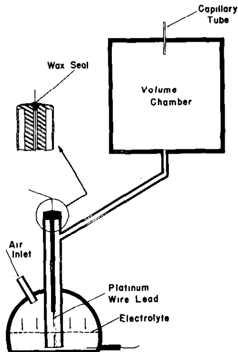
Figure 12. Rate-of-ascent switch.
