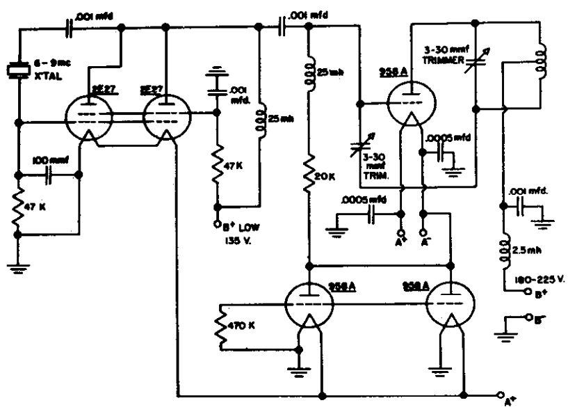
Fig. 7 AM-2 Transmitter
