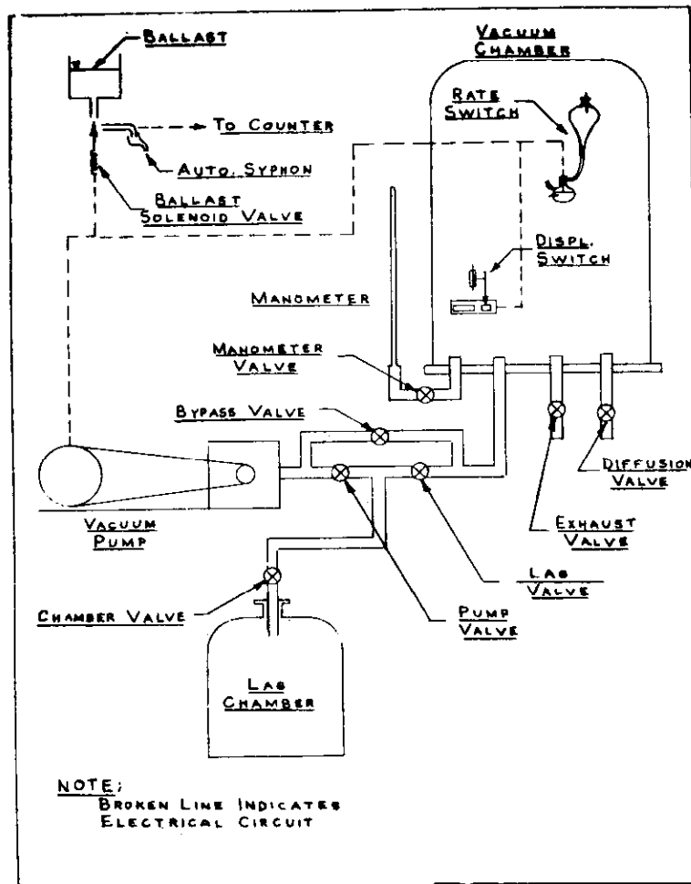
Figure 20. Physical layout, flight-similitude system.
