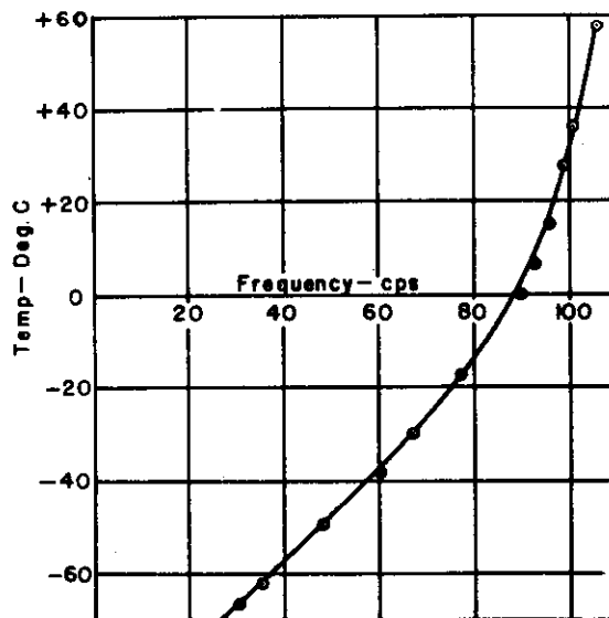
Figure 34. Sample calibration chart for temperature measurements.
