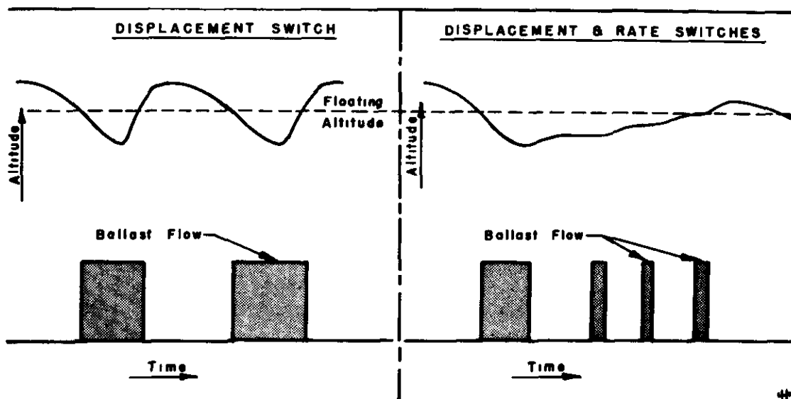
Figure 13. Height-time curve, showing ballast control action.
