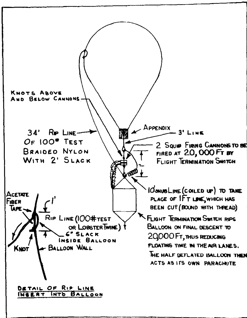
Figure 14: Rip-out line in place on balloon
