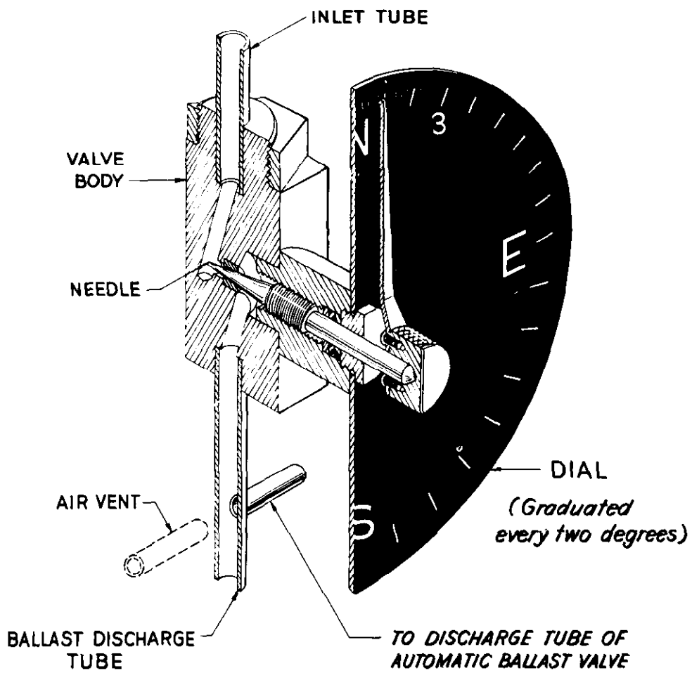
MANUAL BALLAST VALVE
