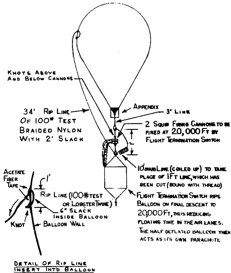
Figure 21. Flight termination equipment.
