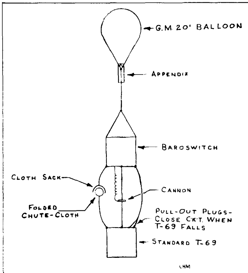
Figure 36: Equipment train, Flight 85
