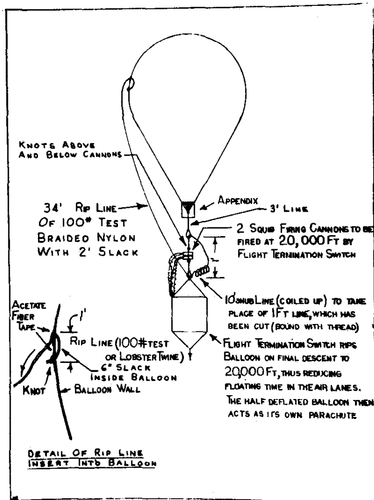
Fig. 13 Balloon Rip Assembly
