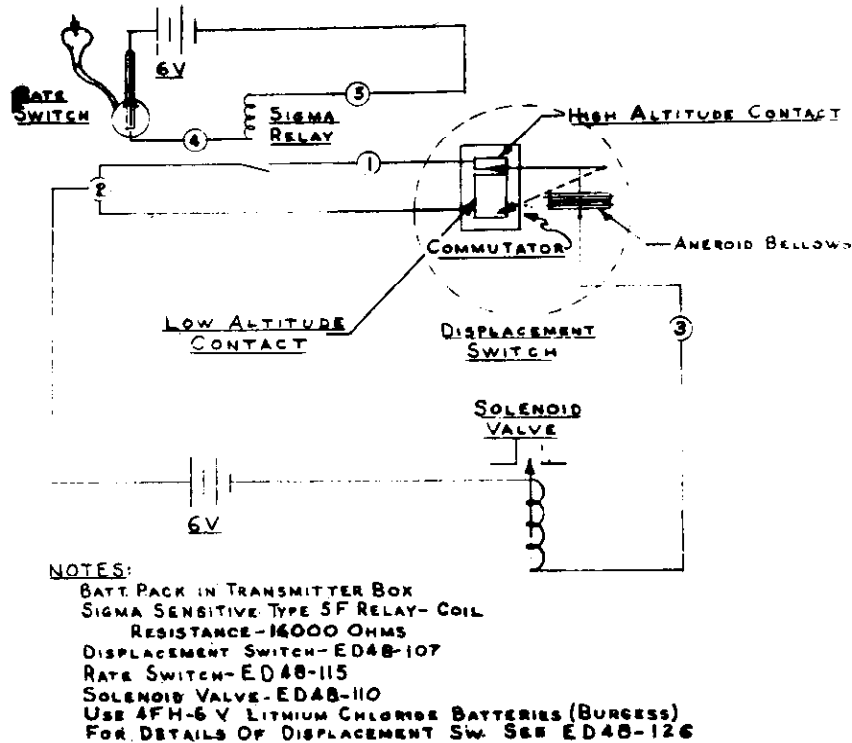
Figure 14. Circuit for ballast control with combined displacement and rate-of-ascent switches.
