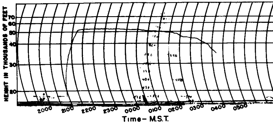
NYU BALLOON PROJECT FLIGHT 71 Barograph Record Of GM 20 Ft. Plastic Balloon Showing Balloon Performance When No Ballast Was Dropped RELEASED AT ALAMOGORDO N.M., 2042 MST-9 JULY, 1948 RECOVERED AT VALENTINE TEXAS, 10 JULY, 1948 ESTIMATED DURATION 10 HOURS
