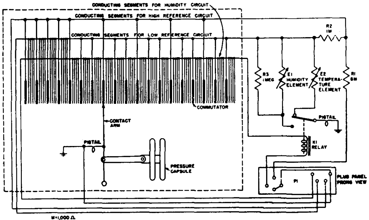
Figure 29. Schematic diagram, Diamond-Hinman radiosonde system.
