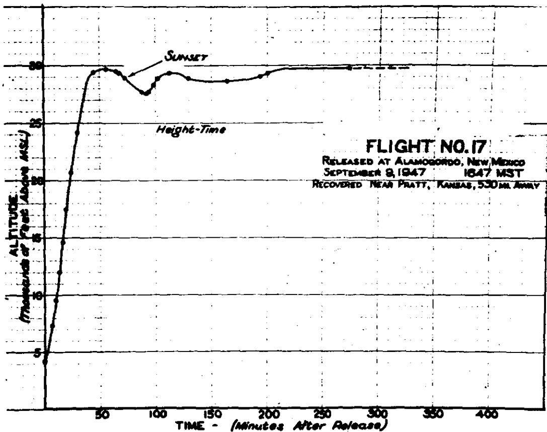
Figure 11: Height-time curve, Flight 17
