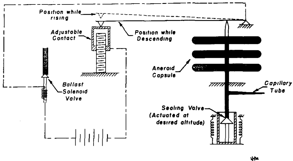
Figure 16. Rate-of-descent switch.
