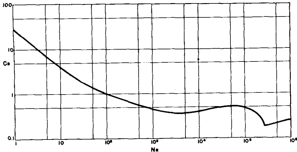
Figure 27. Drag coefficient vs. Reynolds Number, for sphere.
