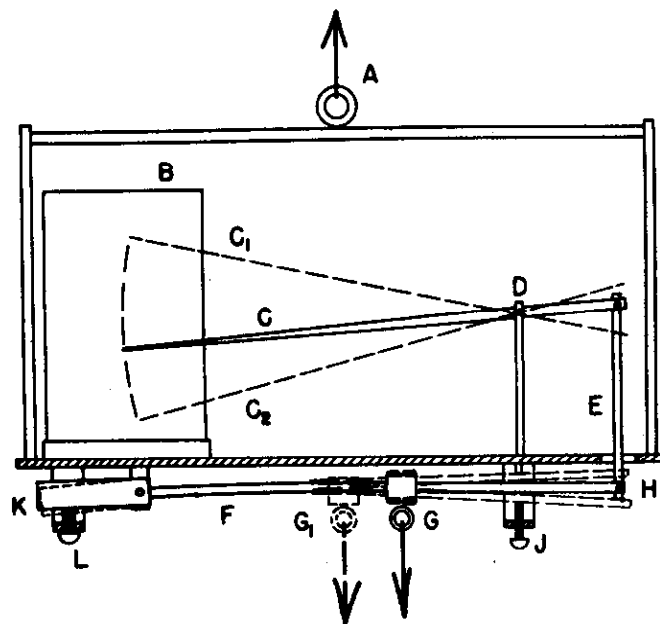
Figure 38. Ballast-recording meter.
