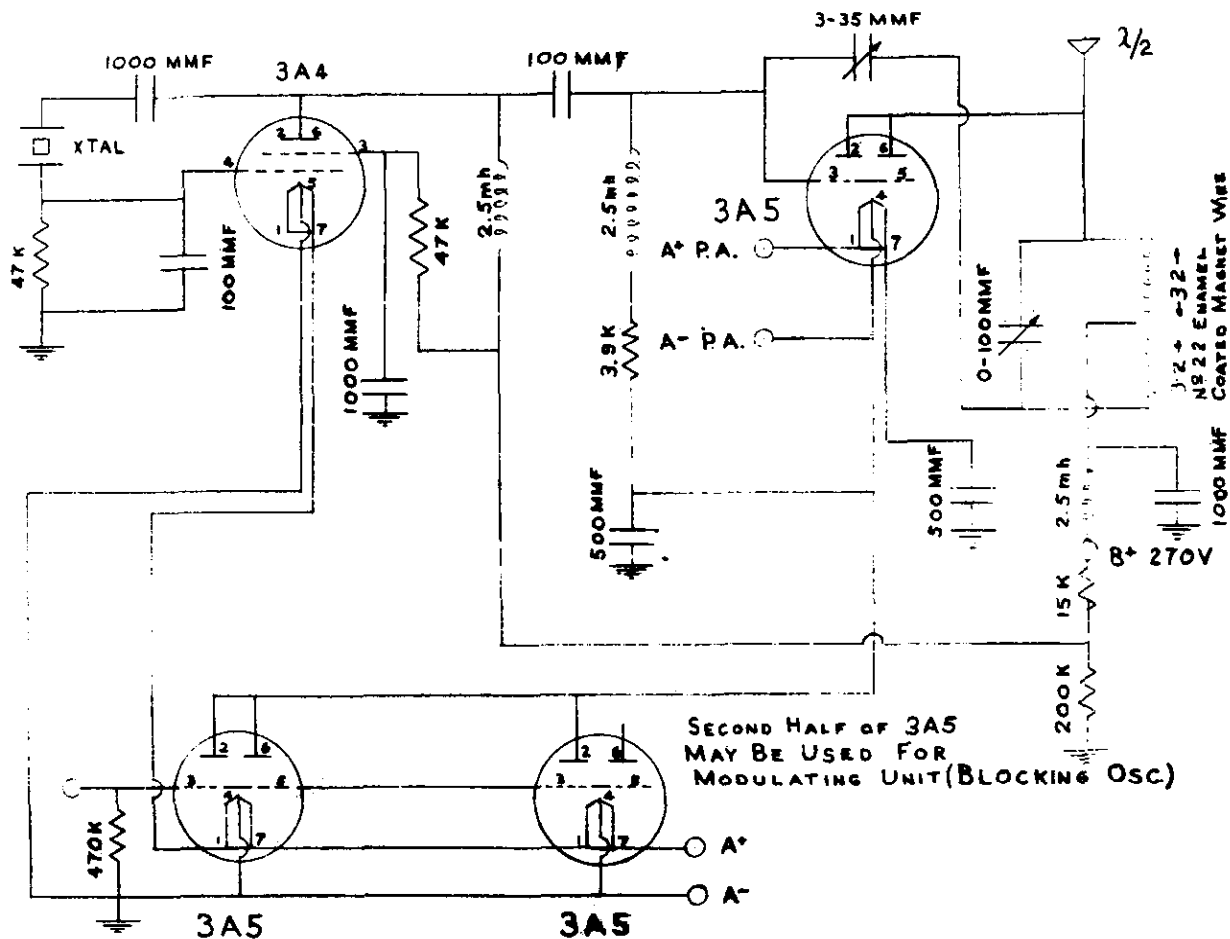
Figure 28. Schematic diagram, AM-1 transmitter.
