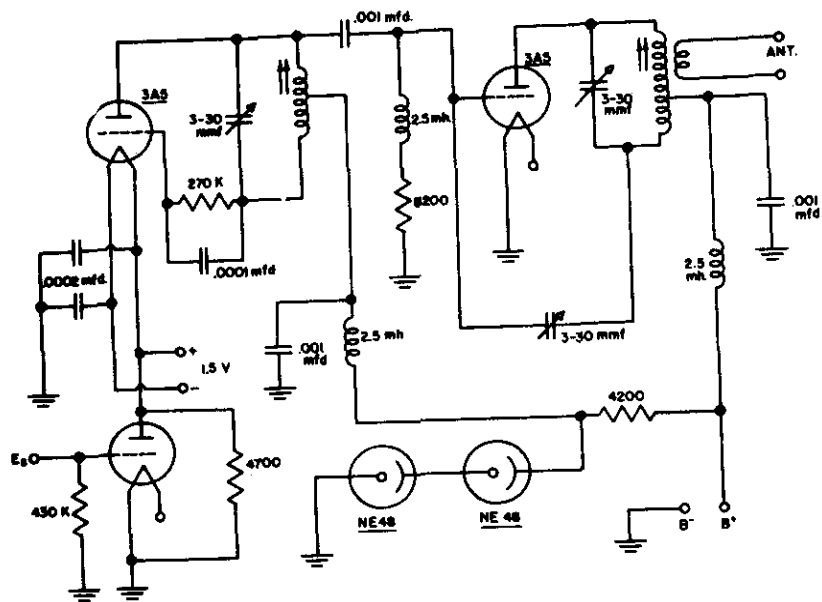
Fig. 5 FM-2 Transmitter
