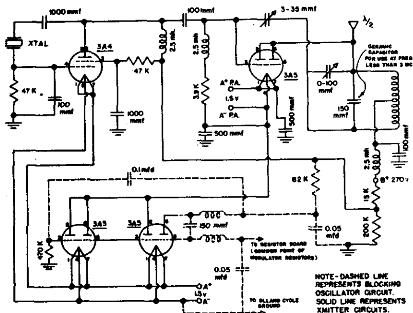
Fig. 6 AM-1 Transmitter
