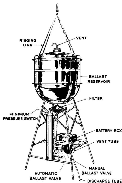
FIG. 3. Ballast-release assembly.
