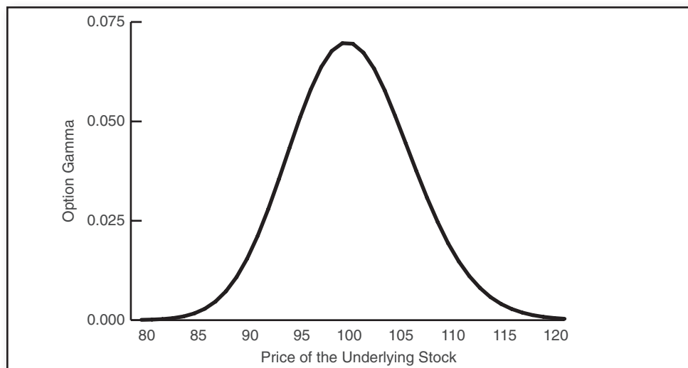
FIGURE 2.7 Gamma
