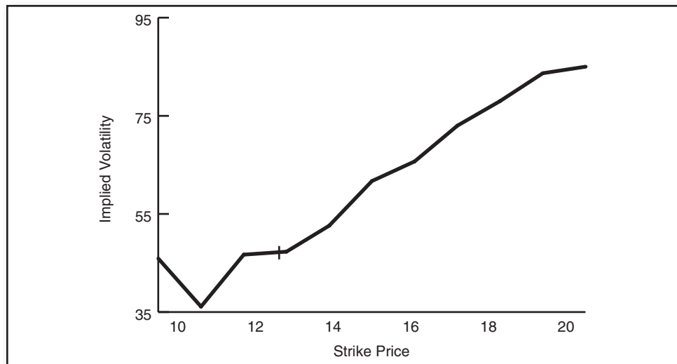
FIGURE 9.10 VIX Skew
