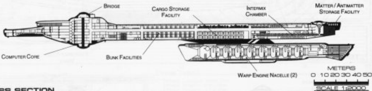
CROSS SECTION
