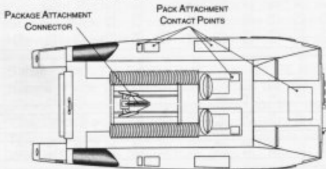
TOP PROFILE
