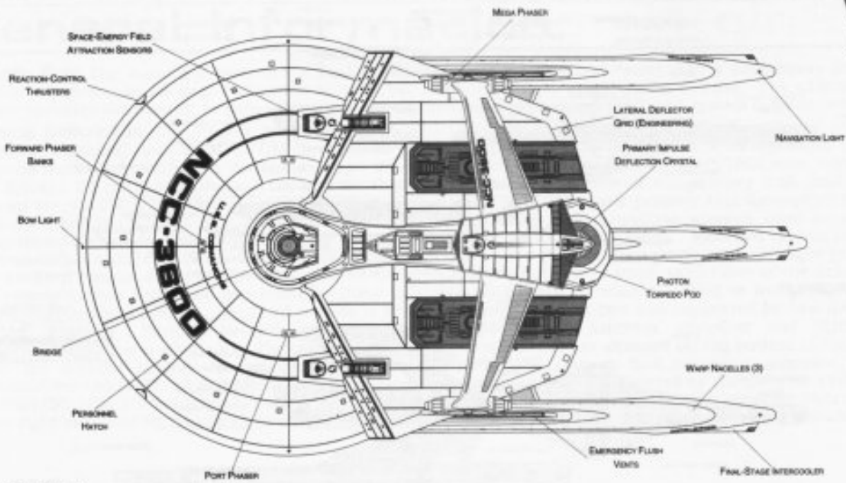
TOP PROFILE
