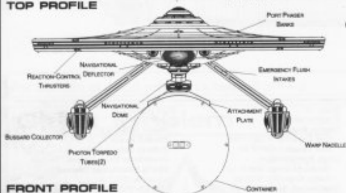
TOP PROFILE
