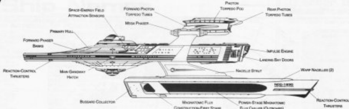
PORT PROFILE
