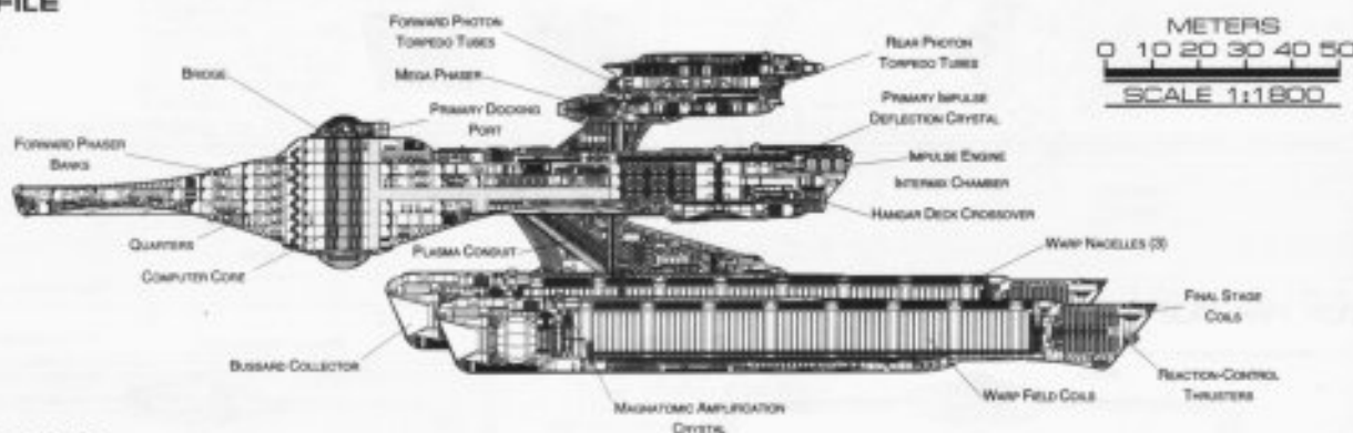
CROSS SECTION
