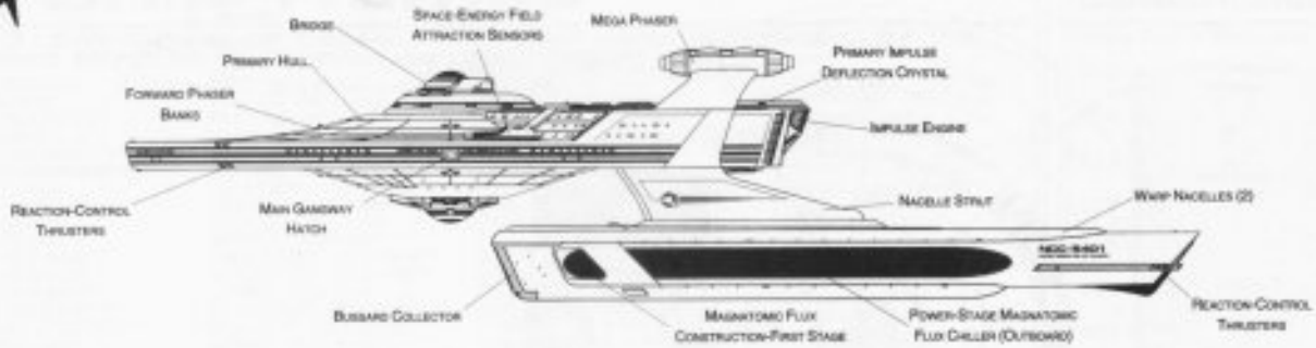
PORT PROFILE
