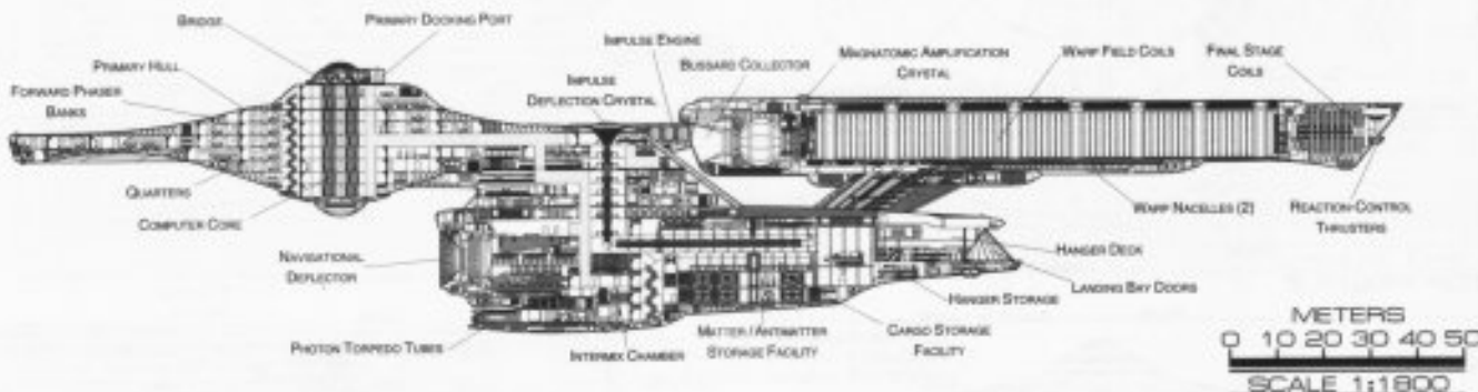
CROSS SECTION
