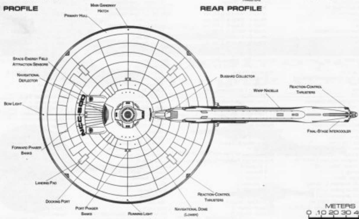
BOTTOM PROFILE
