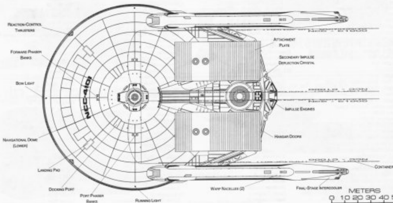
BOTTOM PROFILE
