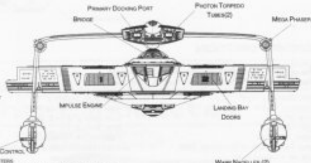
REAR PROFILE
