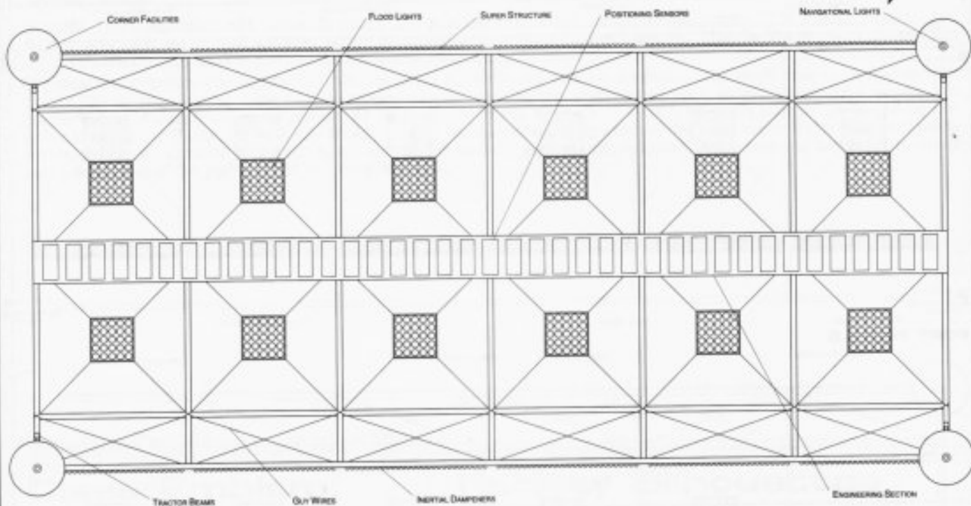
BOTTOM PROFILE
