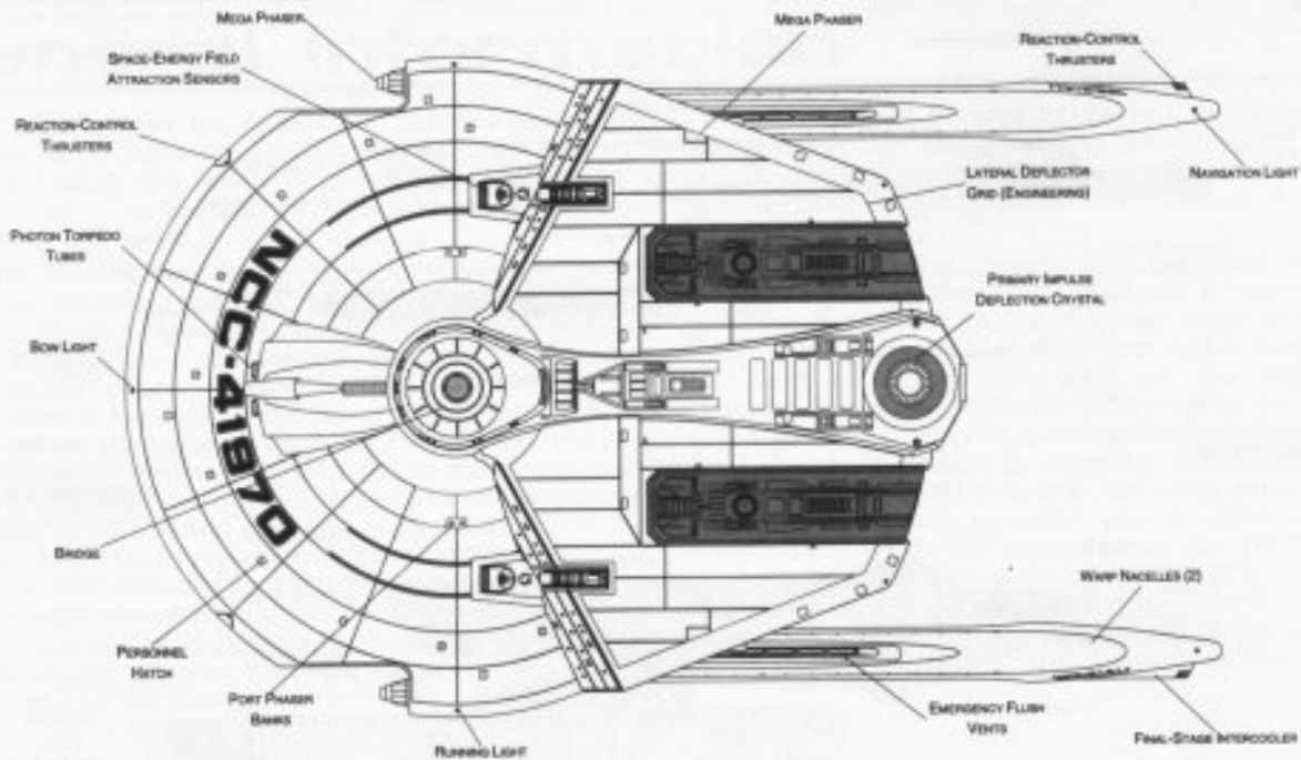
TOP PROFILE
