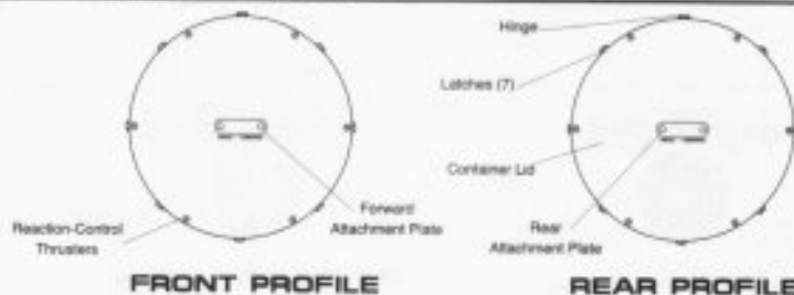
FRONT PROFILE
