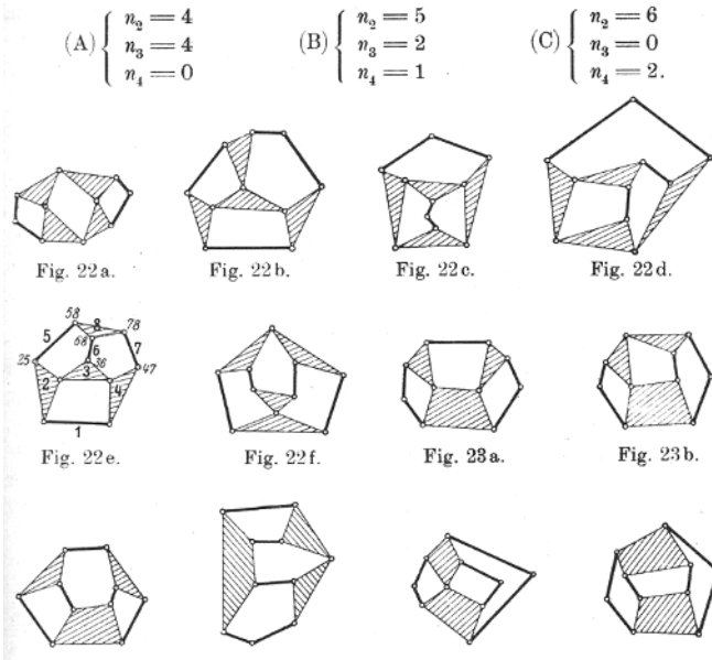
Figure I.32. Table of eight-bar linkages with one degree of freedom when one bar is grounded (Grübler, 1917)
