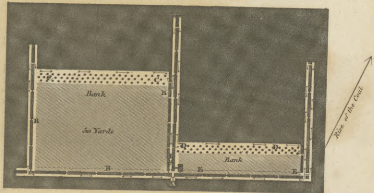
BROAD METHOD OF WORKING COAL.
