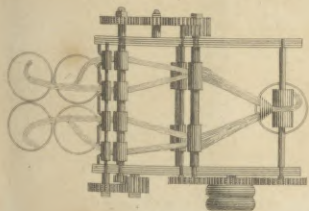
Plan of Drawing frame.
