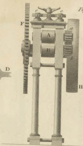
M. Barton's Machine for reducing Plates of Metal to an equal thickness.
