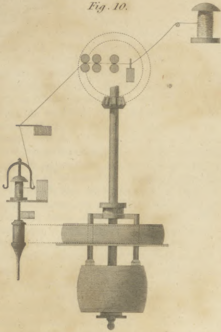
Sir R. Arkwright's, Spinning Frame.
