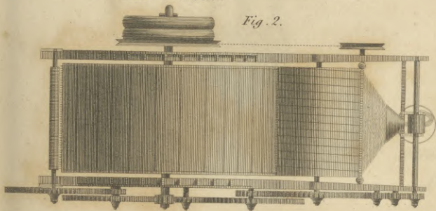
Plan of Cards.
