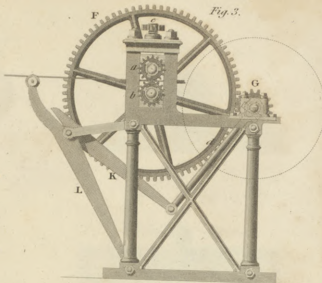
M. Barton's Machine for reducing Plates of Metal to an equal thickness.
