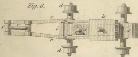
M. Barton's Machine for reducing Plates of Metal to an equal thickness.
