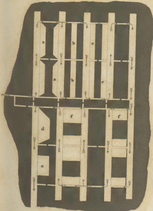
MODE OF REDUCING THE PILLARS, and Retaining the VENTILATION.
