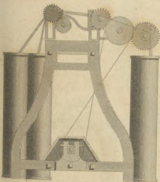
End Elevation of Drawing frame.
