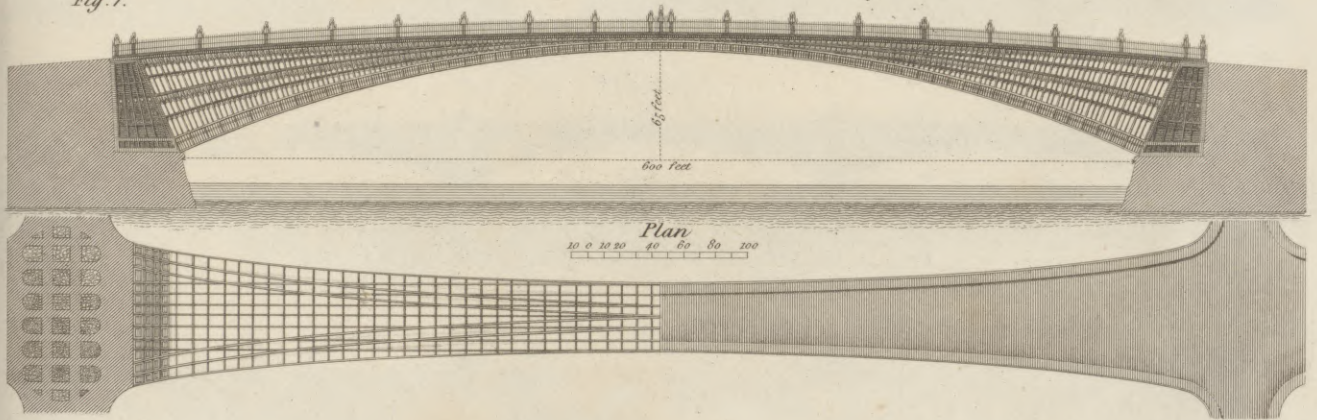
BRIDGE PROPOSED BY MESS: TELFORD AND DOUGLASS.
