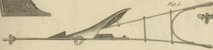
IRON PLOUGH
