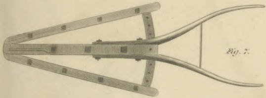
IMPROVED HARROW
