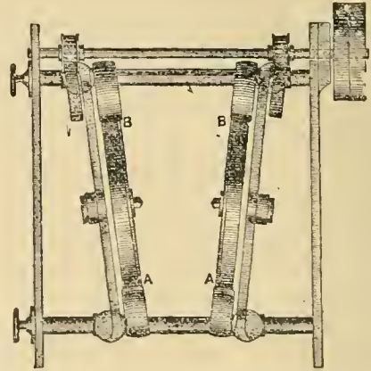
FIG. 13.—Plan of Belt-Stretching Machine.
