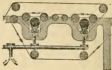
FIG. 5.—Gas Singeing Apparatus.
