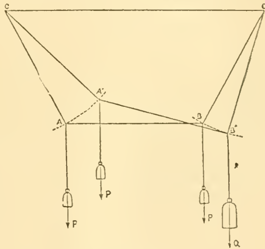
FIG. 1.—Diagram illustrating Chain Balance.
