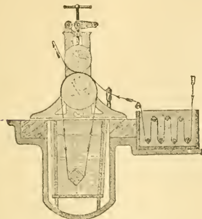
FIG 6 —Section of Lime Squeezer.
