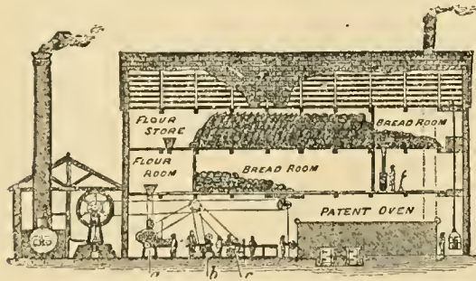
FIG. 1.—Sectional view of Ship-Biscuit Factory.
