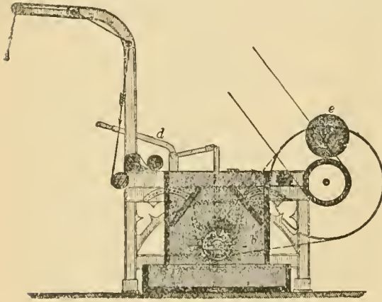
FIG. 11.—Damping-Machine.
