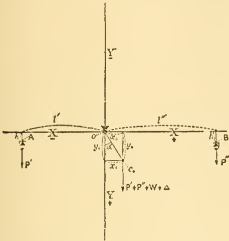
FIG. 7.—Diagram illustrating theory of Precision Balance.
