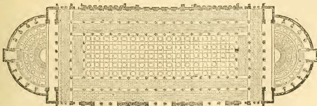
FIG. 3.—Ground-Plan of Trajan's Basilica ( Basilica Ulpia ).
