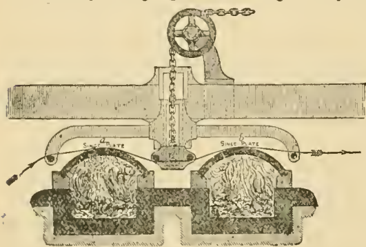
FIG. 4.—Section of Singe Stove.
