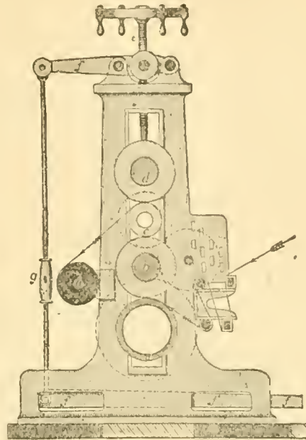
FIG. 17.—Section of Calender.
