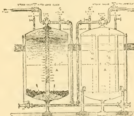
FIG 8 — Barlow's High-Pressure Kiers
