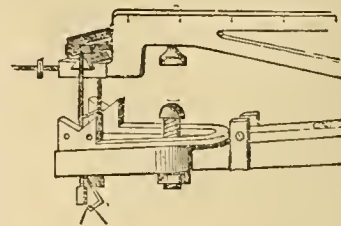
FIG. 4.—Becker's Balance. End of Beam.
