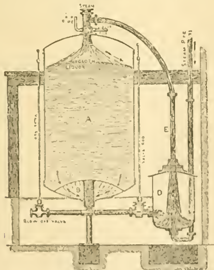
FIG 7 —Taylor's Circulating Kier
