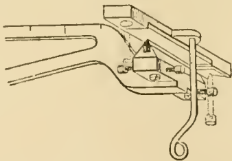
FIG. 3.—Oertling's Balance. End of Beam.
