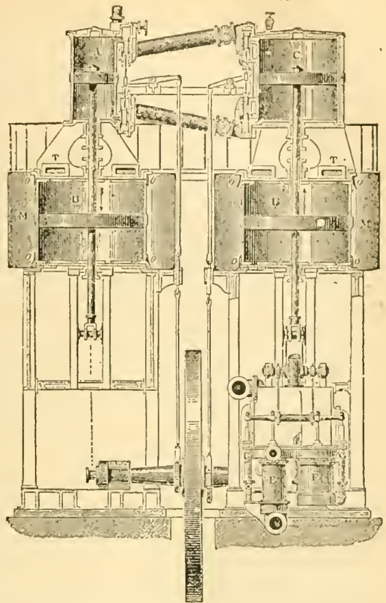
FIG. 4.—Vertical Section of Lackenby Blowing Engines.
