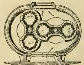
FIG. 6.—Rotary Blower.
