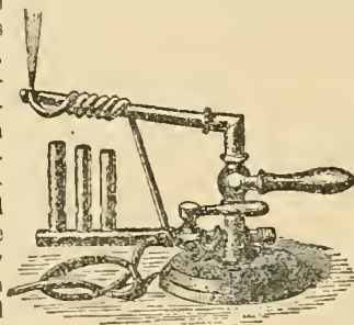
FIG. 6.—Hot-Blast Blowpipe.
