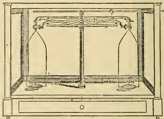
FIG. 5.—Becker's Balance.
