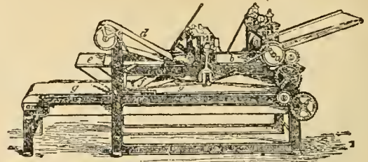
FIG. 2.—Cutting and Panning Machine.
