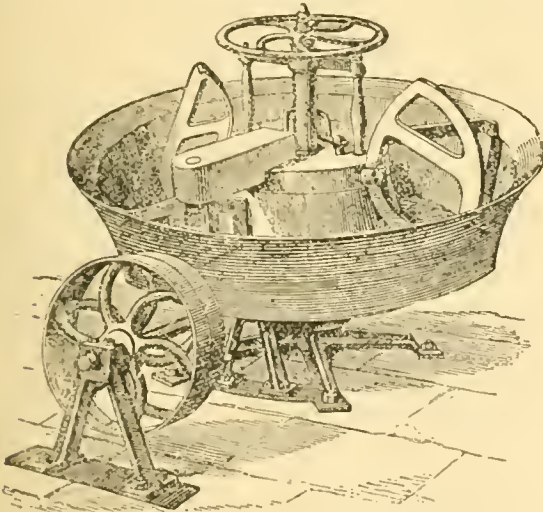
FIG. 6.—Kneading-Machine of Delry Desboves.
