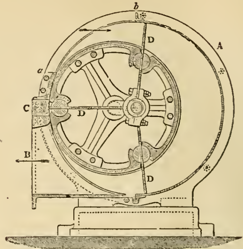
FIG. 5.—Section of an American Blowing-Machine.
