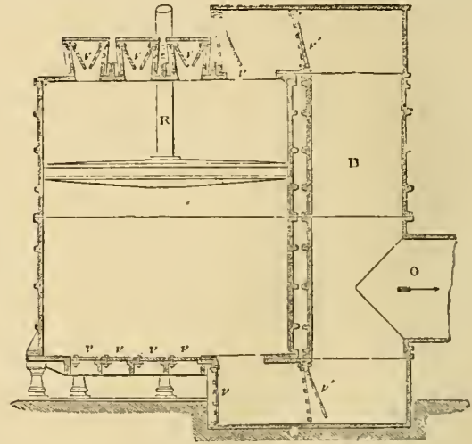
FIG. 3.—Section of Cylinder of Blowing Engine.
