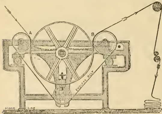
FIG. 12.—Elevation of Belt-Stretching Machine.
