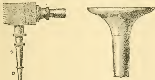
FIG. 1.—Extremities of Gahn's Blowpipe,—ordinary size.
