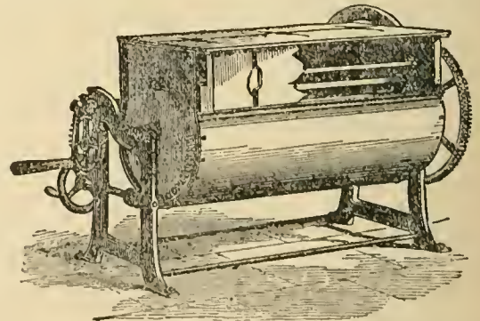
FIG 4.—Kneading Machine.
