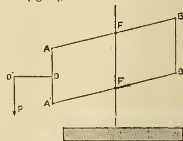
FIG. 8.—Roberval's Balance.
