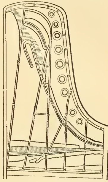
FIG. 33.—Steinway's Grand Piano, 1864. Metal framing in a single casting and overstrung.
