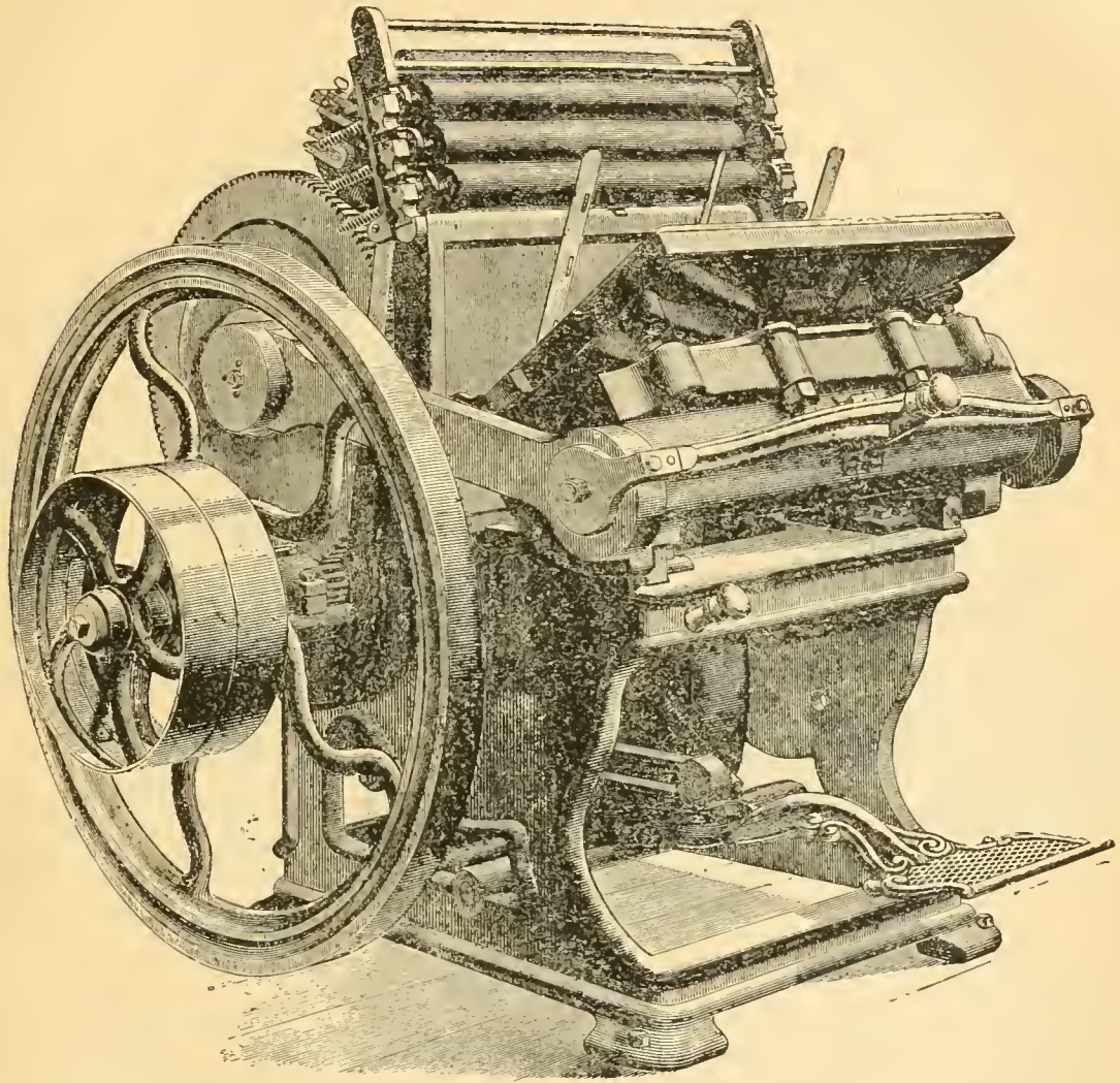
Fig. 3.—THE GALLY UNIVERSAL, THE HIGHEST TYPE OF TREADLE PRESSES.
