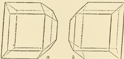
Fig. 10.—Tartaric Acid. a , right-handed; b , left-handed.
