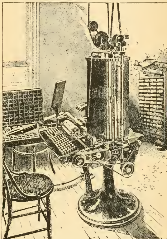
FIG. 9. THORNE TYPE-SETTING AND DISTRIBUTING MACHINE.
