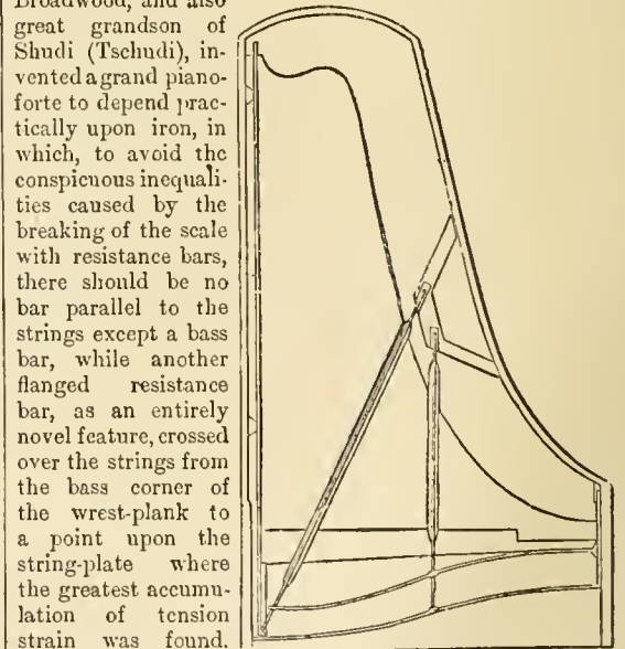
Fig. 31.—Broadwood's Iron Grand Piano, 1834. Complete iron frame with diagonal resistance bar.
