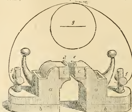
FIG. 4.—Diagram of apparatus of Du Bois-Reymond for experiments on electrical condition of muscle and nerve. a , zinc troughs, mounted on pieces of vulcanite b ; c , paper pads; d , e , small pieces of moist clay; f , f , binding screws for attaching terminals of galvanometer g . A small piece of paper connects d and e , and thus completes the galvanometer circuit. (Wundt.)
