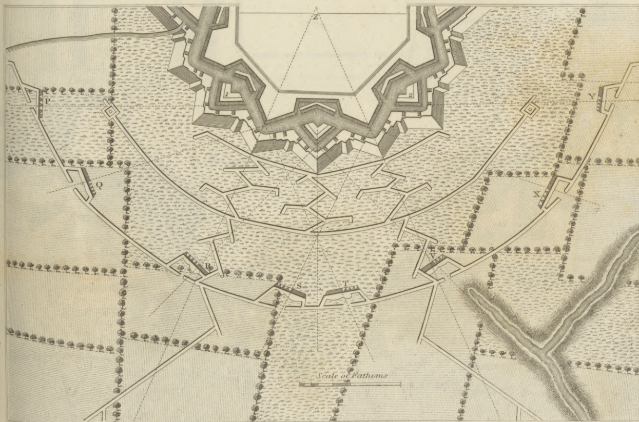
Plan shewing the disposition of the Batteries
