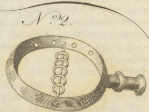
Magic Circle of Circles
