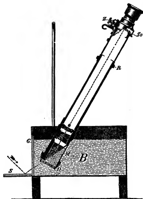
FIG. 6.—Zeiss's Dipping Refractometer.
