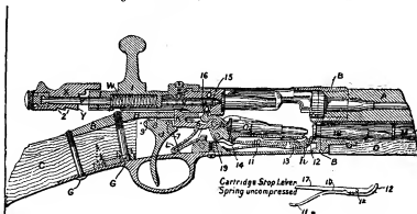
FIG. 16.—Lebel Rifle.
