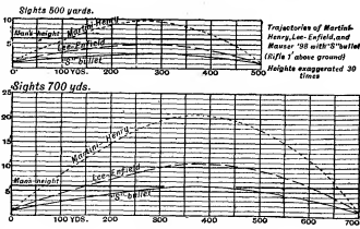
FIG. 20.—Trajectories.
