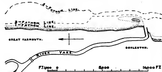
FIG. 10.—Shifting Outlet, fixed by Jetties: River Yare.
