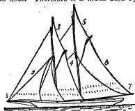
FIG. 5.—Schooner. 1, bowsprit, with martingale to the stem; 2, fore-topmast-stay, jib and stay-foresail; 3, fore-gaff-topsail; 4, foresail and mainstays; 5, main-gaff-topsail; 6, mainsail; 7, end of boom.
