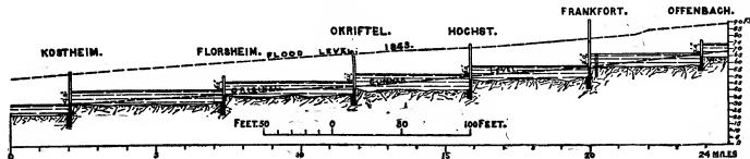
FIG. 7.—Canalized River Main.
