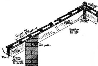
FIG. 22.—Detail of a Slated Roof.
