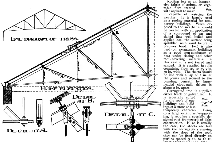
FIG. 9.—Queen-rod Roof Truss.
