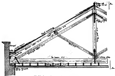
Half elevation; 25° or span.
