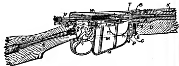
FIGS. 5 and 6.—Lee-Metford.
