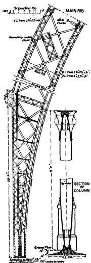
FIG. 11.—Detail of Main Rib and Column, Olympia.
