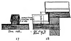
Figs. 17 and 18.—Details of Zinc Flats.
