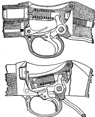
FIG. 2.—Martini-Henry.
