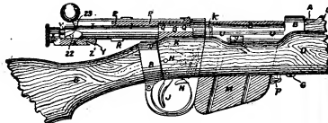
FIGS. 7 and 8.—Lee-Metford.
