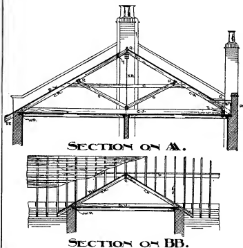
Figs. 6 and 7.—Roof for Domestic Building.
