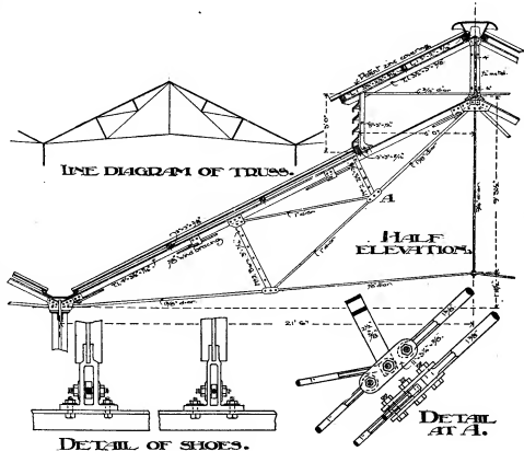
FIG. 10.—Roof at Cardiff Station.
