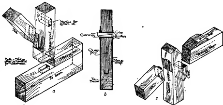
FIG. 4.— a . Detail of queen-post truss at b . b . Vertical section through queen-post. c . Detail of queen-post truss at head; purlin and wrought-iron straps are omitted for the sake of clearness.
