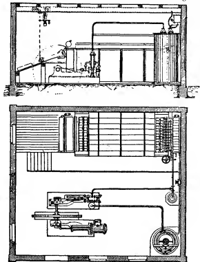
FIG. 6.—General Arrangement of an Ice Factory.
