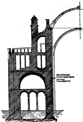
FIG. 13.—Westminster Cathedral: section through nave.
