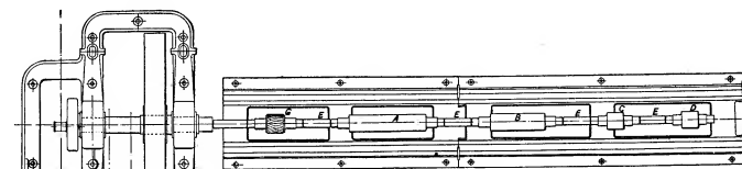
FIG. 3.—12-in. Merchant Guide-Mill and Engine. Four-set mill.
