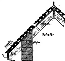
FIG. 23.—Detail of a Tiled Roof.
