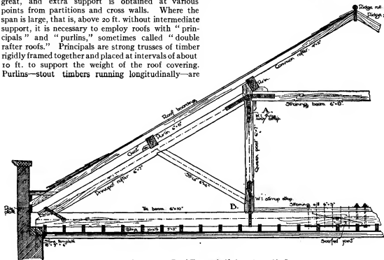
FIG. 3.—Queen-post Roof Truss; half elevation, 38' 0" span.
