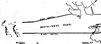
FIG. 15.—Deltaic Jetty Outlet, South Pass, Mississippi.
