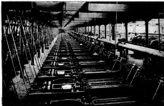
FIG. 15.—BINDER TWINE SPINNING, CONNSWATER MILL.
