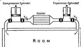
FIG. 1.—Compressed-Air Refrigerating Machine.
