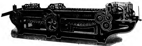
FIG. 11.—GOOD'S HACKLING AND SPREADING MACHINE.
