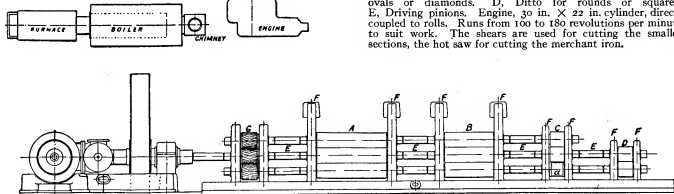
Fig. 2.—General Arrangement of 12-in. Merchant and Guide-Mill Plant. (Thomas Perry & Son Ltd., Bilston.)
