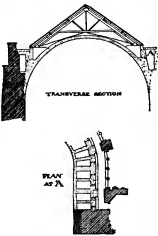
Figs. 15 and 16.—Westminster Cathedral: choir-vaulting.
