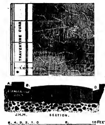
FIG. 5.—Example of Early Basalt Road by the Temple of Saturn on the Clivus Capitolinus. A. Travertine paving. B. Polygonal basalt blocks. C. Concrete bedding. D. Rain-water gutter. The curb shown is taken from another part of the road.
