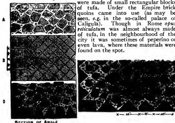
FIG. 3.—Section of Concrete Wall, showing the use of bricks merely as a facing.
