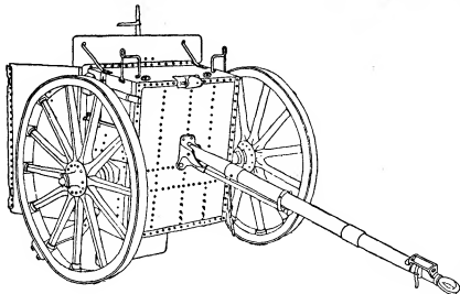
FIG. 66.—Wagon Body, Rumanian (Krupp) Quick-firing Field Gun.
