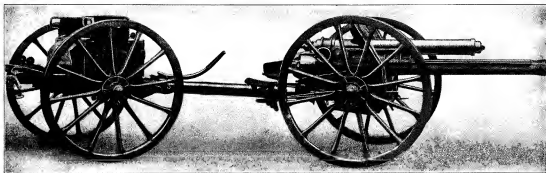
FIG. 61.—BRITISH 18-PR. QUICK-FIRING GUN AND LIMBER.
