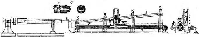
FIG. 21.—Rifling Machine.
