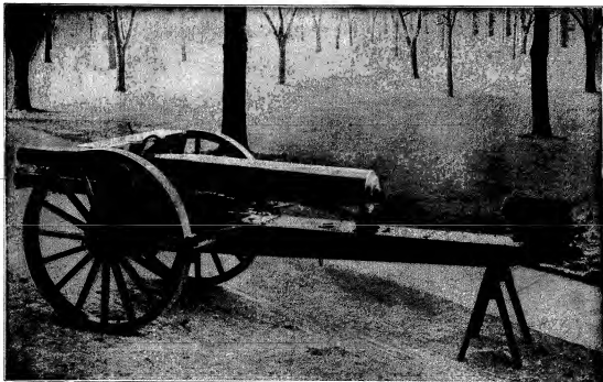
FIG. 69.—4.7-IN. SIEGE GUN, TRAVELLING POSITION (U.S.A.).
