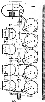
FIG. 5.—Esparto Bleaching and Beating Plant.
