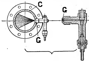
Fig. 15.—Crossley Oil Engine.
