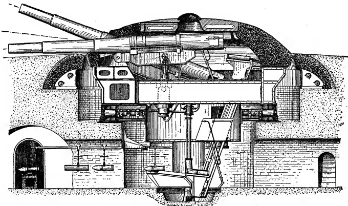
FIG. 82.—Krupp Cupola for two 28-cm. Guns.
