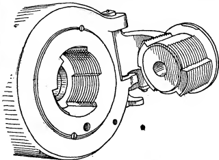
FIG. 38.—Welin Breech Screw.
