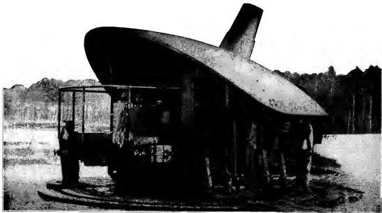
FIG. 83.—KRUPP 11.2-IN. HOWITZER AND SHIELD.
