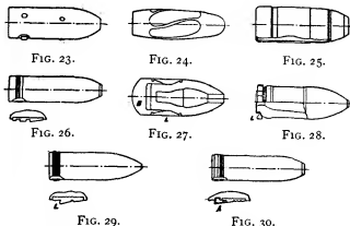
FIGS. 23-30.—Projectiles for Rifled Ordnance.
