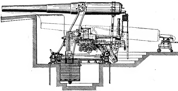
FIG. 81.—Buffington-Crozier Disappearing Carriage for 10" B.L. Gun, U.S.A.
