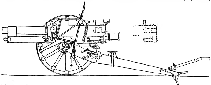
FIG. 63.—The German Q.F. Gun. C. 96. n./A. (1906).
