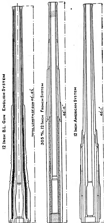
Figs. 55-57.—British, French and American Construction.
