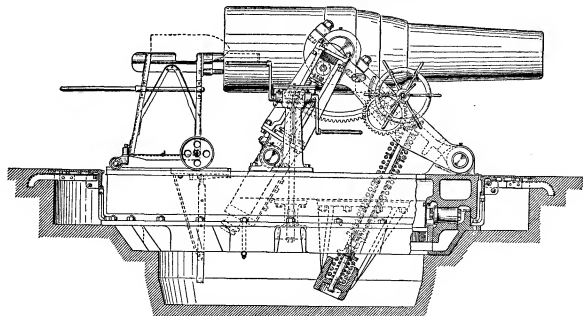
FIG. 89.—12" B.L. Mortar, Model 1896, U.S.A.
