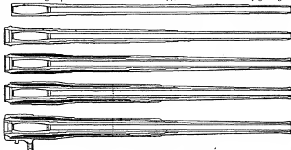
FIG. 14.—Modern B.L. Construction.
