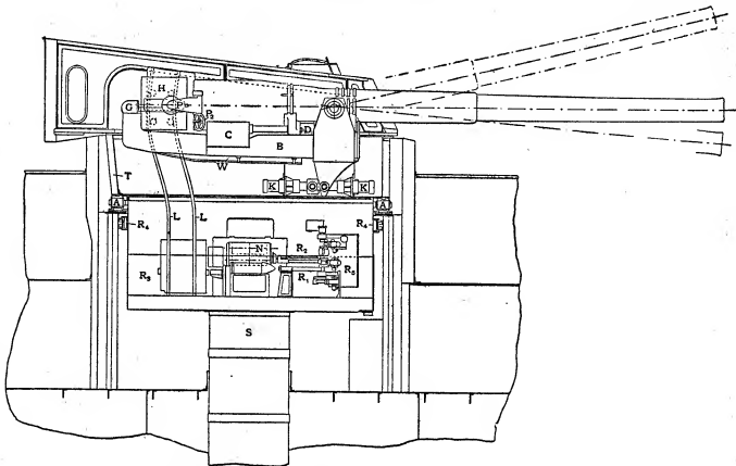
FIG. 91.—Diagram of 12-in. Gun Mounting, "Dreadnought" type.
