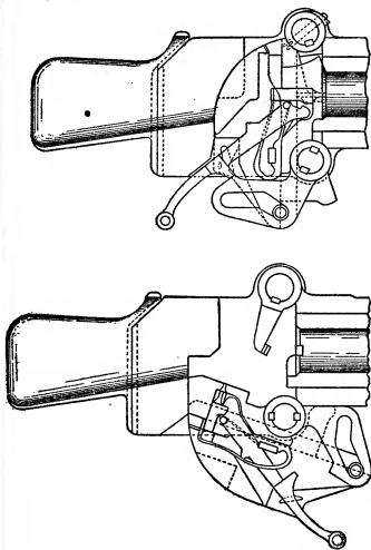
FIG. 35.—Nordenfeldt Q.F. Breech Mechanism.
