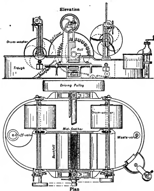
FIG. 2.—Rag-breaking Engine.
