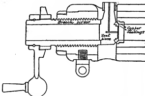
FIG. 10.—Armstrong B.L. Arrangement.
