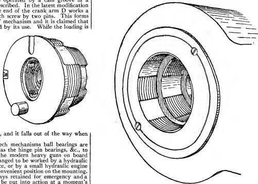
FIG. 39.—Elswick Coned Screw.
