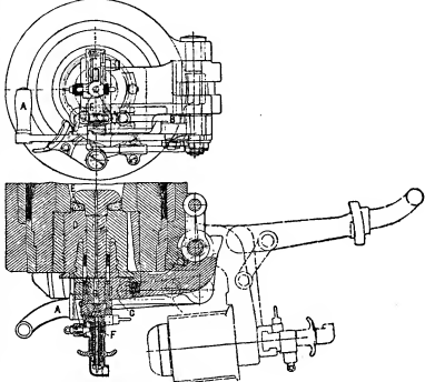
FIG. 43.—Breech Mechanism, Modern 6-in. Gun.
