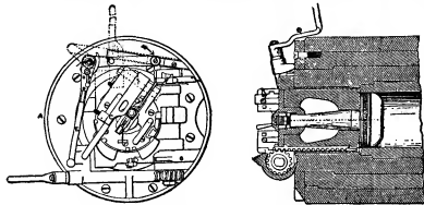
FIG. 40.—Breech Mechanisms, Heavy Guns.
