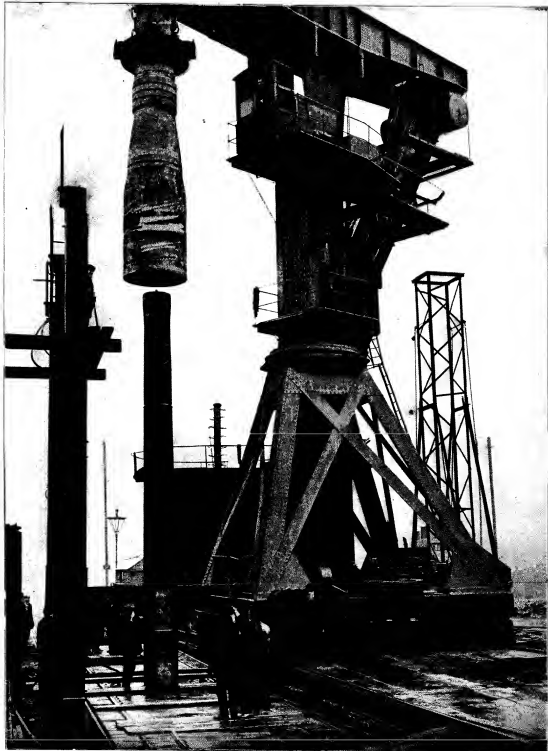
FIG. 18.—SHRINKING-ON PROCESS.
