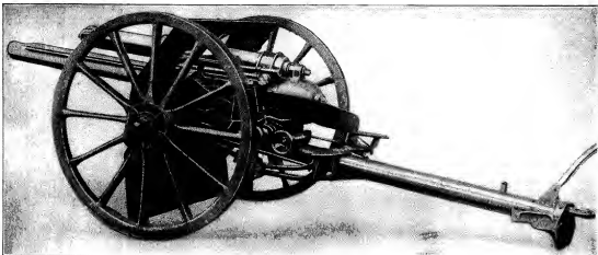
FIG. 60.—BRITISH 18-PR. QUICK-FIRING GUN.
