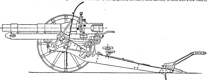
FIG. 65.—Rumanian (Krupp) Quick-Firing Field Gun.
