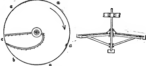
FIG. 10.—Convex Revolving Slime-table.
