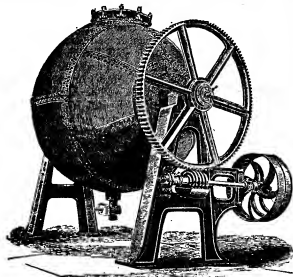
FIG. 1.—Revolving Spherical Rag Boiler.
