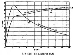
FIG. 31.—Pressure Curves (uniform and increasing twist).
