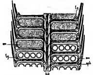
FIG. 10.— Lepidostrobus . Diagram of axis, in longitudinal section. ax , Axis, bearing the sporophylls ( sph ), on each of which a sporangium ( sm ) is seated. lg , Ligule.
