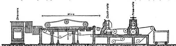
FIG. 4.—"Presse-Pâte," or Half-stuff Machine.
