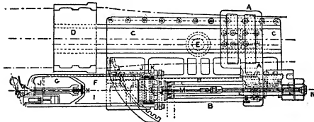
FIG. 85.—Details of Mounting shown in fig. 84.
