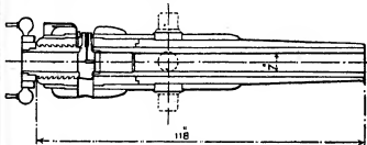
FIG. 11.—Armstrong B.L. Construction.
