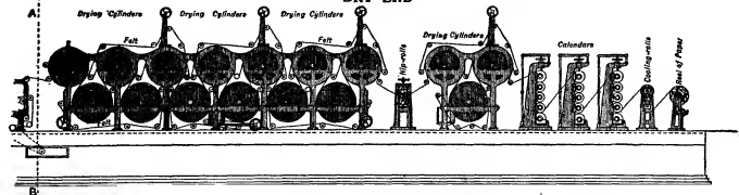
FIG. 12.—Paper-Making Machine.
