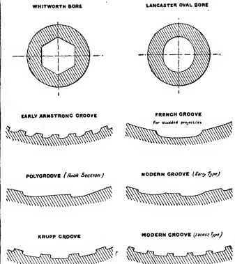
FIG. 22.—Sections of Rifling.
