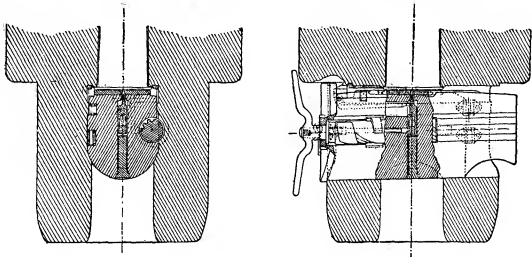
FIG. 33—Krupp Breech Action.
