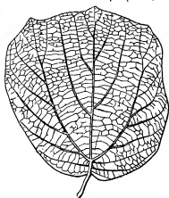
FIG. 3.— Credneria triacuminata .
