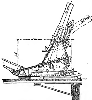
FIG. 73.—Diagram of British 6-in. B.L. Howitzer (79° elevation).
