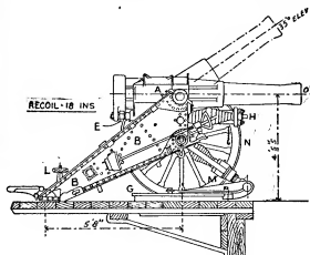
FIG. 72.—Diagram of British 6-in. B.L. Howitzer.
