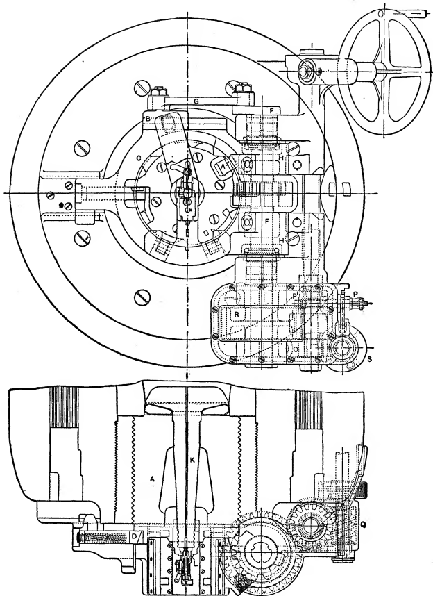
FIG. 41.—12-in. Gun, Breech Mechanism.
