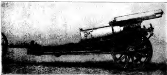
FIG. 76.—KRUPP 8.26-IN. MORTAR, TRAVELLING.
