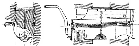
FIG. 32—Krupp Breech Action.
