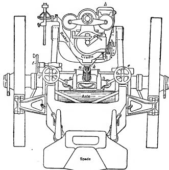
FIG. 75.—Diagram of 6-in. Siege Howitzer, U.S.A.
