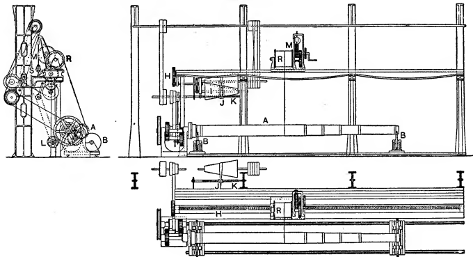
FIG. 20.—Wire-winding Machine.
