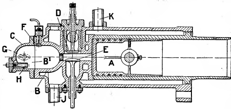
FIG. 14.—Crossley Oil Engine.
