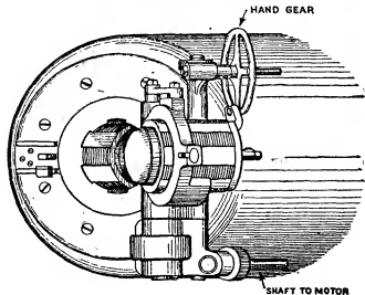
FIG. 37.—Interrupted Breech Screw—Cylindrical.
