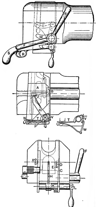
FIG. 34.—Hotchkiss Q.F. Breech Mechanism.
