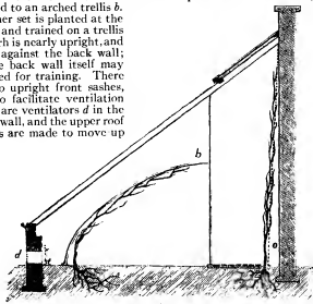
FIG. 8.—Peach House.
