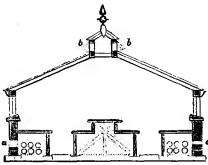
FIG. 4.—Section of Plant Stove.
