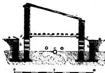
FIG. 10.—Ventilated Plant Pit.
