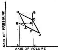
FIG. 5.—Elementary Carnot Cycle for Gas.
