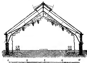
FIG. 7.—Span-roofed Vinery.
