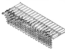
FIG. 9.—Individual Action of the Latch Needle.
