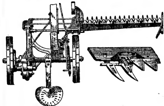
FIG. 1.—Mower (viewed from above) with enlarged detail of Blade. (Harrison, McGregor & Co.)
