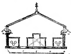
FIG. 3.—Section of Greenhouse.
