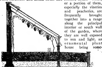
FIG. 5.—Lean-to Vinery.
