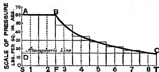
FIG. 3.—Watt's Indicator Diagram. Patent of 1782.
