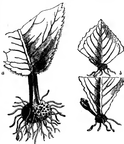
FIG. 23.—Leaf Cuttings.
