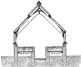
FIG. 9.—Forcing House.
