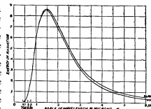
FIG. 8.—Distribution of energy in the spectrum of full radiation at 2000^\circ Abs. according to formulæ of Planck & Wien.
