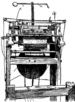
FIG. 3.—Hand Stocking Frame.
