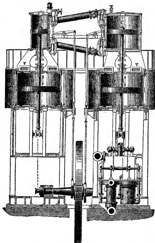
FIG. 4.—Vertical Section of Lackenby Blowing Engines (1871).
