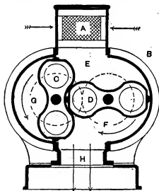
FIG. 6.—Thwaites' Improved Roots' Blower.
