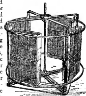
FIG. 21.—Cowan's four-frame Extractor; interior.
