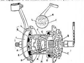
FIG. 12.—Eadie Two-speed Coaster Hub.
