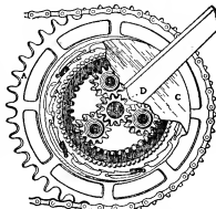
FIG. 13.—Sunbeam Two-Speed Gear.
