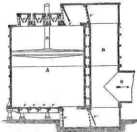
Fig. 3.—Section of Cylinder of Early Blowing Engine (1851).
