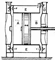
FIG. 5.—Richardson, Westgarth & Co.'s Blowing Engine.
