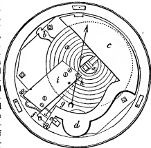
FIG. 4.—Aneroid Barometer.
