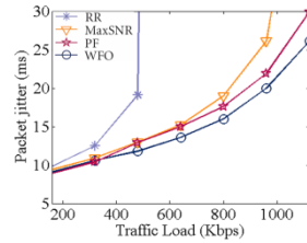
Fig. 9 c. Packet jitter.
