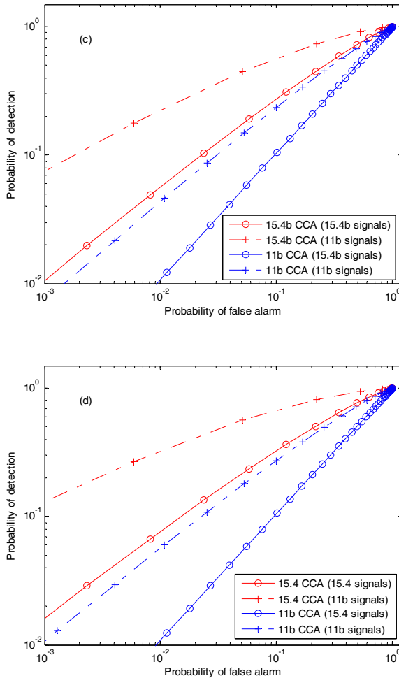
Fig. 4. ROC of energy based CCA in the case of SNR=-9.5 dB measured by WPAN over a) AWGN channel; b) log-normal shadowing ( \sigma_{dB}= 6\text{dB} ) channel; (c) Rayleigh fading channel, and d) Rician fading ( K=1.5 ) channel.
