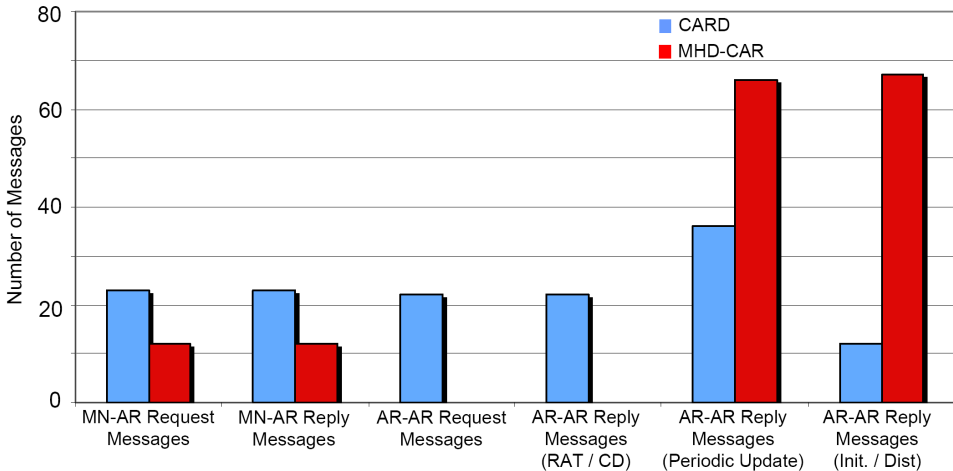
Fig. 10. Signalling Load Comparison of CARD and MHD-CAR
