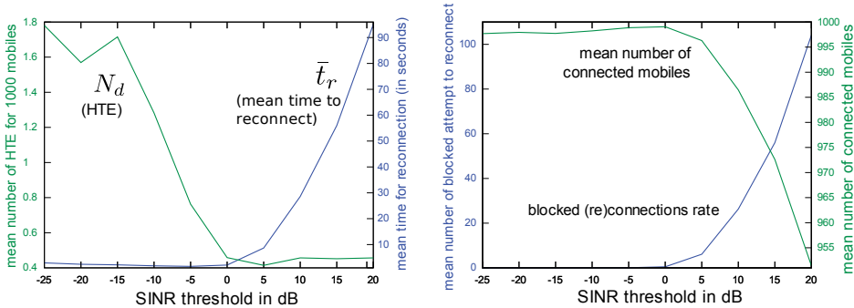
(a) Comparing the number of lost connections and the mean time before reconnection (b) Comparing the mean number of connected mobiles and the block rate
