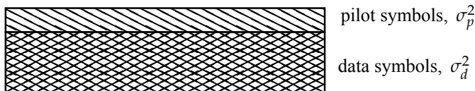
Fig. 4. Overlay pilot scheme
