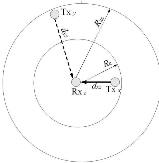
Fig. 1. Model to drive the pdf of the SIR from a single neighboring cell
