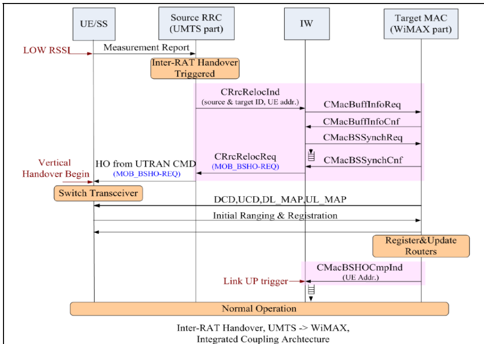
Fig. 4. Handover signaling procedure from UMTS to WiMAX
