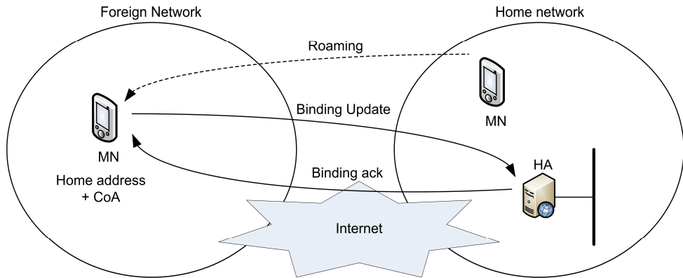
Fig. 3. MIPv6 Operation
