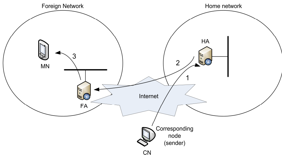
Fig. 2. MIPv4 Operation
