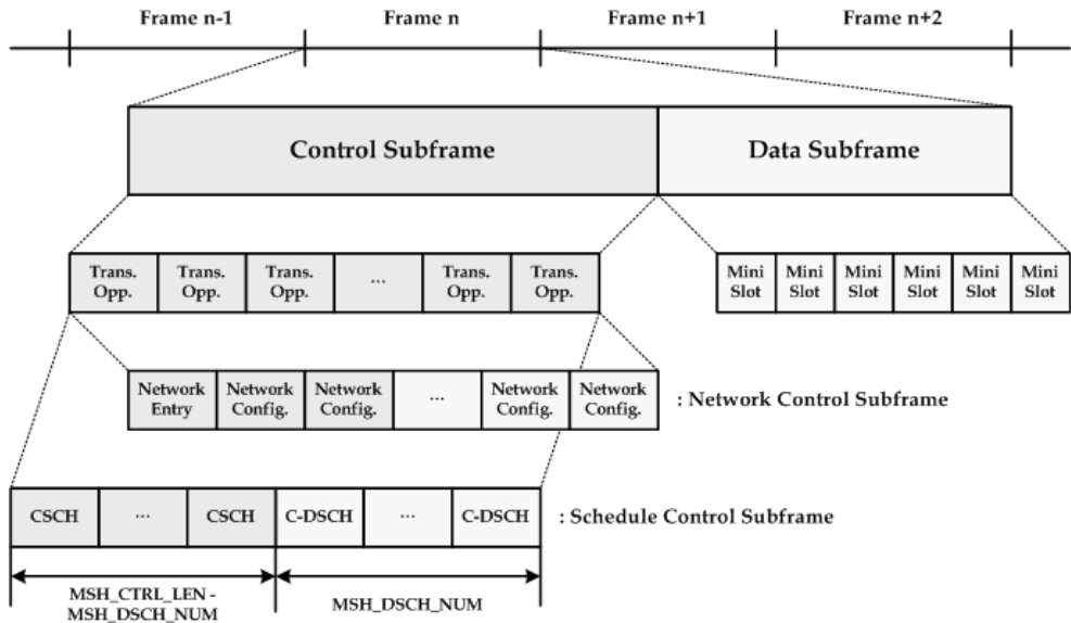
Fig. 1. Frame structure of IEEE 802.16 mesh mode
