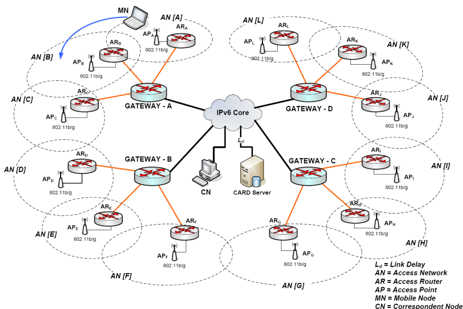
Fig. 7. Simulation Topology
