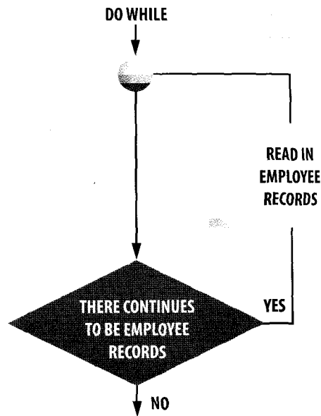
Fig 2 While loop
